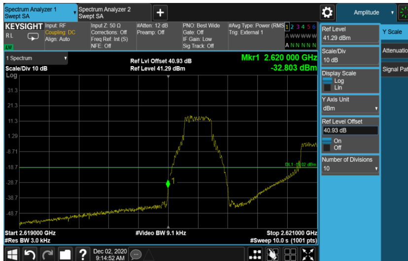
Port D, Channel Position B, WCDMA 5.0MHz, LTE 10.0MHz, NB 250KHz
