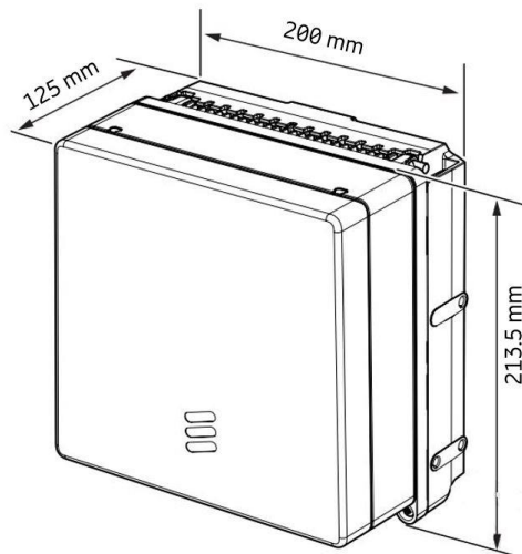
Figure D.1 Picture of Single Radio version of Radio 4402 B2/B25.
