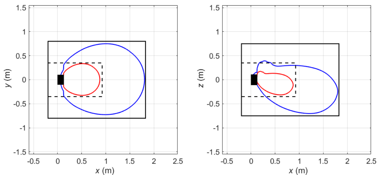
Figure 2 Compliance boundary for general public (black solid line) and workers (black dashed line) exposure for Single Radio. The blue solid lines correspond to compliance distance results for general public exposure obtained using the spherical model. The solid red lines indicate the corresponding compliance distance results for workers exposure. The EUT is shown from above (left) and from the side (right) with its back plane located at x = 0 m. Mode: B2/B25 (1900) (L/N ). Total power delivered to the antenna: 23.0 W.
