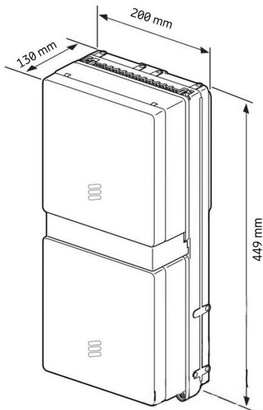
Figure D.2 Picture of Dual Radio version of Radio 4402 B2/B25.
