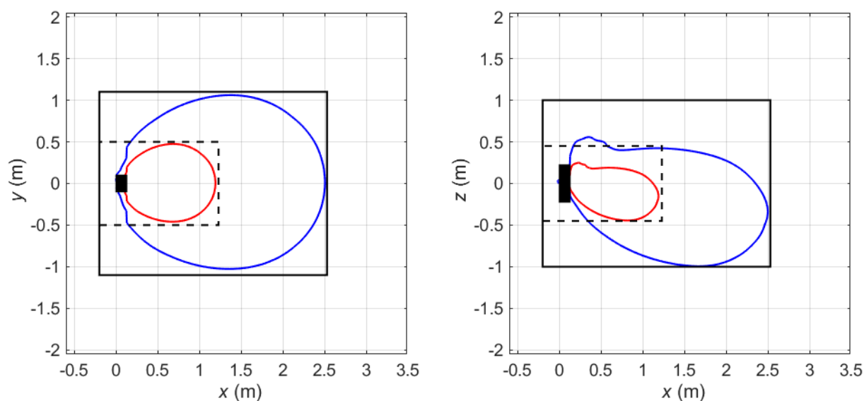
Figure 3 Compliance boundary for general public (black solid line) and workers (black dashed line) exposure for Dual Radio. The blue solid lines correspond to compliance distance results for general public exposure obtained using the spherical model. The solid red lines indicate the corresponding compliance distance results for workers exposure. The EUT is shown from above (left) and from the side (right) with its back plane located at x = 0 m. Mode: B2/B25 (1900) (L/N ). Total power delivered to the antenna: 45.9 W.
