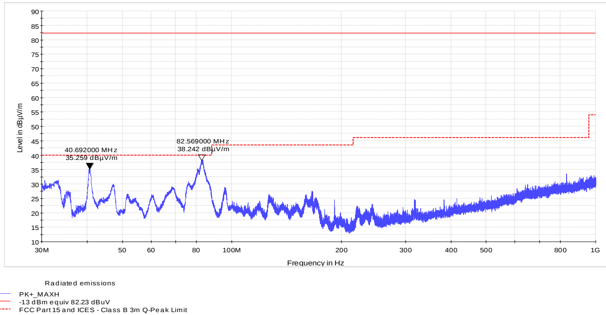
Figure 8.3-15: Radiated emissions spectral plot, WCDMA, high channel (30 to 1000 MHz)
