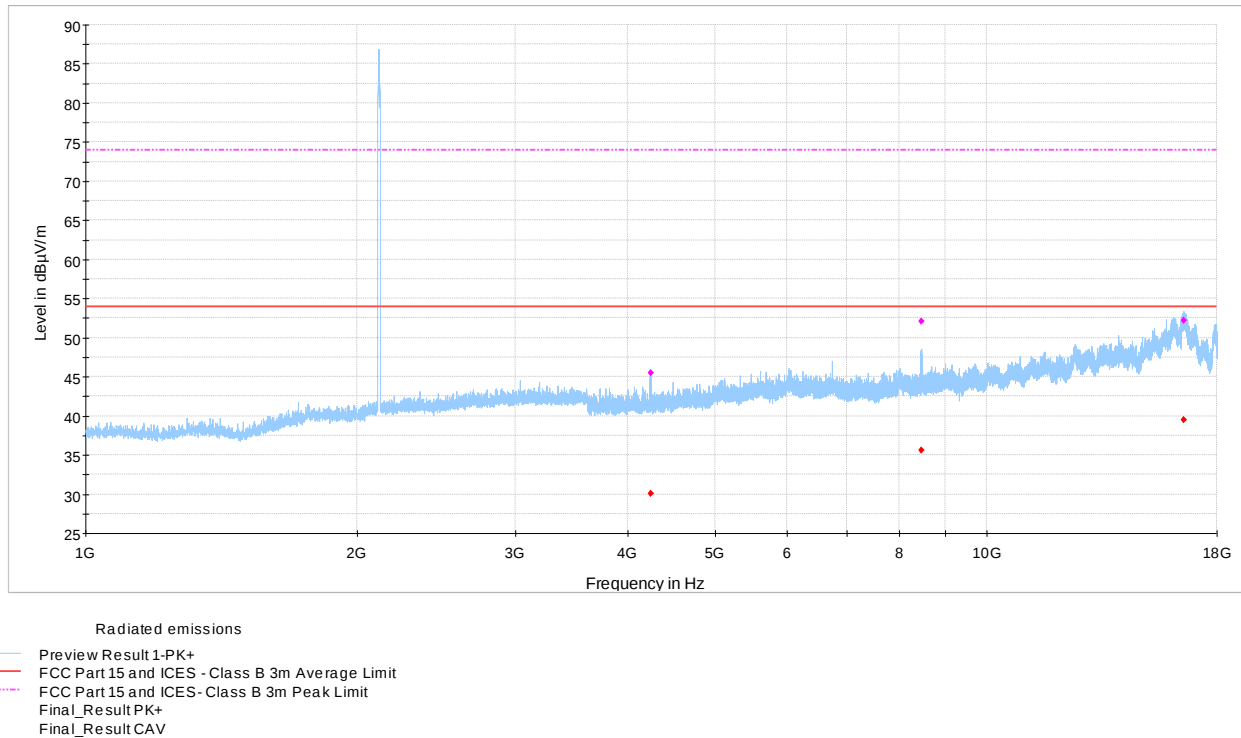
Figure 8.3-22: Radiated emissions spectral plot (1 to 18 GHz) WCDMA
