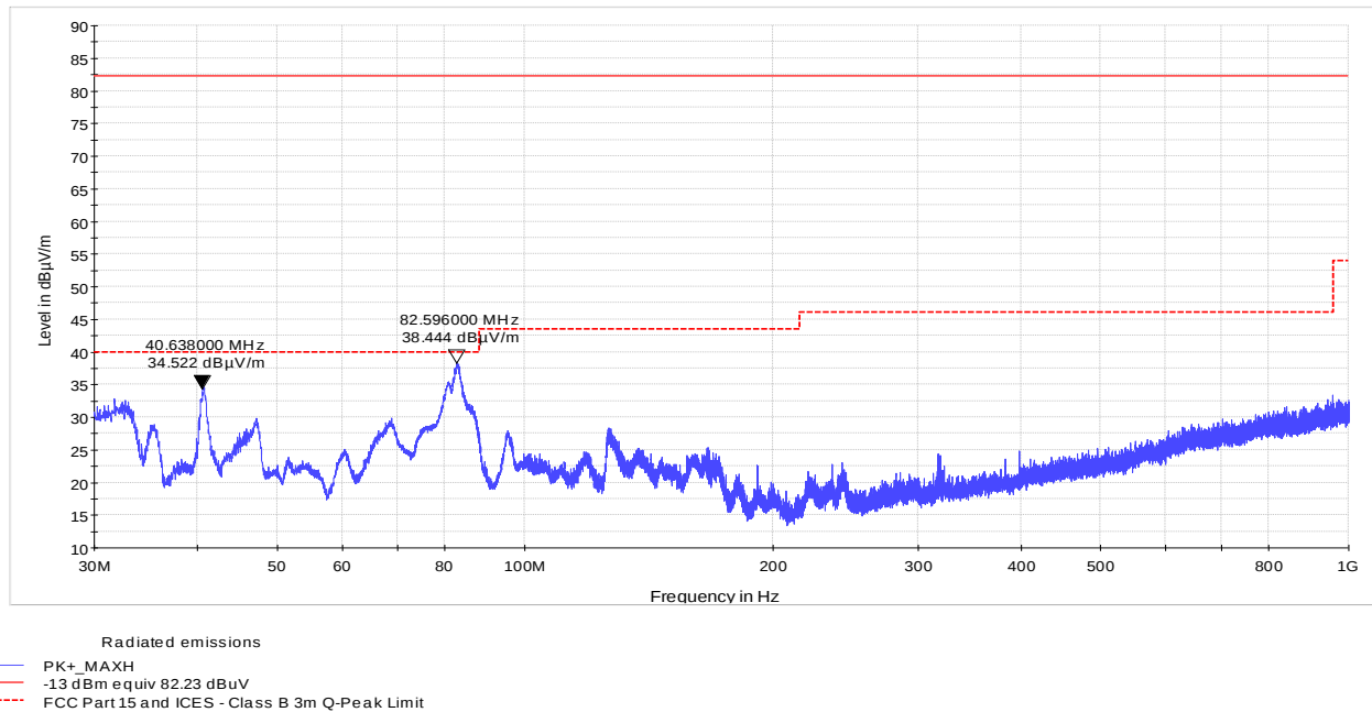
Figure 8.3-16: Radiated emissions spectral plot, WCDMA, two carriers (30 to 1000 MHz)
