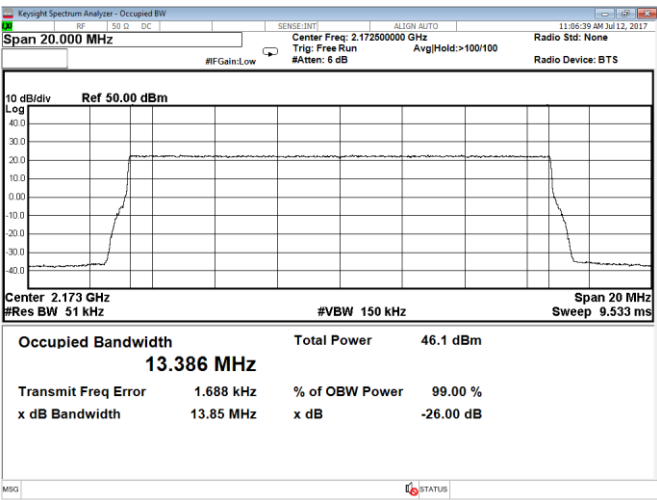
Figure 8.5-18: Occupied bandwidth, QPSK, LTE, 15 MHz, Port B, High channel
