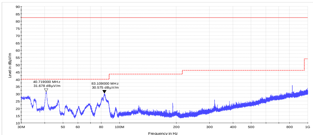
Figure 8.3-13: Radiated emissions spectral plot, WCDMA, low channel (30 to 1000 MHz)
