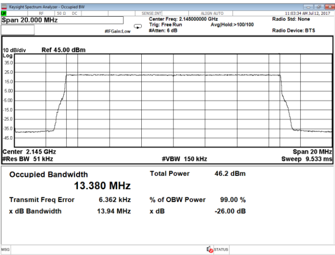
Figure 8.5-14: Occupied bandwidth, QPSK, LTE, 15 MHz, Port A, Mid channel
