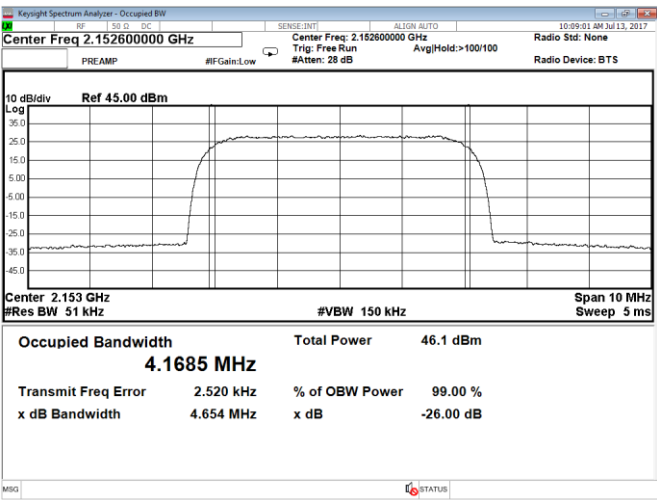
Figure 8.5-30: Occupied bandwidth, QPSK, WCDMA, 5 MHz, Port B, High channel
