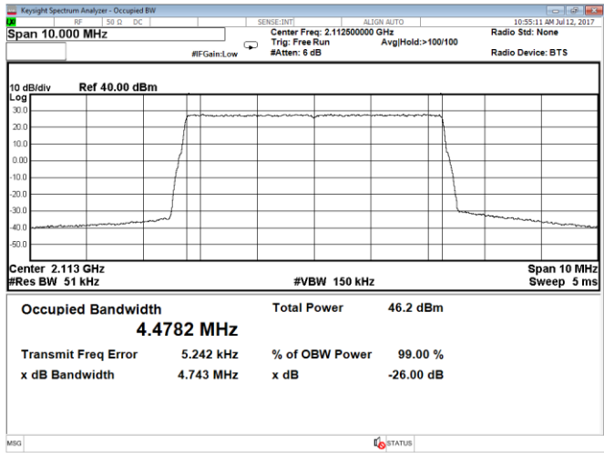
Figure 8.5-1: Occupied bandwidth, QPSK, LTE, 5 MHz, Port A, Low channel
