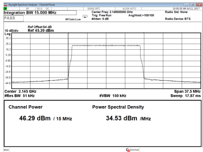
Figure 8.1-24: Output power at mid channel, QPSK, 15 MHz, LTE, Port A
