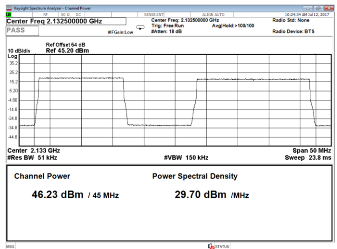
Figure 8.1-64: Output power 2 carriers, QPSK, carrier 1: 15 MHz, carrier 2: 20 MHz, LTE, Port A, bottom range
