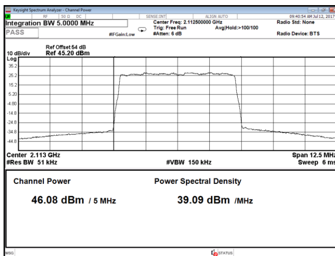
Figure 8.1-14: Output power at low channel, 16QAM, 5 MHz, LTE, Port B
