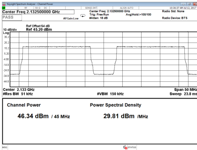
Figure 8.1-73: Output power 2 carriers, QPSK, carrier 1: 20 MHz, carrier 2: 20 MHz, LTE, Port B, bottom range
