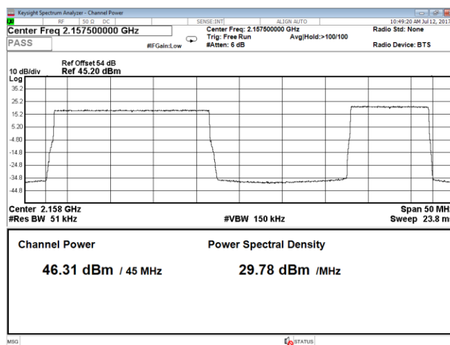
Figure 8.1-56: Output power 2 carriers, QPSK, carrier 1: 20 MHz, carrier 2: 10 MHz, LTE, Port A, top range
