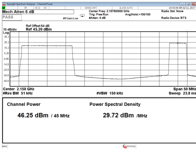
Figure 8.1-41: Output power 2 carriers, QPSK, carrier 1: 15 MHz, carrier 2: 5 MHz, LTE, Port A, top range
