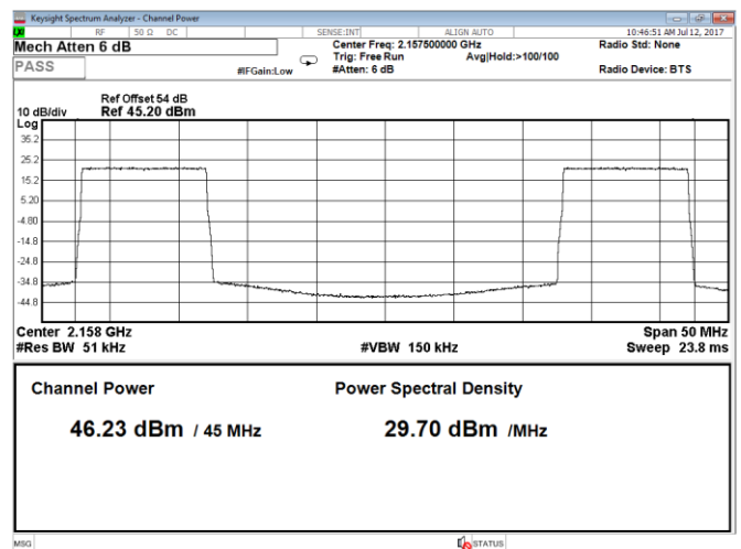
Figure 8.1-60: Output power 2 carriers, QPSK, carrier 1: 10 MHz, carrier 2: 10 MHz, LTE, Port B, top range
