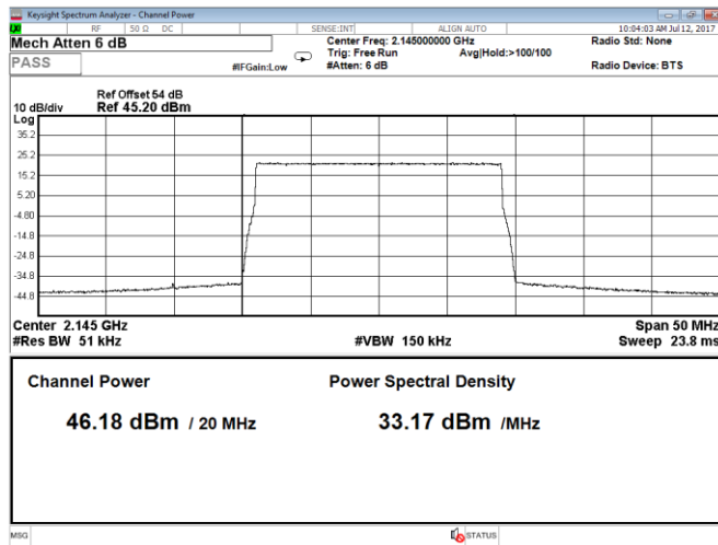
Figure 8.1-33: Output power at mid channel, QPSK, 20 MHz, LTE, Port B
