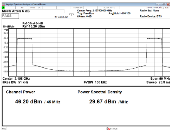
Figure 8.1-47: Output power 2 carriers, QPSK, carrier 1: 5 MHz, carrier 2: 5 MHz, LTE, Port B, top range
