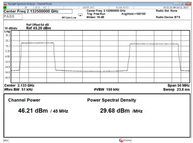
Figure 8.1-58: Output power 2 carriers, QPSK, carrier 1: 10 MHz, carrier 2: 15 MHz, LTE, Port B, bottom range
