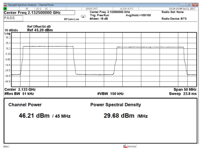
Figure 8.1-68: Output power 2 carriers, QPSK, carrier 1: 15 MHz, carrier 2: 20 MHz, LTE, Port B, bottom range
