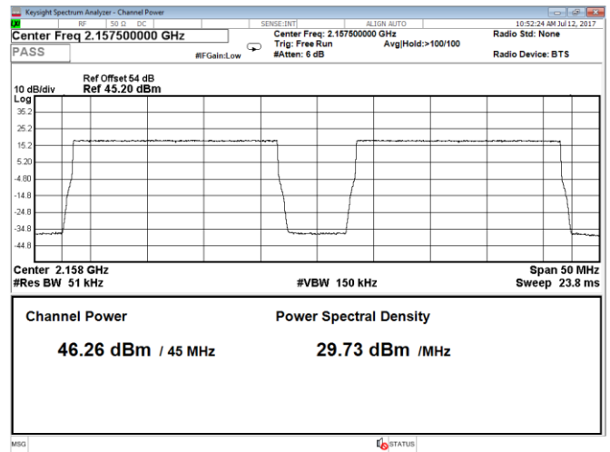
Figure 8.1-74: Output power 2 carriers, QPSK, carrier 1: 20 MHz, carrier 2: 20 MHz, LTE, Port B, top range
