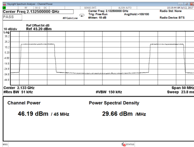
Figure 8.1-57: Output power 2 carriers, QPSK, carrier 1: 10 MHz, carrier 2: 10 MHz, LTE, Port B, bottom range
