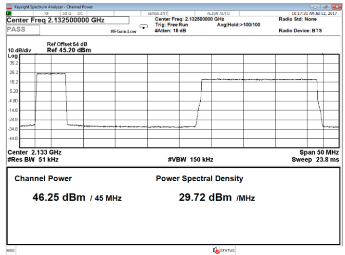
Figure 8.1-38: Output power 2 carriers, QPSK, carrier 1: 5 MHz, carrier 2: 20 MHz, LTE, Port A, bottom range
