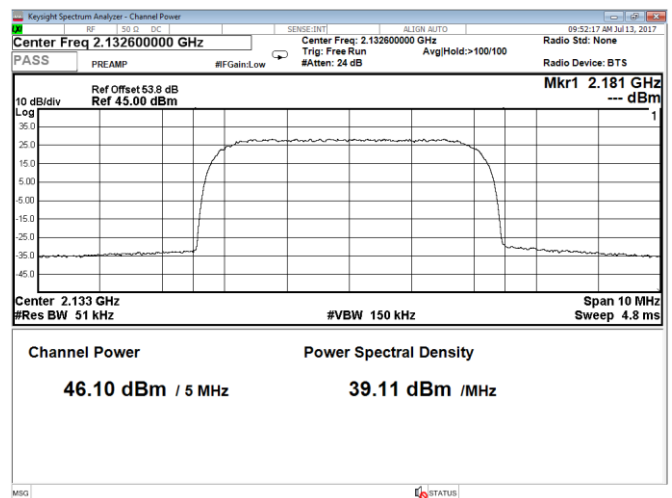
Figure 8.1-76: Output power at mid channel, QPSK, 5 MHz, WCDMA, Port A
