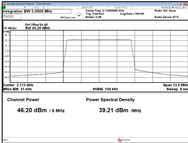
Figure 8.1-5: Output power at low channel, QPSK, 5 MHz, LTE, Port A
