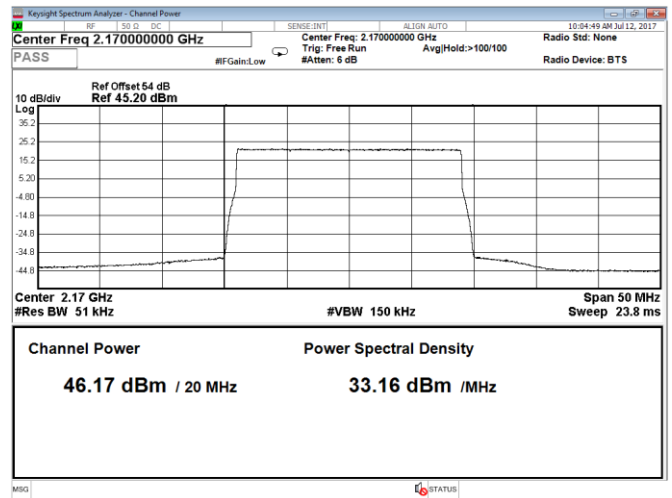
Figure 8.1-34: Output power at high channel, QPSK, 20 MHz, LTE, Port B
