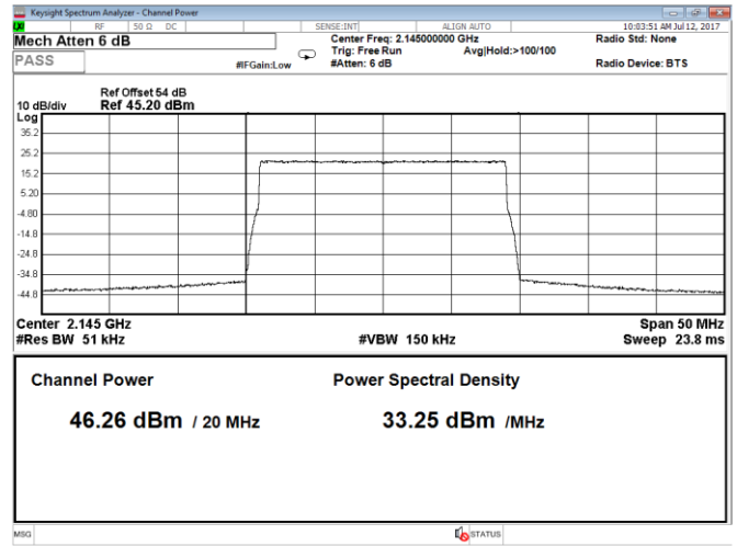
Figure 8.1-30: Output power at mid channel, QPSK, 20 MHz, LTE, Port A
