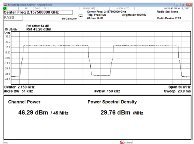
Figure 8.1-72: Output power 2 carriers, QPSK, carrier 1: 20 MHz, carrier 2: 20 MHz, LTE, Port A, top range
