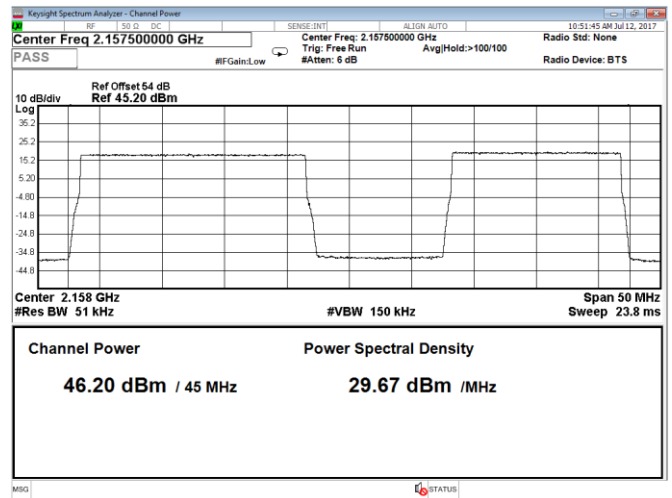
Figure 8.1-70: Output power 2 carriers, QPSK, carrier 1: 20 MHz, carrier 2: 15 MHz, LTE, Port B, top range
