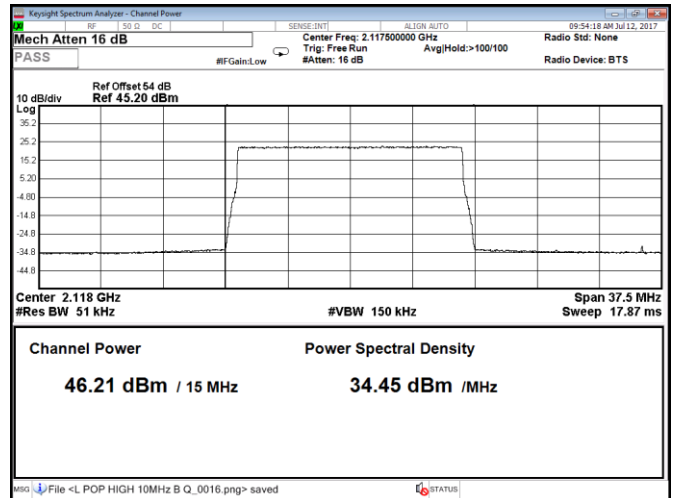
Figure 8.1-26: Output power at low channel, QPSK, 15 MHz, LTE, Port B
