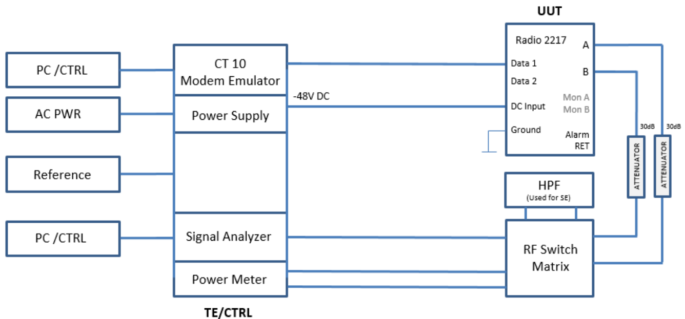
Figure 3.5-1: Setup diagram – Radio Compliance, conducted tests
