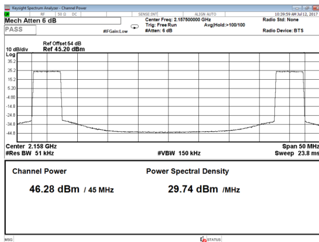
Figure 8.1-39: Output power 2 carriers, QPSK, carrier 1: 5 MHz, carrier 2: 5 MHz, LTE, Port A, top range
