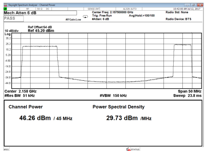
Figure 8.1-40: Output power 2 carriers, QPSK, carrier 1: 10 MHz, carrier 2: 5 MHz, LTE, Port A, top range
