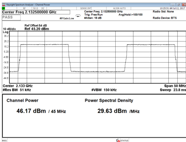
Figure 8.1-67: Output power 2 carriers, QPSK, carrier 1: 15 MHz, carrier 2: 15 MHz, LTE, Port B, bottom range
