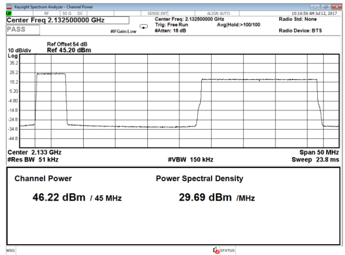
Figure 8.1-46: Output power 2 carriers, QPSK, carrier 1: 5 MHz, carrier 2: 20 MHz, LTE, Port B, bottom range
