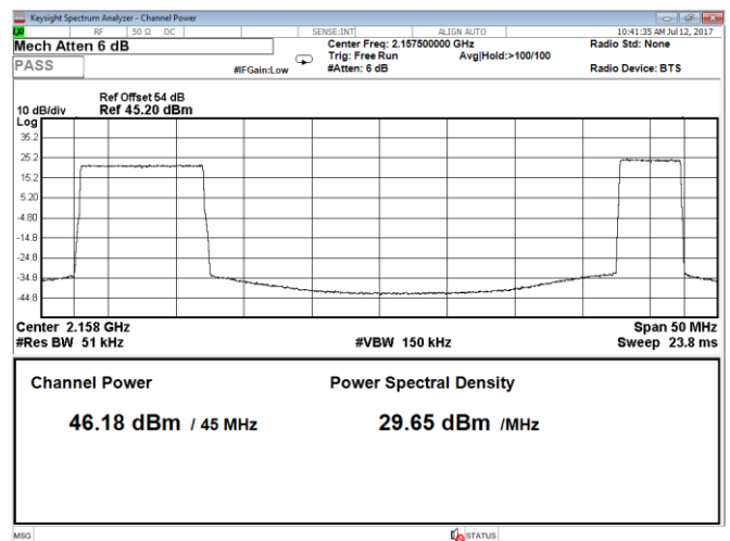
Figure 8.1-48: Output power 2 carriers, QPSK, carrier 1: 10 MHz, carrier 2: 5 MHz, LTE, Port B, top range
