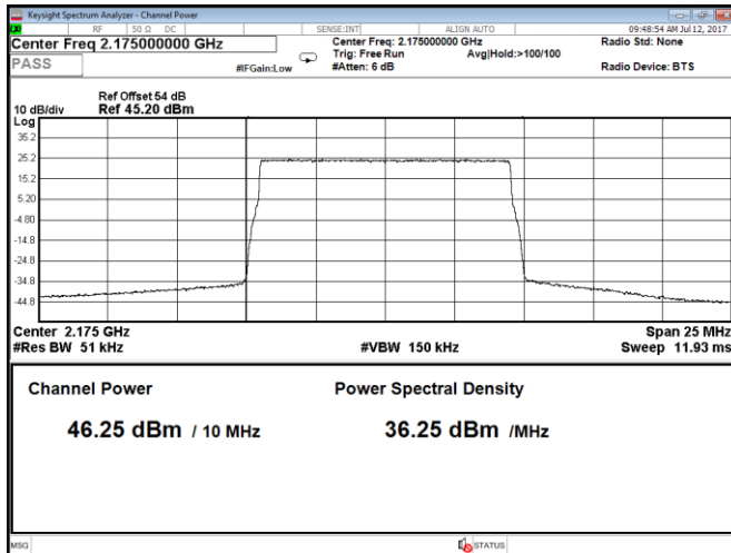
Figure 8.1-19: Output power at high channel, QPSK, 10 MHz, LTE, Port A
