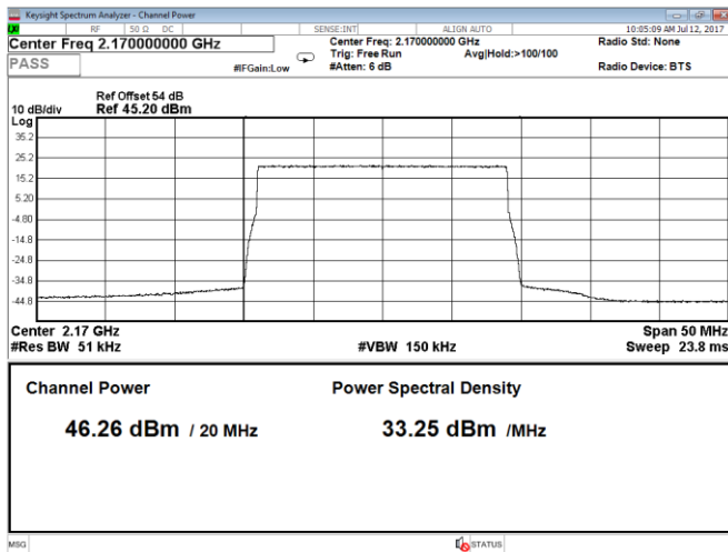
Figure 8.1-31: Output power at high channel, QPSK, 20 MHz, LTE, Port A
