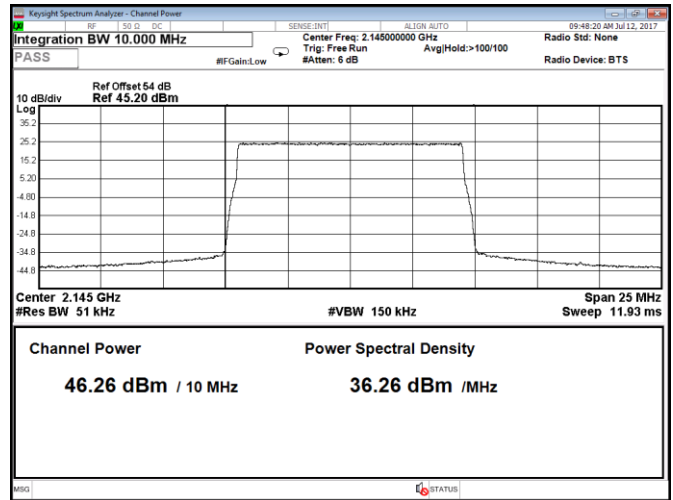
Figure 8.1-18: Output power at mid channel, QPSK, 10 MHz, LTE, Port A
