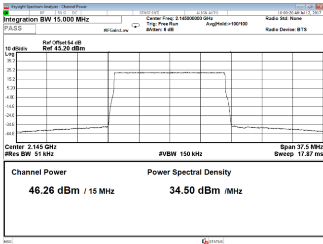
Figure 8.1-27: Output power at mid channel, QPSK, 15 MHz, LTE, Port B
