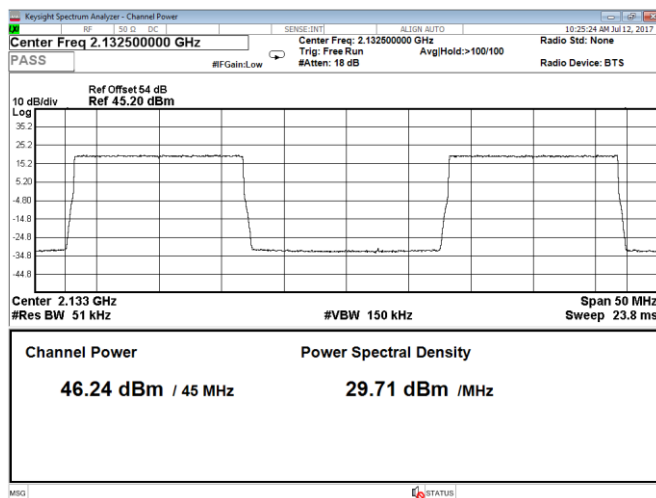
Figure 8.1-63: Output power 2 carriers, QPSK, carrier 1: 15 MHz, carrier 2: 15 MHz, LTE, Port A, bottom range
