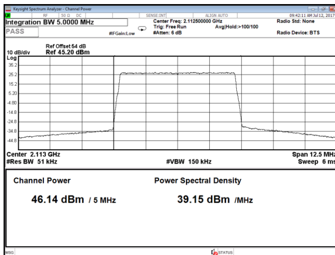
Figure 8.1-16: Output power at low channel, 256QAM, 5 MHz, LTE, Port B
