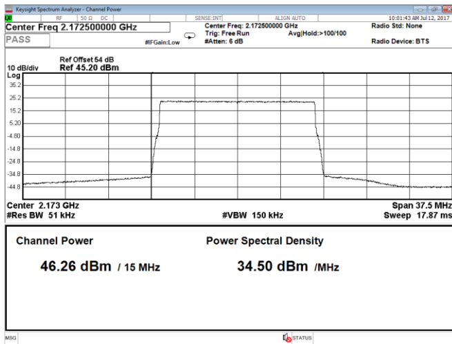
Figure 8.1-25: Output power at high channel, QPSK, 15 MHz, LTE, Port A
