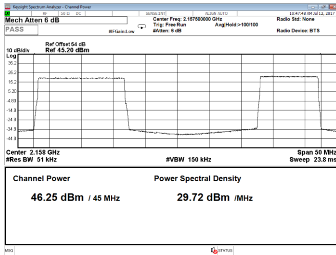
Figure 8.1-61: Output power 2 carriers, QPSK, carrier 1: 15 MHz, carrier 2: 10 MHz, LTE, Port B, top range
