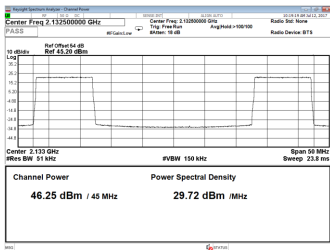
Figure 8.1-51: Output power 2 carriers, QPSK, carrier 1: 10 MHz, carrier 2: 10 MHz, LTE, Port A, bottom range
