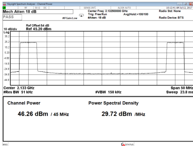
Figure 8.1-35: Output power 2 carriers, QPSK, carrier 1: 5 MHz, carrier 2: 5 MHz, LTE, Port A, bottom range
