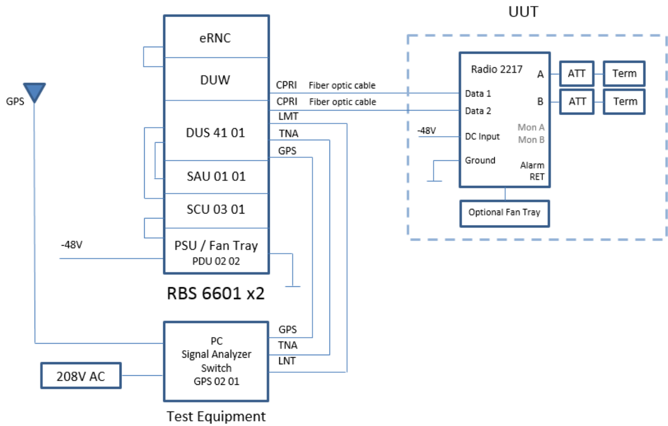
Figure 3.6-3: EUT Set-up for Radiated Emissions Compliance Testing
