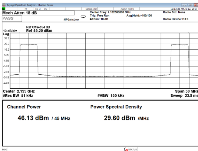
Figure 8.1-43: Output power 2 carriers, QPSK, carrier 1: 5 MHz, carrier 2: 5 MHz, LTE, Port B, bottom range
