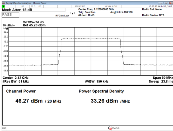
Figure 8.1-29: Output power at low channel, QPSK, 20 MHz, LTE, Port A
