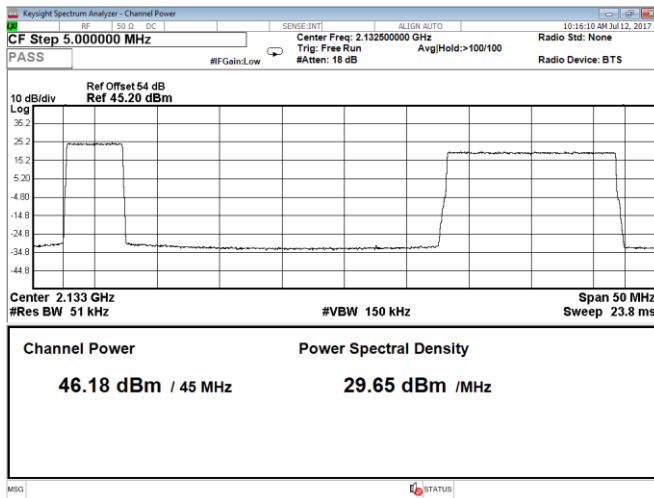
Figure 8.1-45: Output power 2 carriers, QPSK, carrier 1: 5 MHz, carrier 2: 15 MHz, LTE, Port B, bottom range
