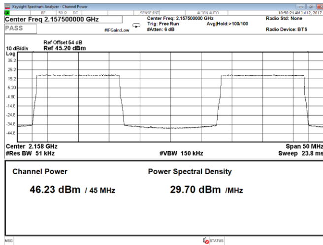
Figure 8.1-69: Output power 2 carriers, QPSK, carrier 1: 15 MHz, carrier 2: 15 MHz, LTE, Port B, top range
