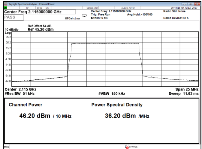
Figure 8.1-20: Output power at low channel, QPSK, 10 MHz, LTE, Port B
