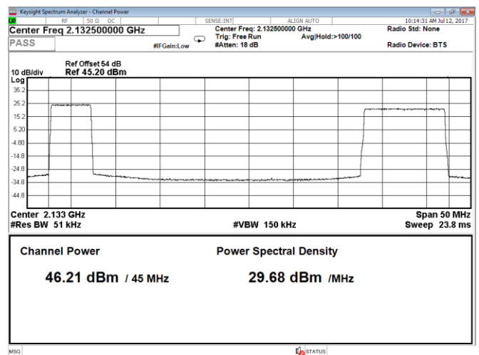
Figure 8.1-44: Output power 2 carriers, QPSK, carrier 1: 5 MHz, carrier 2: 10 MHz, LTE, Port B, bottom range
