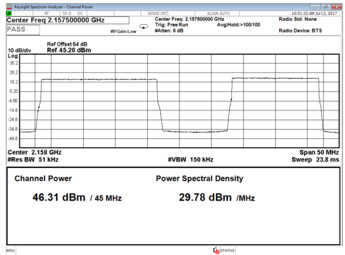
Figure 8.1-66: Output power 2 carriers, QPSK, carrier 1: 20 MHz, carrier 2: 15 MHz, LTE, Port A, top range
