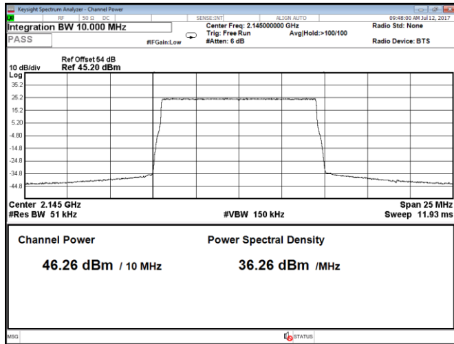
Figure 8.1-21: Output power at mid channel, QPSK, 10 MHz, LTE, Port B
