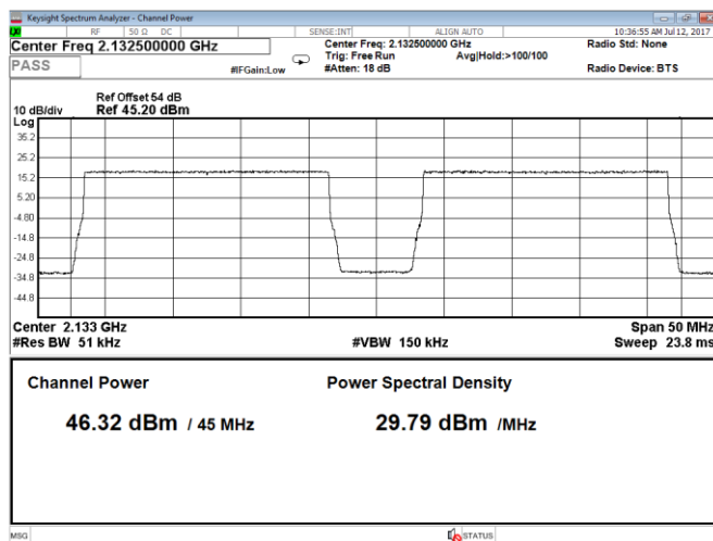
Figure 8.1-71: Output power 2 carriers, QPSK, carrier 1: 20 MHz, carrier 2: 20 MHz, LTE, Port A, bottom range
