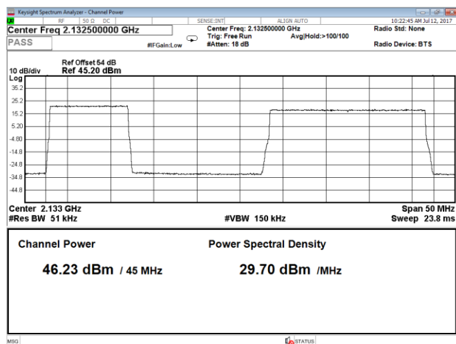
Figure 8.1-53: Output power 2 carriers, QPSK, carrier 1: 10 MHz, carrier 2: 20 MHz, LTE, Port A, bottom range
