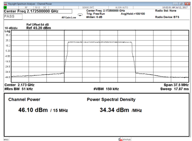
Figure 8.1-28: Output power at high channel, QPSK, 15 MHz, LTE, Port B
