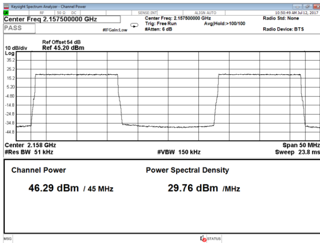
Figure 8.1-65: Output power 2 carriers, QPSK, carrier 1: 15 MHz, carrier 2: 15 MHz, LTE, Port A, top range
