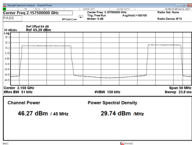
Figure 8.1-55: Output power 2 carriers, QPSK, carrier 1: 15 MHz, carrier 2: 10 MHz, LTE, Port A, top range
