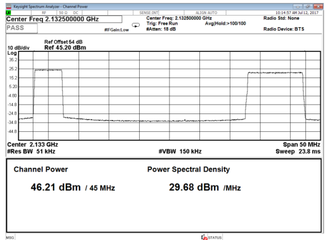
Figure 8.1-36: Output power 2 carriers, QPSK, carrier 1: 5 MHz, carrier 2: 10 MHz, LTE, Port A, bottom range
