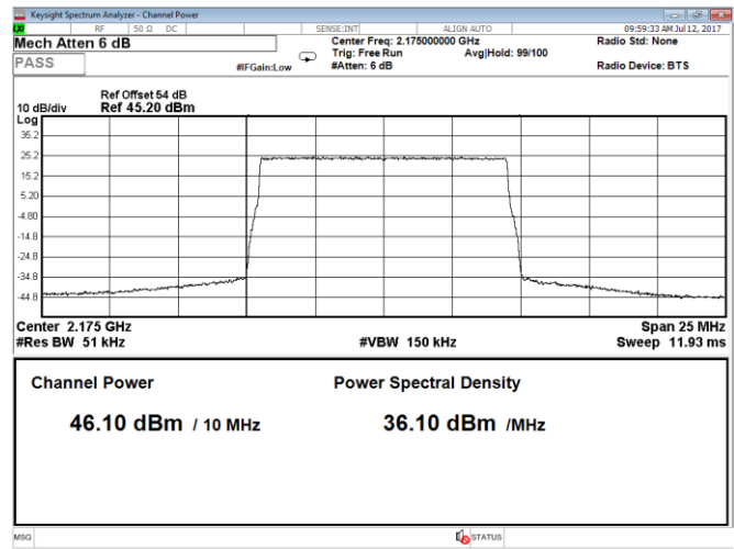
Figure 8.1-22: Output power at high channel, QPSK, 10 MHz, LTE, Port B
