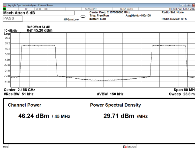
Figure 8.1-54: Output power 2 carriers, QPSK, carrier 1: 10 MHz, carrier 2: 10 MHz, LTE, Port A, top range
