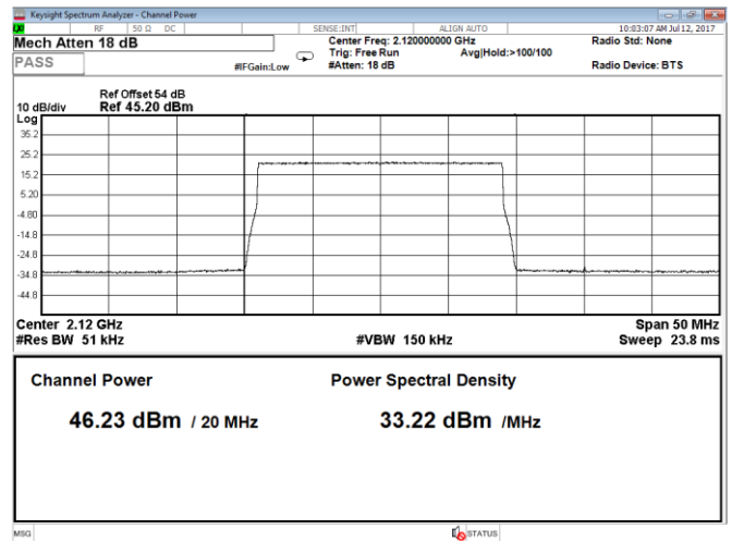
Figure 8.1-32: Output power at low channel, QPSK, 20 MHz, LTE, Port B
