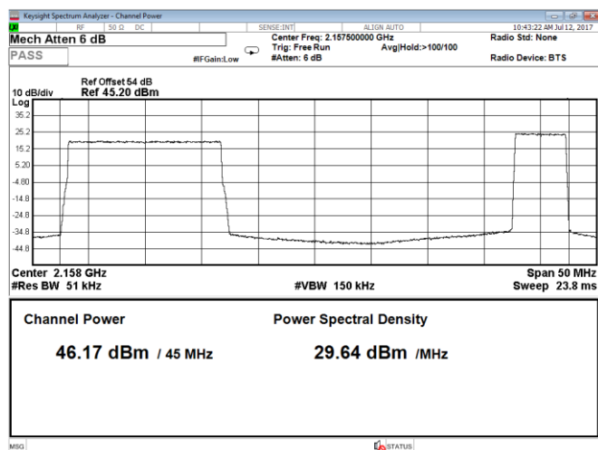
Figure 8.1-49: Output power 2 carriers, QPSK, carrier 1: 15 MHz, carrier 2: 5 MHz, LTE, Port B, top range
