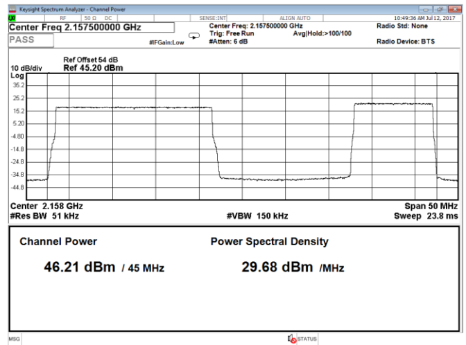
Figure 8.1-62: Output power 2 carriers, QPSK, carrier 1: 20 MHz, carrier 2: 10 MHz, LTE, Port B, top range
