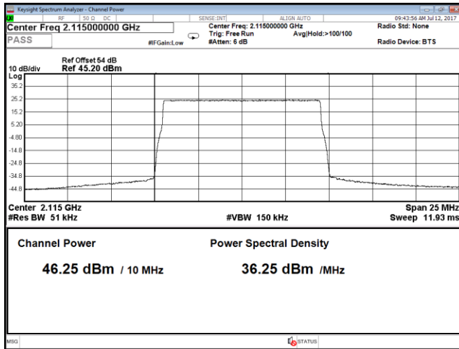
Figure 8.1-17: Output power at low channel, QPSK, 10 MHz, LTE, Port A
