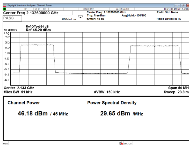
Figure 8.1-52: Output power 2 carriers, QPSK, carrier 1: 10 MHz, carrier 2: 15 MHz, LTE, Port A, bottom range
