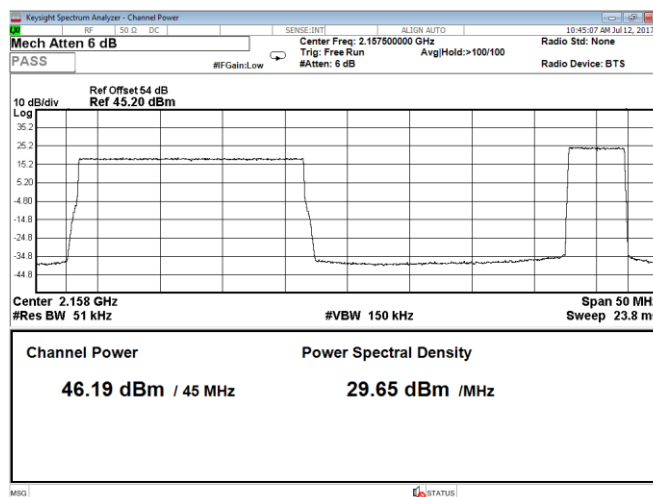
Figure 8.1-50: Output power 2 carriers, QPSK, carrier 1: 20 MHz, carrier 2: 5 MHz, LTE, Port B, top range
