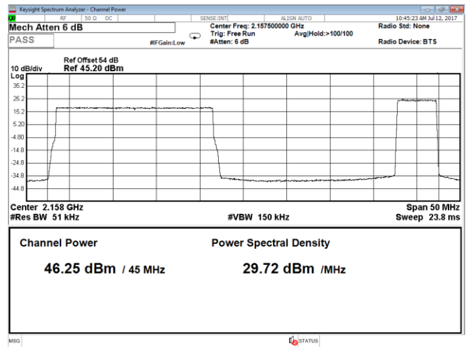
Figure 8.1-42: Output power 2 carriers, QPSK, carrier 1: 20 MHz, carrier 2: 5 MHz, LTE, Port A, top range
