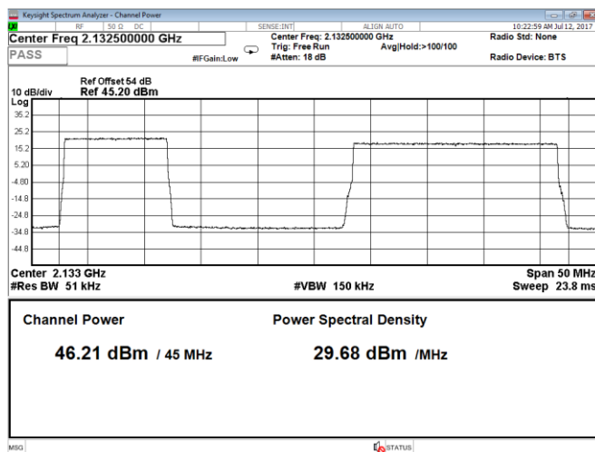
Figure 8.1-59: Output power 2 carriers, QPSK, carrier 1: 10 MHz, carrier 2: 20 MHz, LTE, Port B, bottom range
