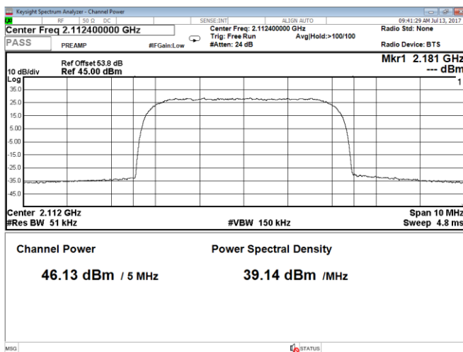
Figure 8.1-75: Output power at low channel, QPSK, 5 MHz, WCDMA, Port A
