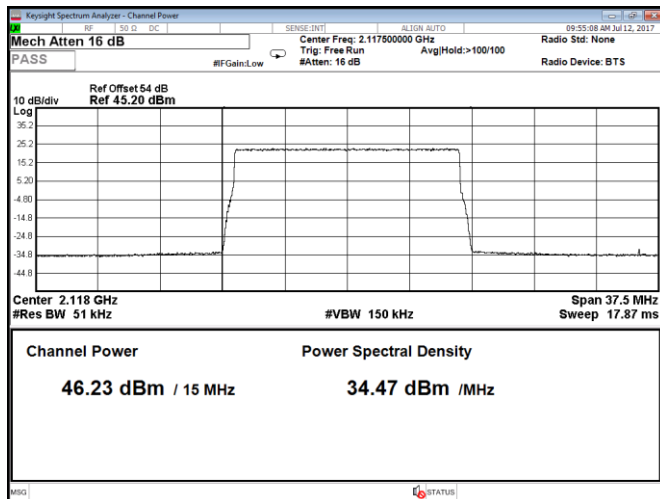
Figure 8.1-23: Output power at low channel, QPSK, 15 MHz, LTE, Port A
