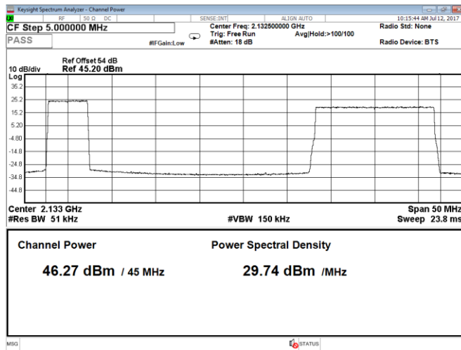
Figure 8.1-37: Output power 2 carriers, QPSK, carrier 1: 5 MHz, carrier 2: 15 MHz, LTE, Port A, bottom range
