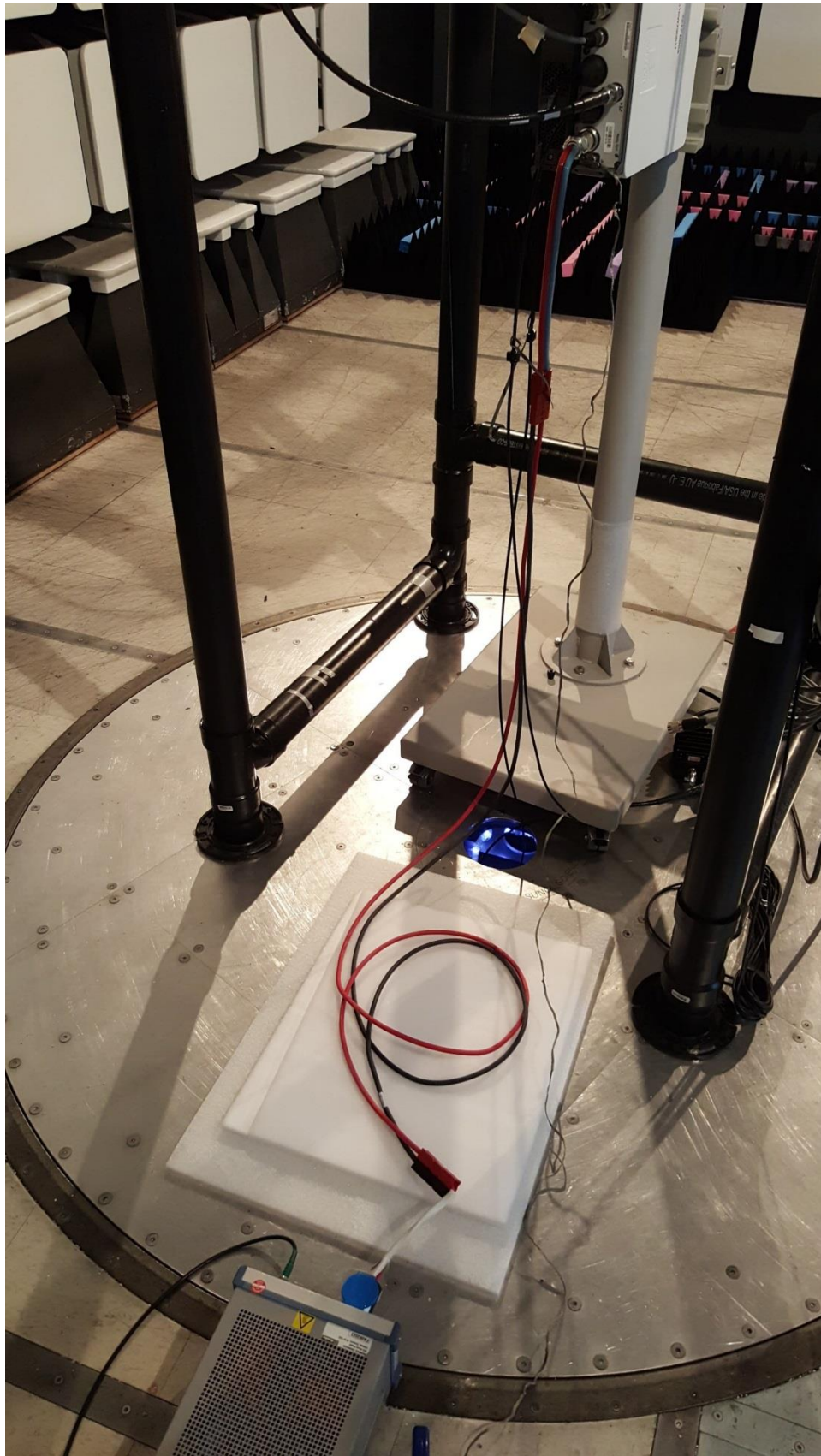
EUT Set-up for Conducted emissions on AC line Compliance Testing
