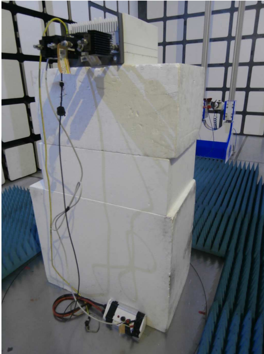
Radiated Emissions 1 GHz to 9 GHz
