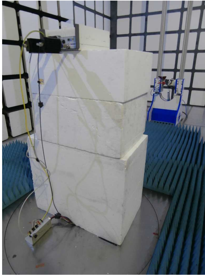
Radiated Emissions 1 GHz to 9 GHz
