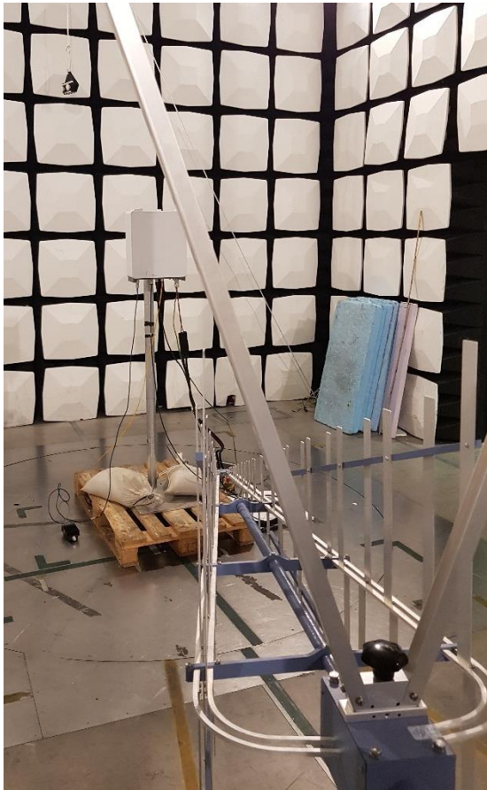
30 – 1000 MHz
