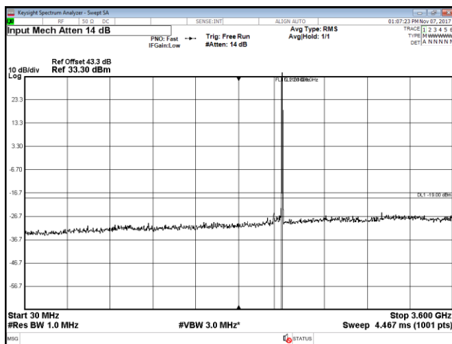
Figure 8.2-11: Conducted spurious emissions within 30–3600 MHz, Port B, LTE, 5 MHz high channel, QPSK
