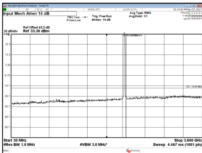
Figure 8.2-51: Conducted spurious emissions within 30–3600 MHz, Port A, LTE, 15 MHz mid channel, QPSK
