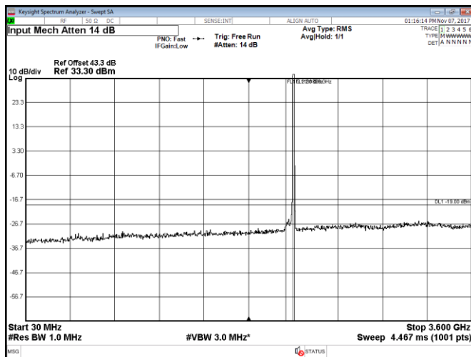
Figure 8.2-71: Conducted spurious emissions within 30–3600 MHz, Port D, LTE, 15 MHz high channel, QPSK
