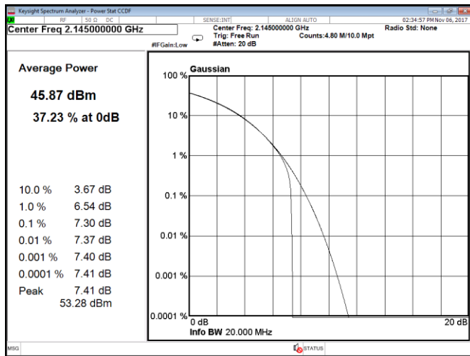
Figure 8.1-209: CCDF, QPSK, 20 MHz, LTE, Port B, mid channel
