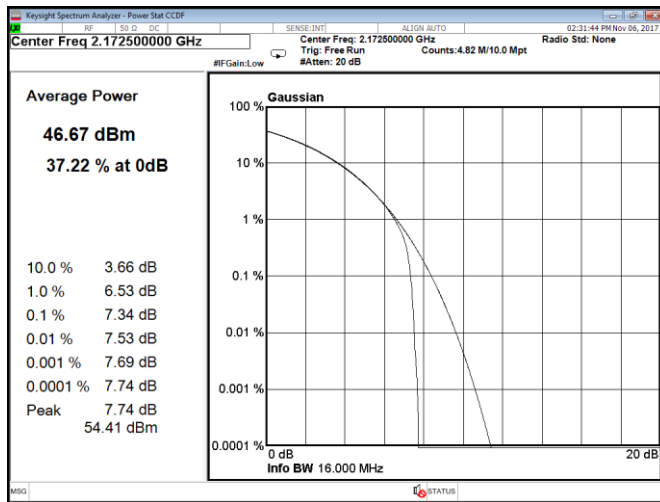
Figure 8.1-201: CCDF, QPSK, 15 MHz, LTE, Port C, high channel
