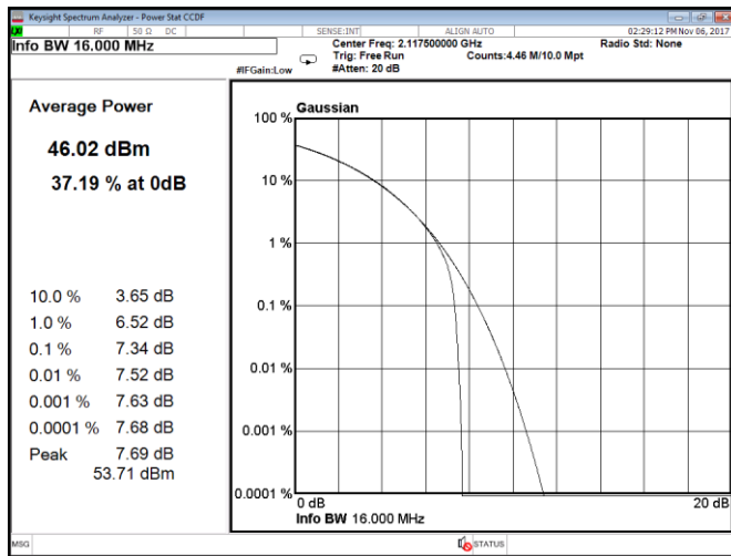
Figure 8.1-193: CCDF, QPSK, 15 MHz, LTE, Port A, low channel
