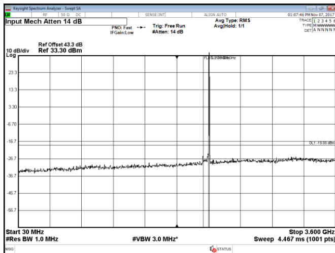
Figure 8.2-23: Conducted spurious emissions within 30–3600 MHz, Port D, LTE, 5 MHz high channel, QPSK
