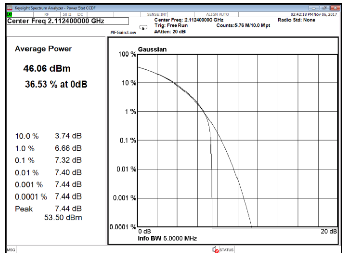
Figure 8.1-220: CCDF, QPSK, WCDMA, Port B, low channel
