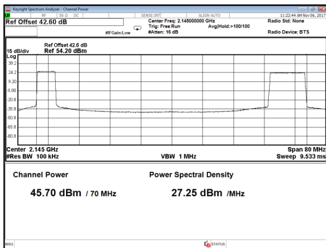
Figure 8.1-71: Output power 2 carriers, QPSK, carrier 1: 5 MHz, carrier 2: 10 MHz, LTE, Port C
