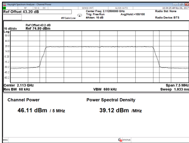
Figure 8.1-9: Output power at low channel, 64QAM, 5 MHz, LTE, Port A
