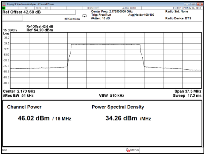
Figure 8.1-49: Output power at high channel, QPSK, 15 MHz, LTE, Port C
