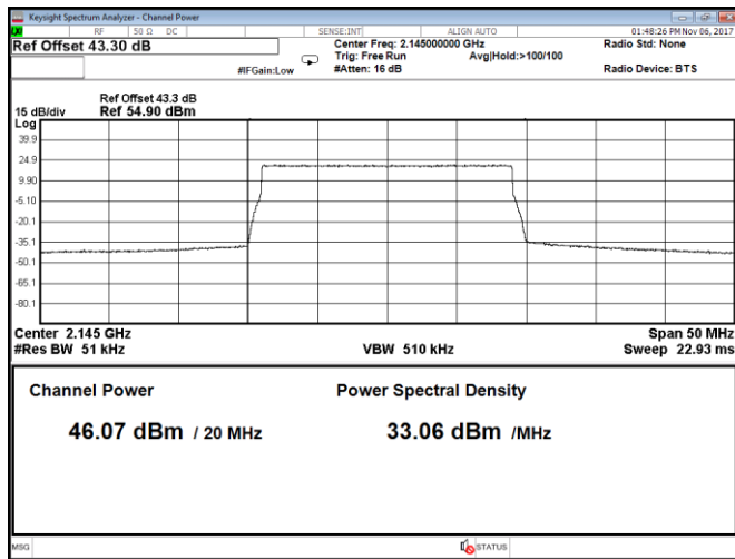
Figure 8.1-57: Output power at mid channel, QPSK, 20 MHz, LTE, Port B
