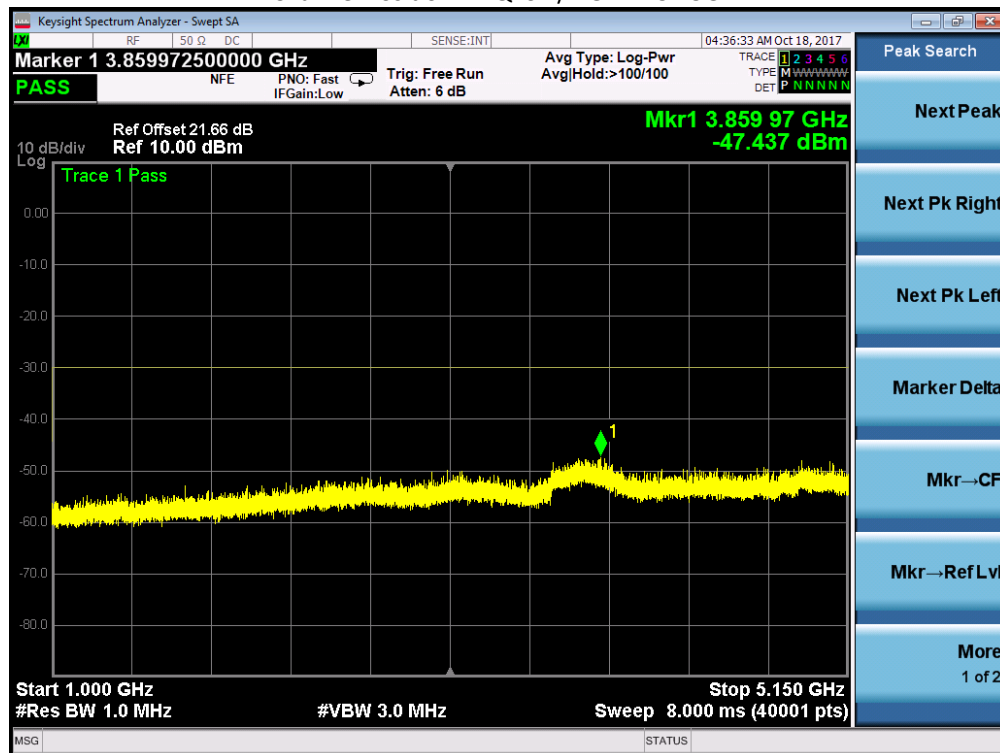
Channel Position B - QPSK / 1GHz – 5.15GHz
