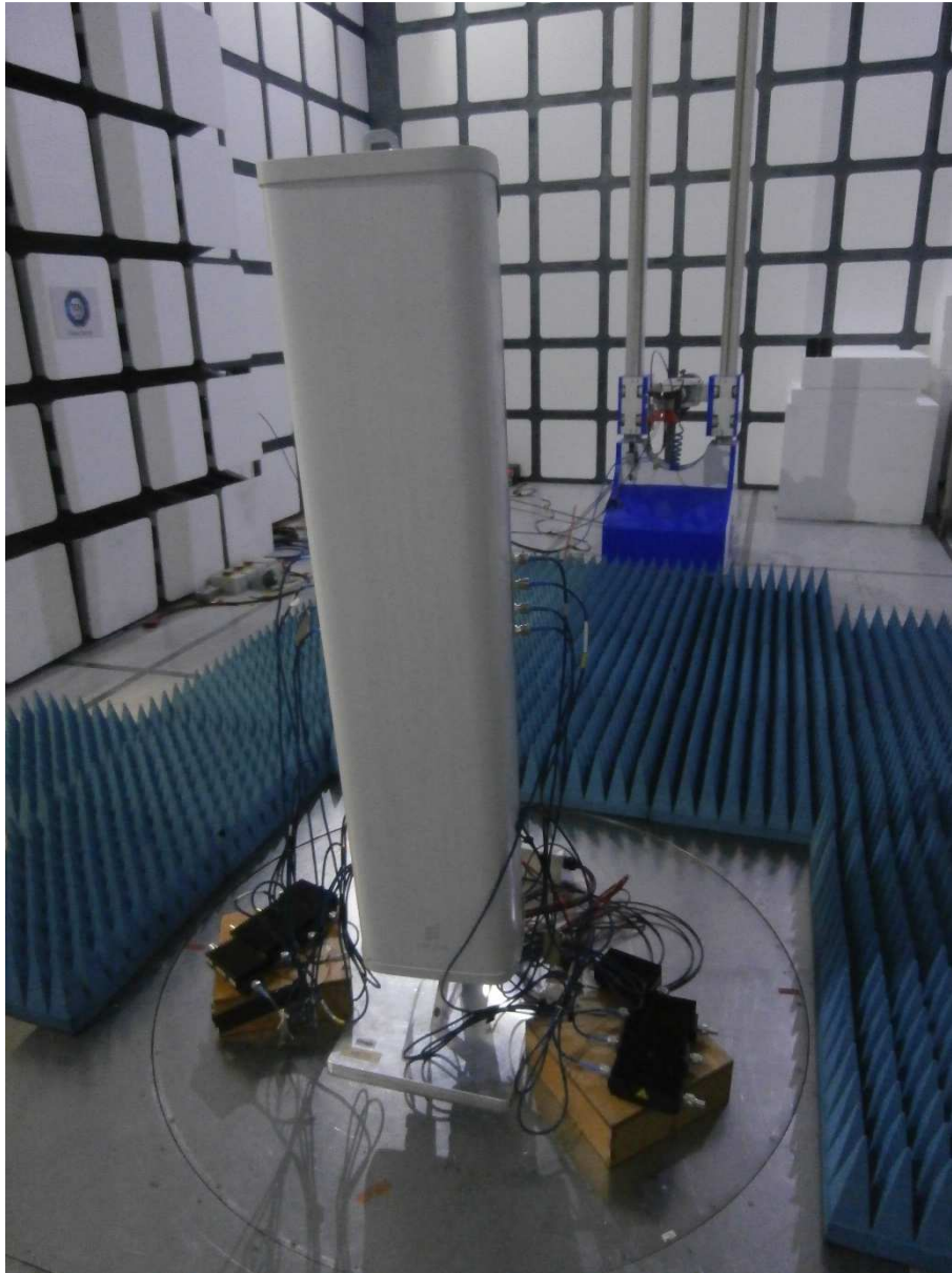
Radiated Emissions 8 GHz to 18 GHz
