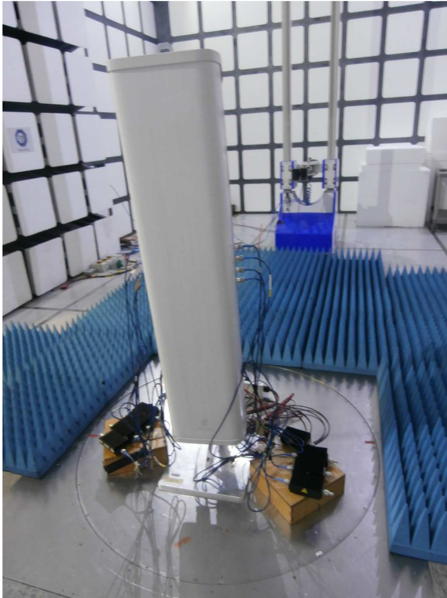
Radiated Emissions 1 GHz to 8 GHz
