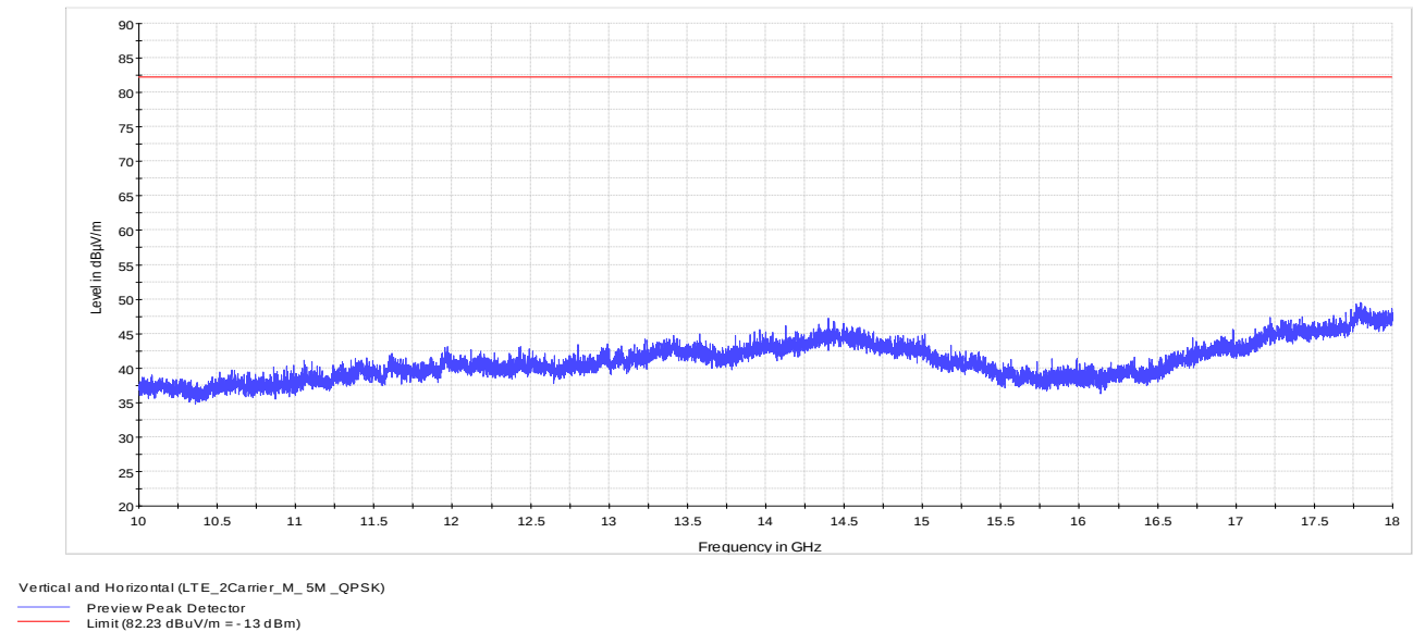
Figure 8.1-19: 10 to 18 GHz – LTE_2Carrier_M_5M_QPSK
