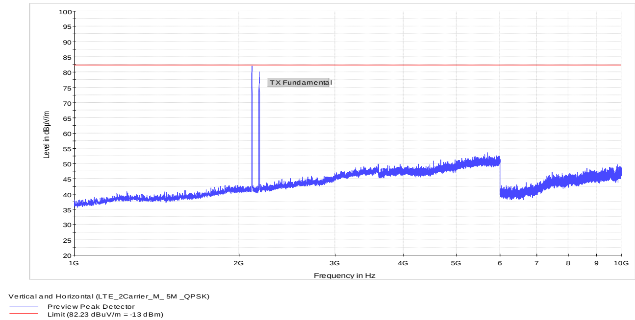
Figure 8.1-18: 1 to 10 GHz – LTE_2Carrier_M_5M_QPSK
