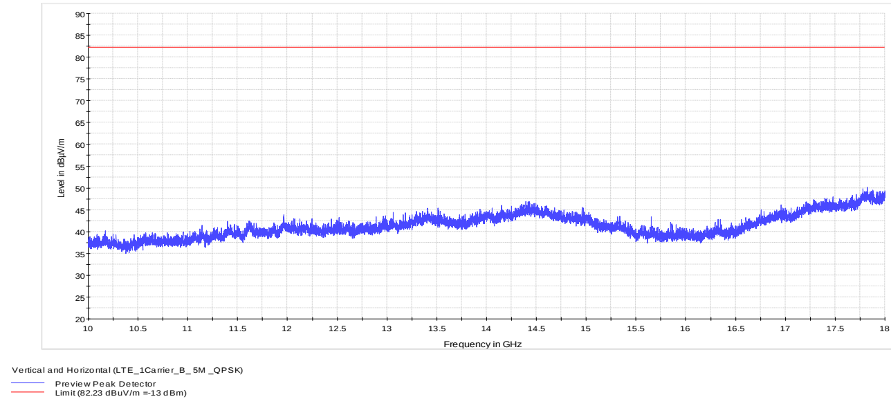
Figure 8.1-7: 10 to 18 GHz – LTE_1Carrier_B_5M_QPSK
