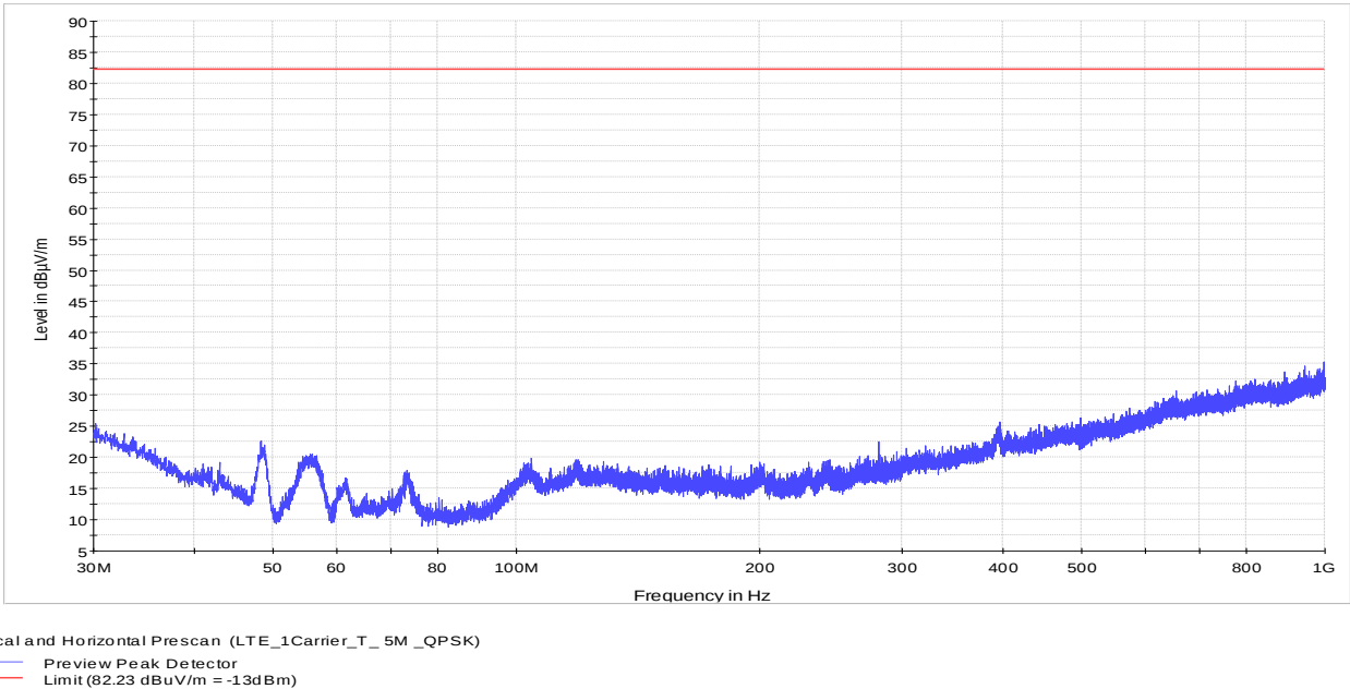
Figure 8.1-13: 30 to 1000 MHz – LTE_1Carrier_T_5M_QPSK
