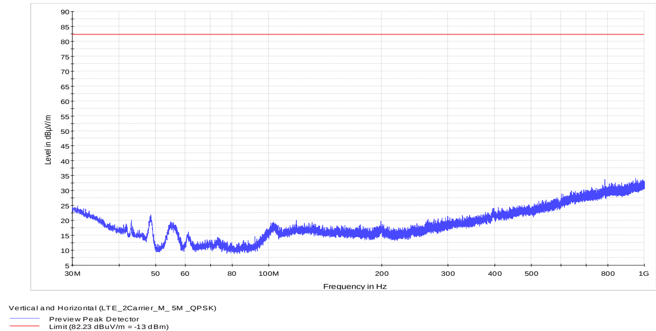
Figure 8.1-17: 30 to 1000 MHz – LTE_2Carrier_M_5M_QPSK
