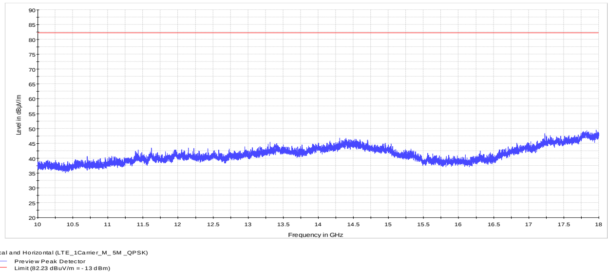
Figure 8.1-11: 10 to 18 GHz – LTE_1Carrier_M_5M_QPSK
