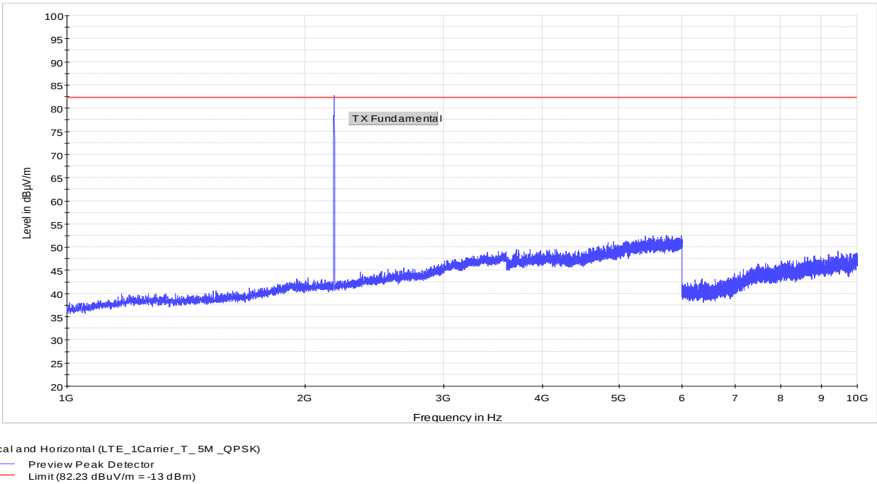
Figure 8.1-14: 1 to 10 GHz – LTE_1Carrier_T_5M_QPSK
