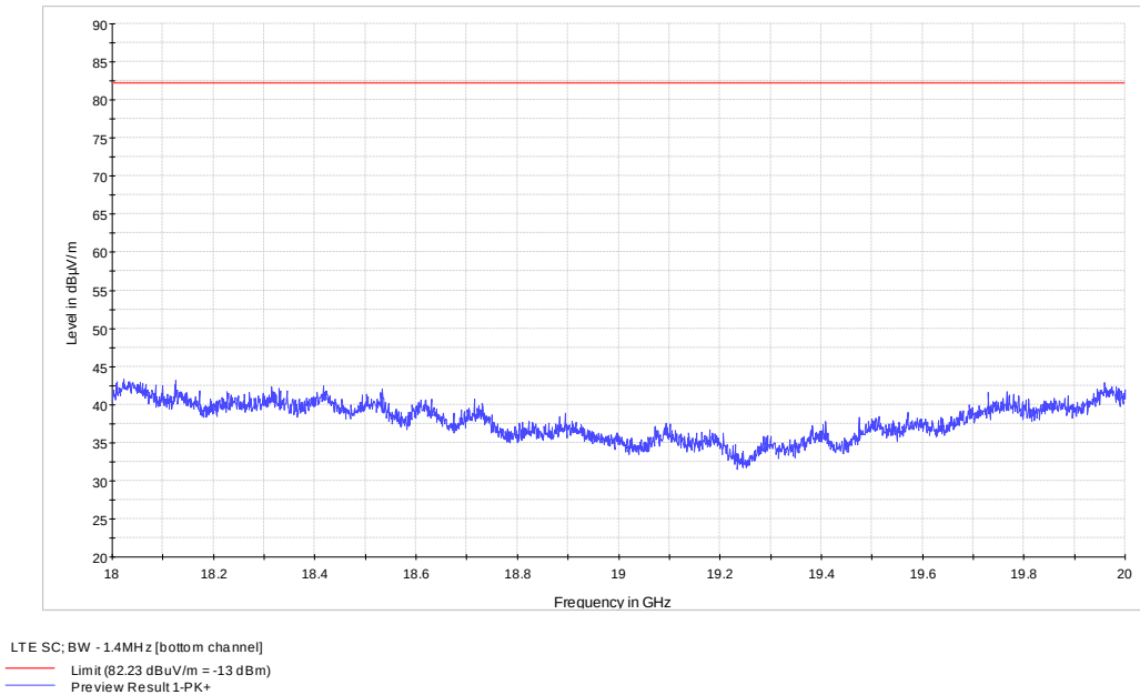
Figure 8.1-6: 18 to 20 GHz – LTE, BW=1.4M, Bottom channel
