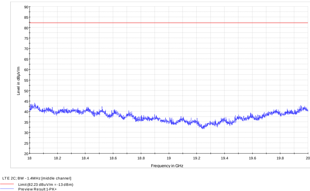
Figure 8.1-12: 18 to 20 GHz – LTE, 2 Carriers, BW=1.4M, Middle channel
