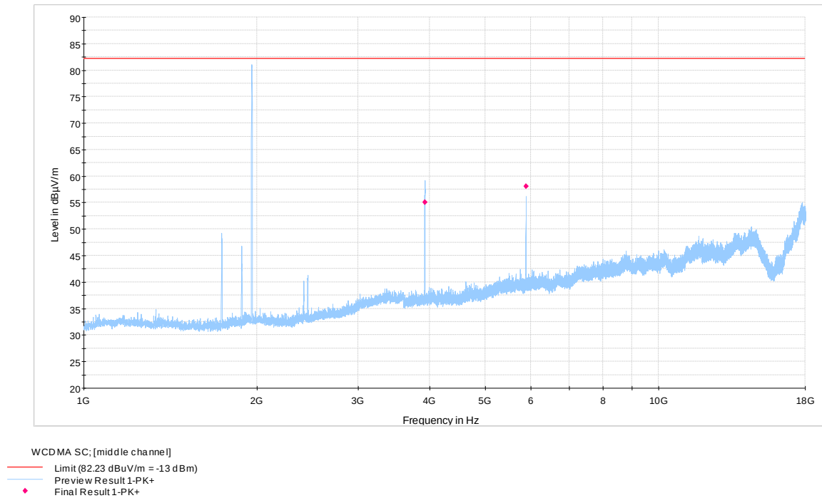
Figure 8.1-14: 1 to 18 GHz – WCDMA, 1 Carrier, Middle Channel
