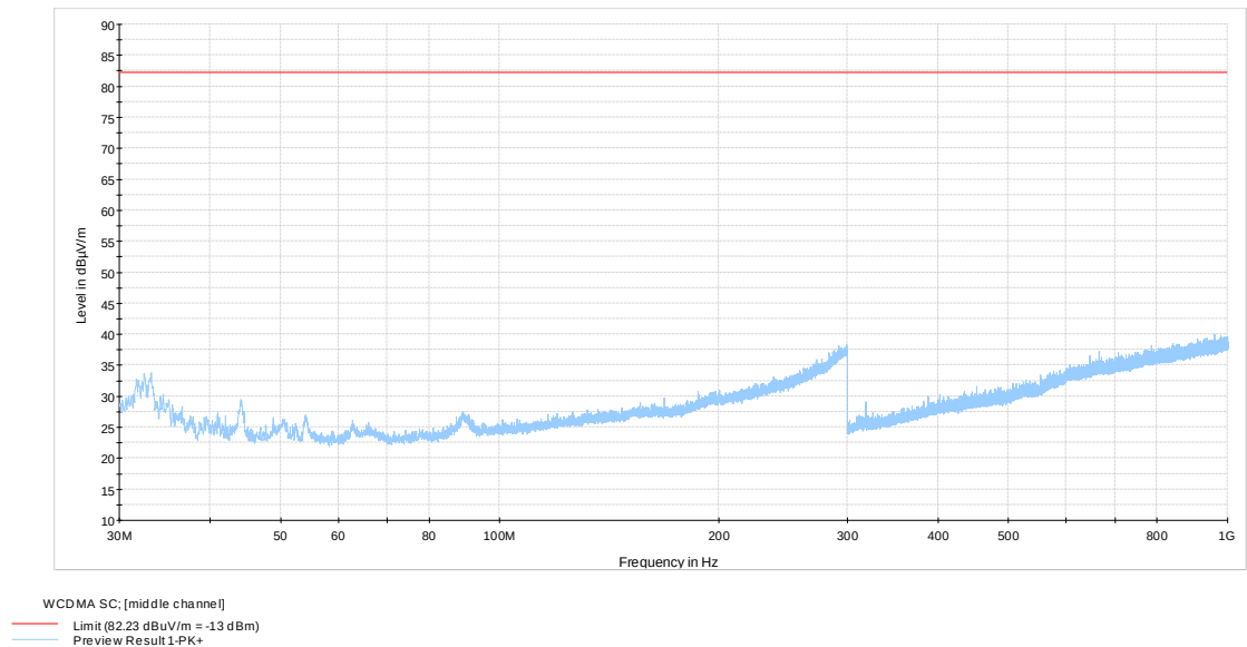
Figure 8.1-13: 30 to 1000 MHz – WCDMA, 1 Carrier, Middle Channel
