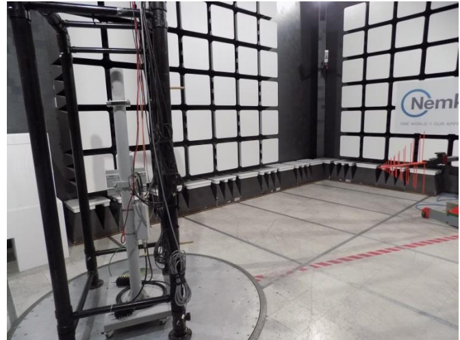
Figure 8.1-19: Setup photo – below 1 GHz
