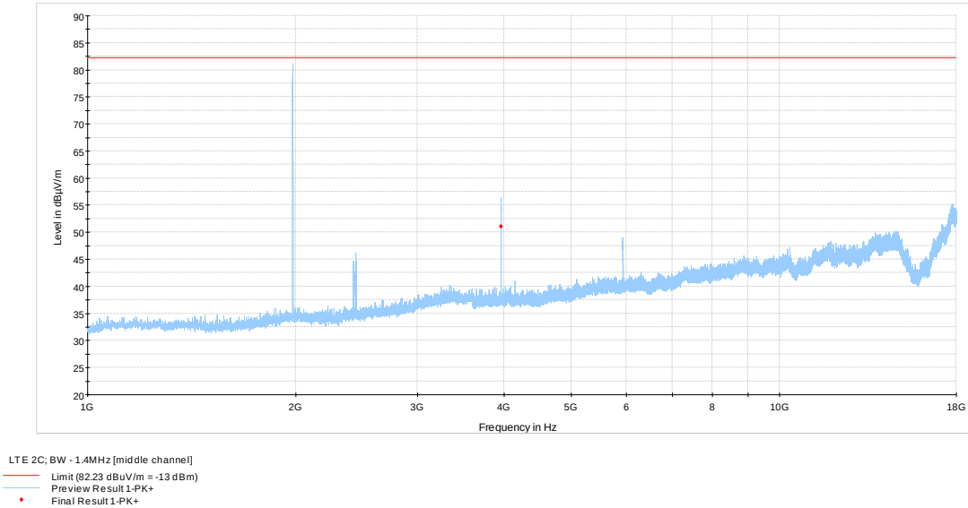
Figure 8.1-11: 1 to 18 GHz – LTE, 2 Carriers, BW=1.4M, Middle channel
