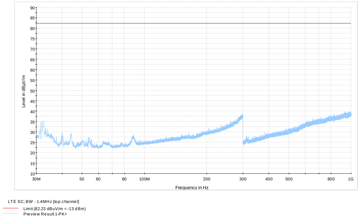
Figure 8.1-7: 30 to 1000 MHz – LTE, BW=1.4M, Top channel
