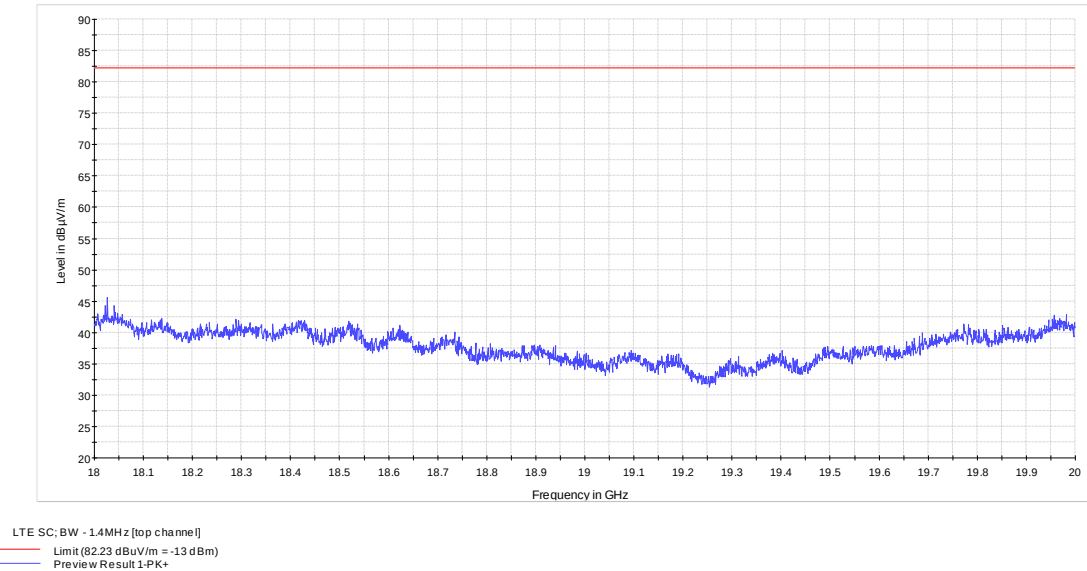
Figure 8.1-9: 18 to 20 GHz – LTE, BW=1.4M, Top channel
