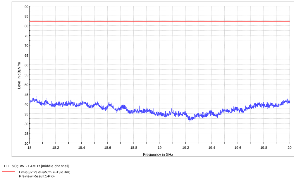
Figure 8.1-3: 18 to 20 GHz – LTE, BW=1.4M, Middle channel
