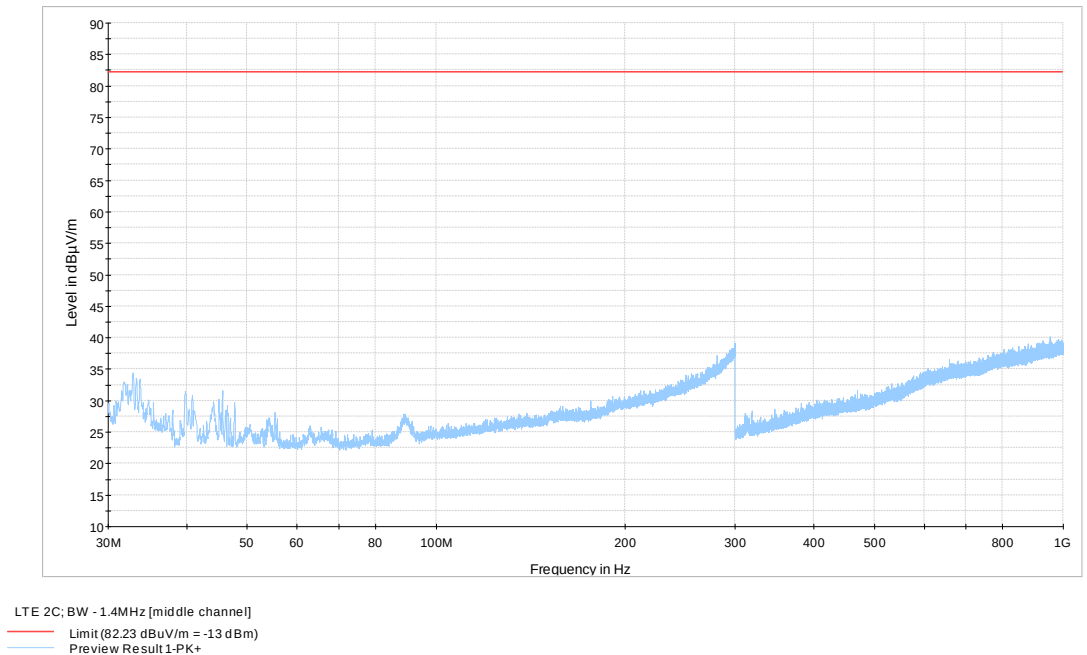
Figure 8.1-10: 30 to 1000 MHz – LTE, 2 Carriers, BW=1.4M, Middle channel
