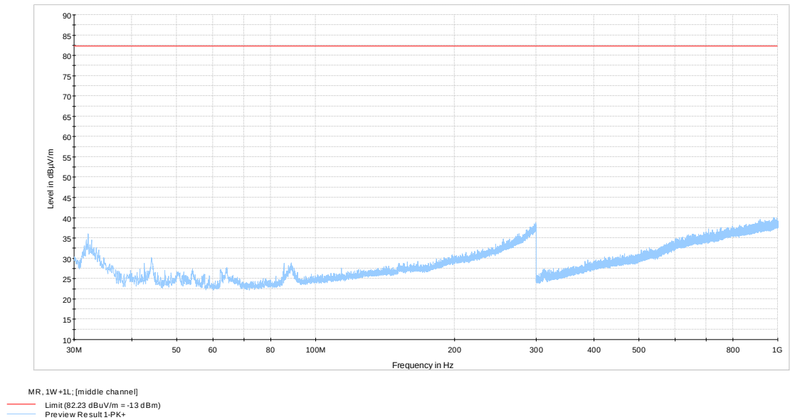
Figure 8.1-16: 30 to 1000 MHz – LTE+WCDMA Multi RAT, 1W+1L, Middle Channel
