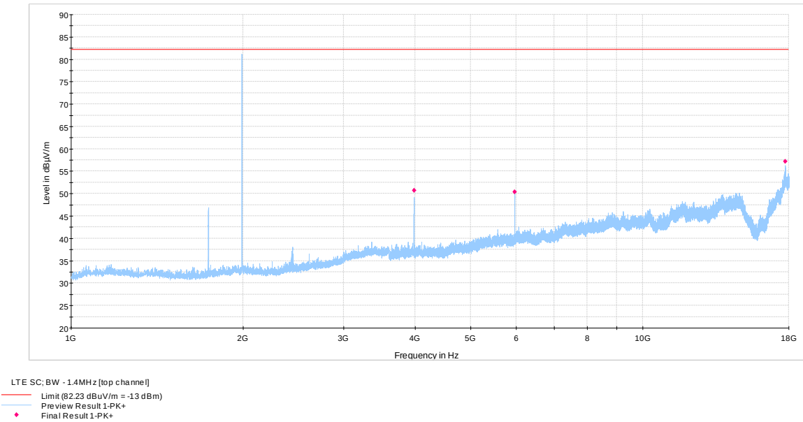
Figure 8.1-8: 1 to 18 GHz – LTE, BW=1.4M, Top channel
