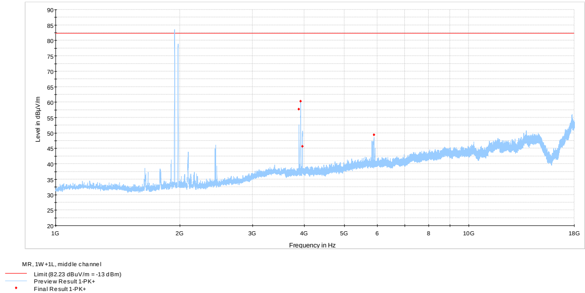
Figure 8.1-17: 1 to 18 GHz – LTE+WCDMA Multi RAT, 1W+1L, Middle Channel
