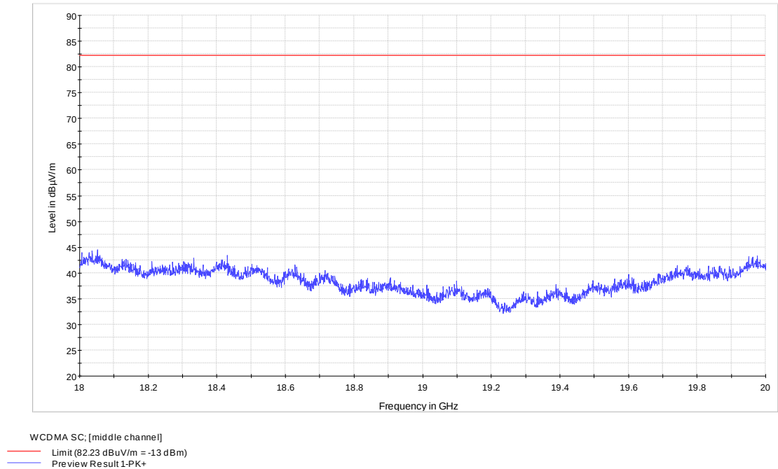
Figure 8.1-15: 18 to 20 GHz – WCDMA, 1 Carrier, Middle Channel
