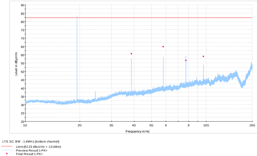
Figure 8.1-5: 1 to 18 GHz – LTE, BW=1.4M, Bottom channel
