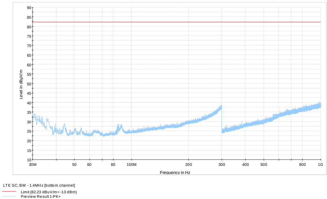
Figure 8.1-4: 30 to 1000 MHz – LTE, BW=1.4M, Bottom channel
