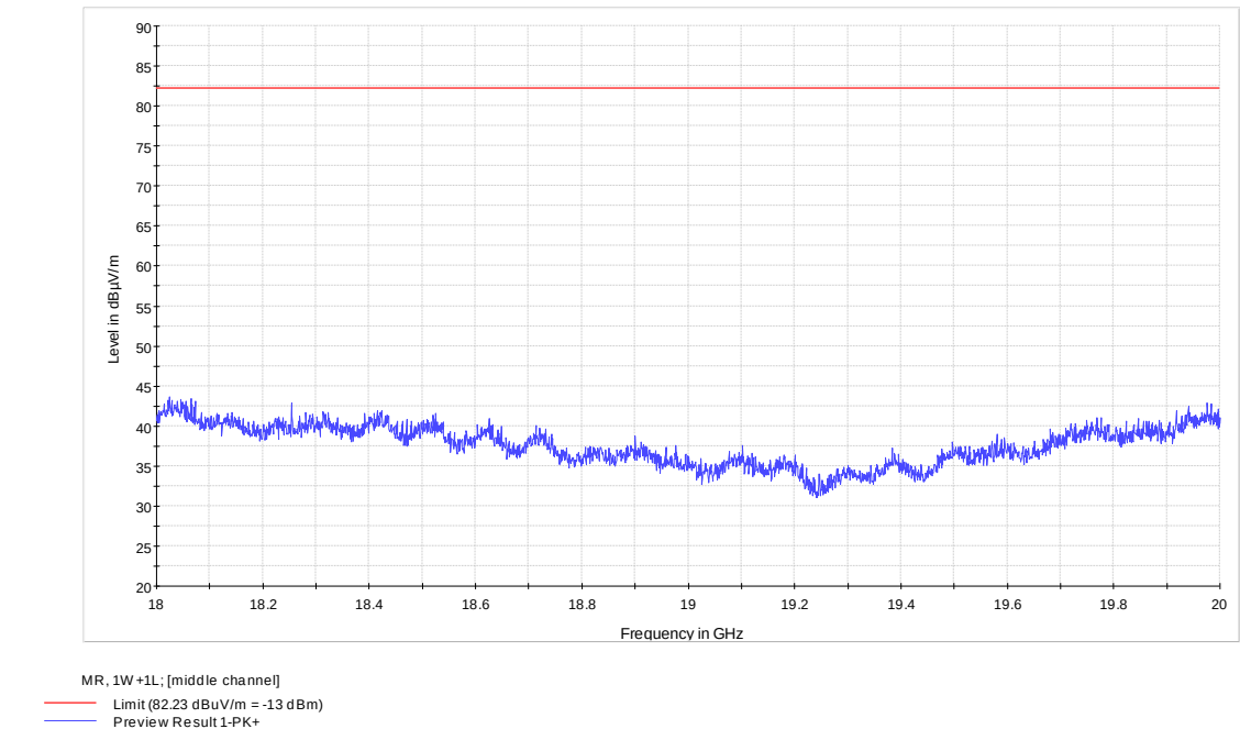
Figure 8.1-18: 18 to 20 GHz – LTE+WCDMA Multi RAT, 1W+1L, Middle Channel
