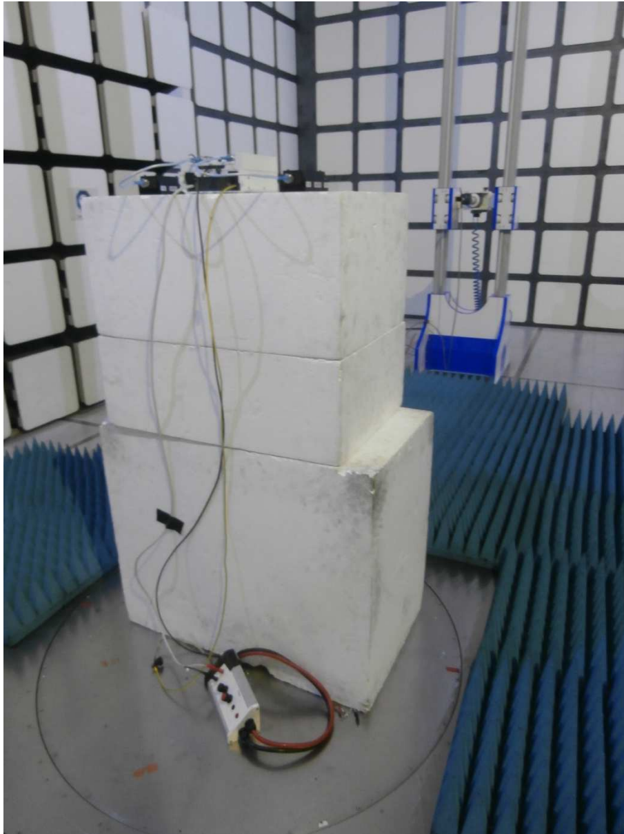
Radiated Emissions 18 GHz to 20 GHz
