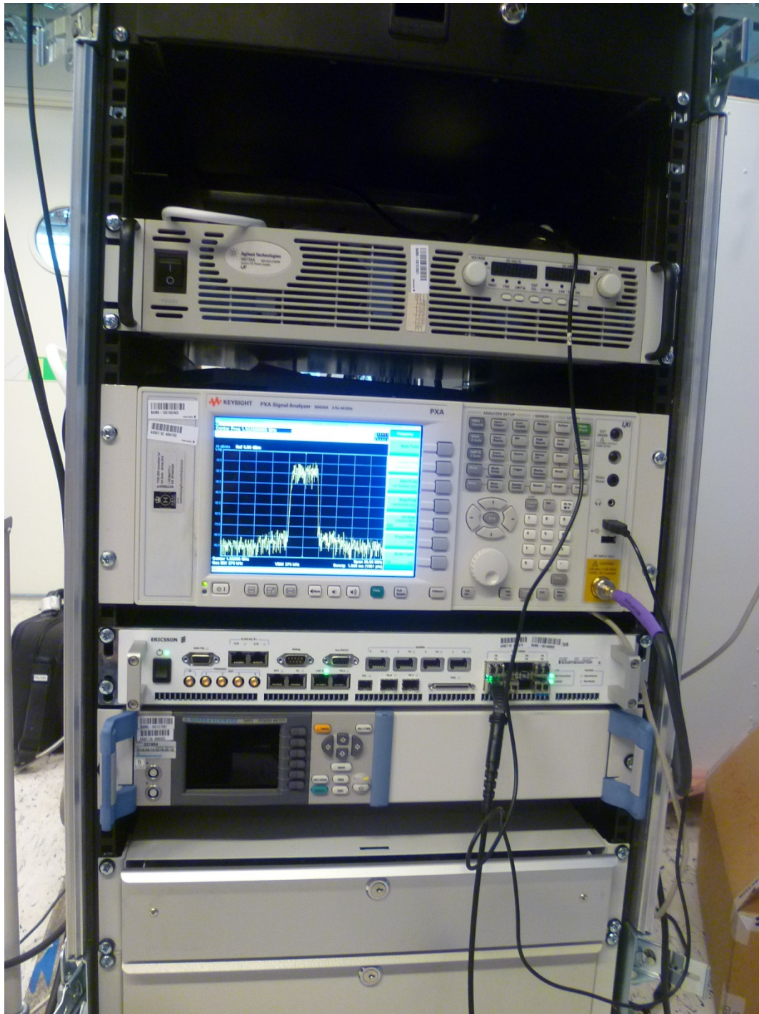
Measurement equipment set up – close up
