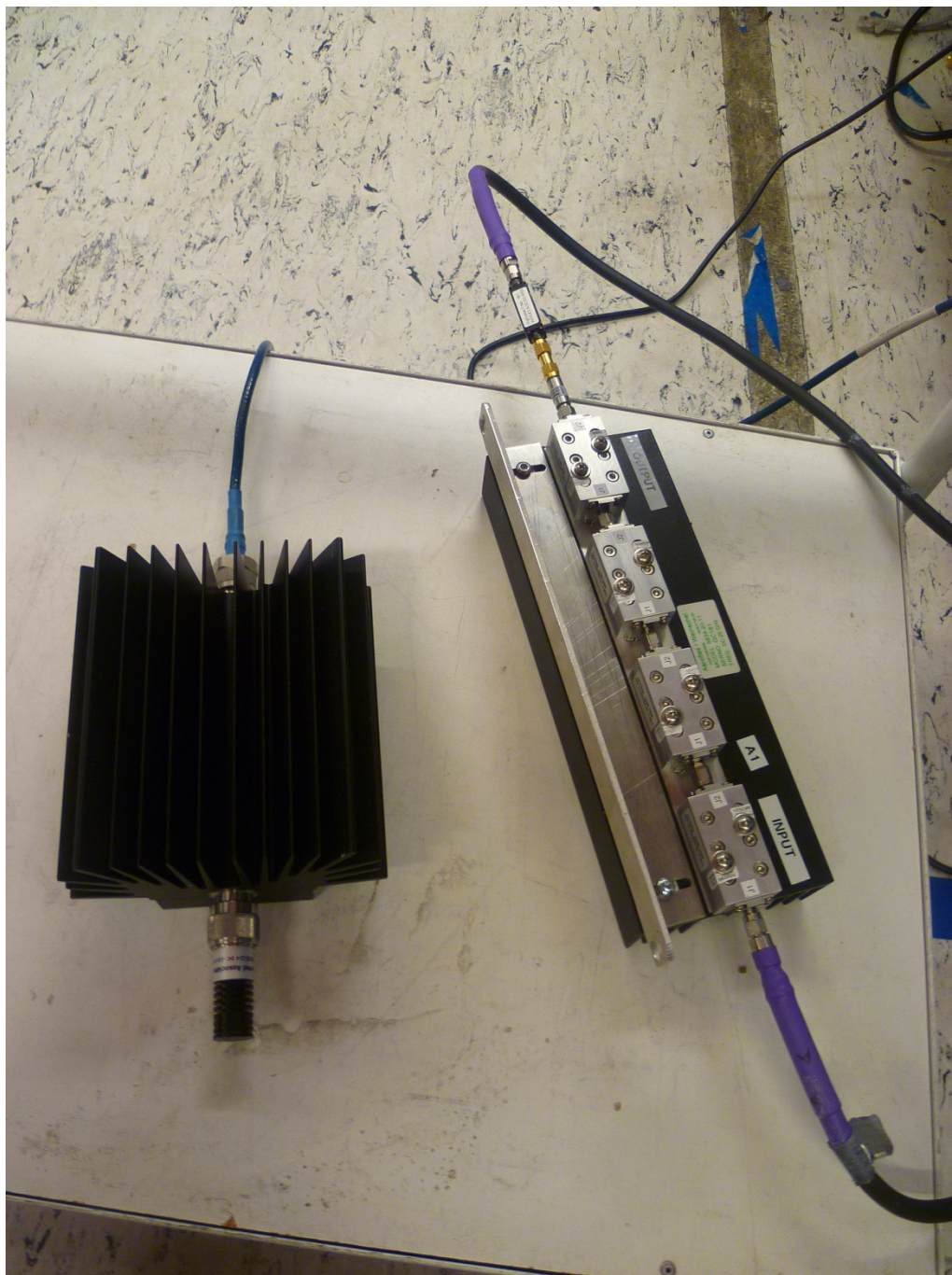
Attenuators and RF load
