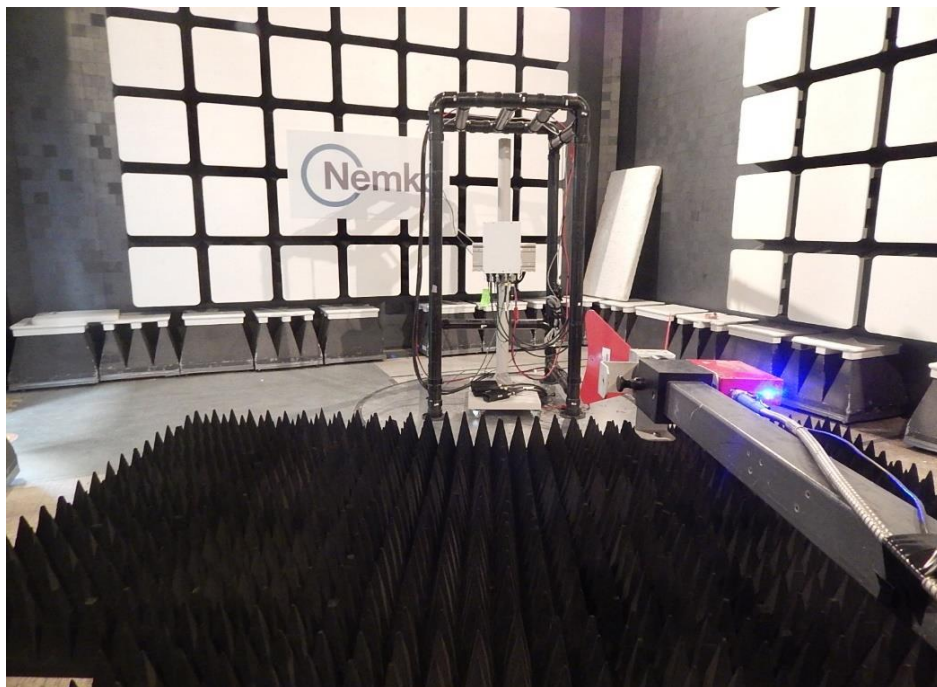
Figure-4: EUT Set-up photos for Radiated Emissions from 1-18 GHz
