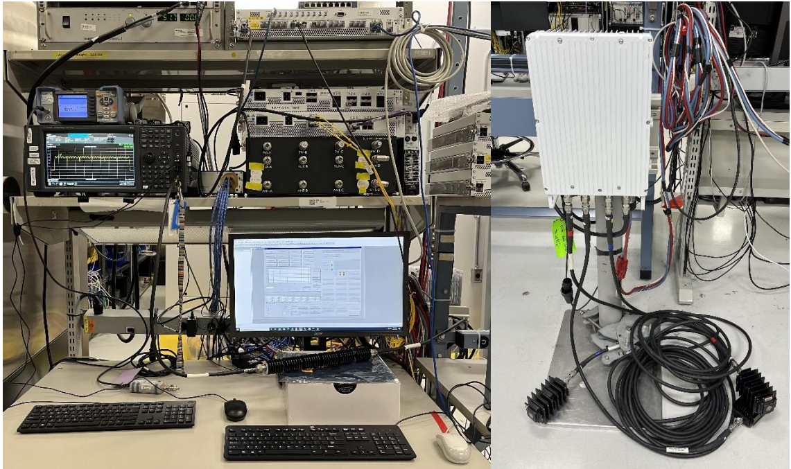
Figure-1: Set up photo for Radio Compliance Testing
