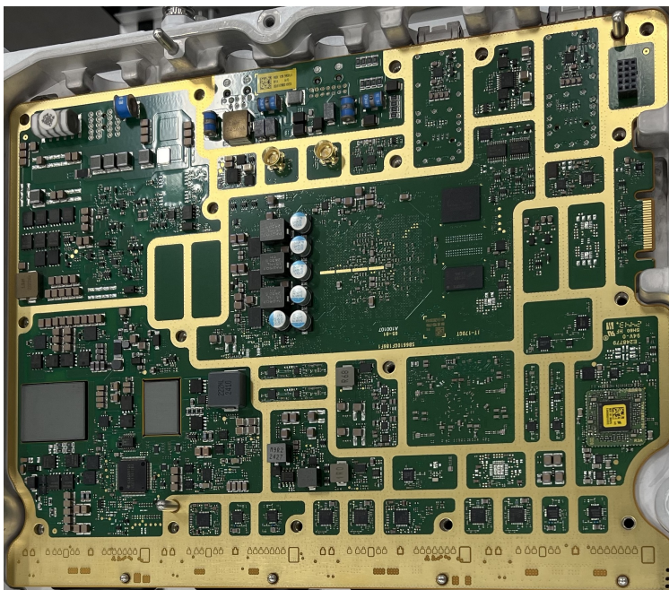
Figure 2: Radio 4461 B77D Radio Board (ROA 128 9931/77) Primary Side – TVK 128 3670
