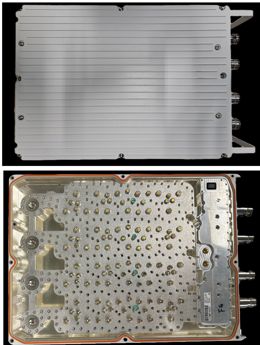
Figure 5: Radio 4461 B77D RF Radio Filter Assembly KRF 901 765
