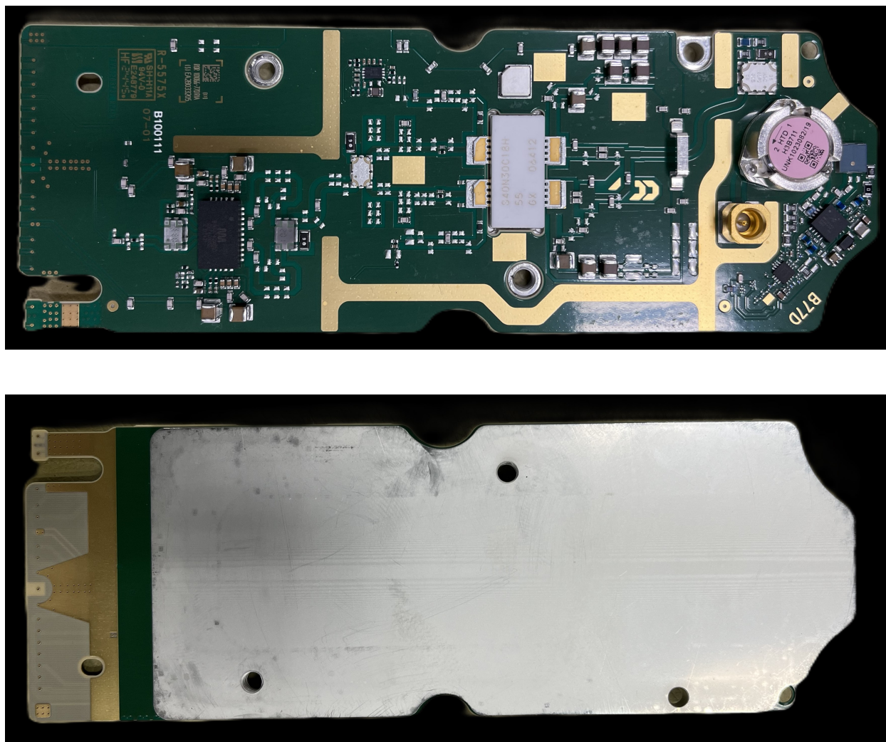
Figure 4: Radio 4461 B77D PA Board ROR 101 066/77D – TVK 128 3737
