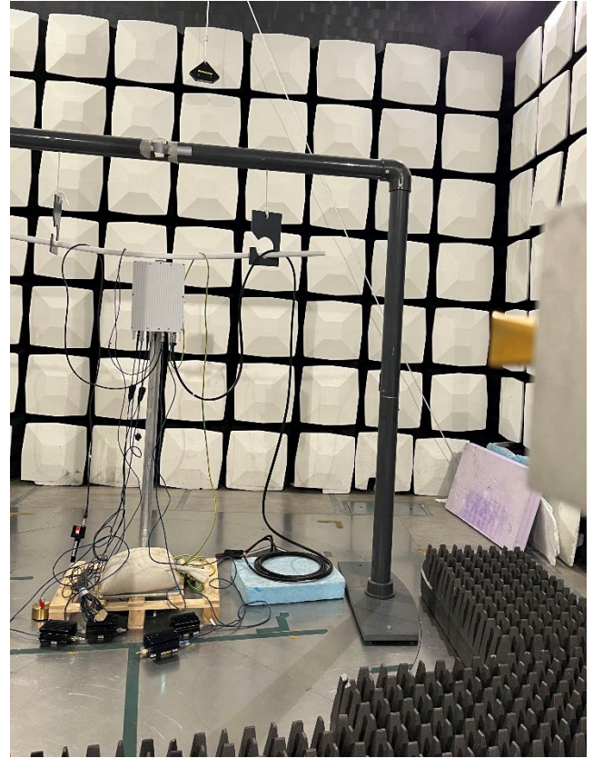
Photo of the test setup above 1 GHz
