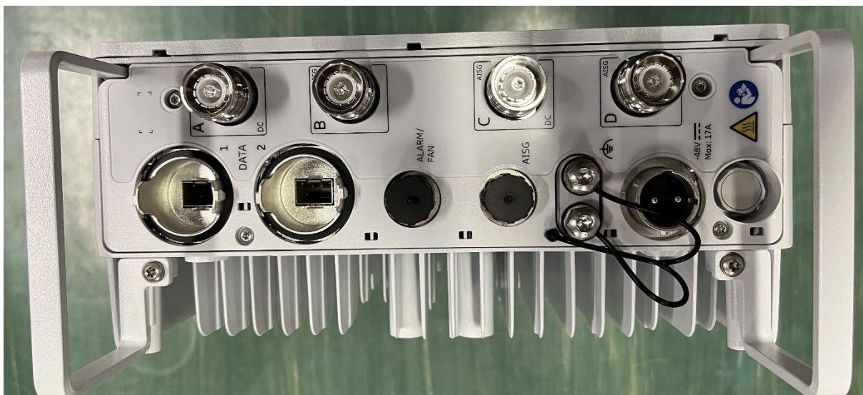
Figure 3: Radio 4471HP B66 Bottom View
