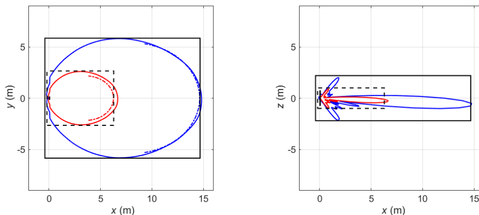
Figure 2 Compliance boundary for general public exposure (black solid line) and occupational exposure (black dashed line) for the markets where the FCC limits apply. The blue solid and dash-dotted lines correspond to compliance distance results for general public exposure obtained using the spherical and cylindrical models, respectively. The red solid and dash-dotted lines correspond to compliance distance results for occupational exposure obtained using the spherical and cylindrical models, respectively. The antenna is shown from the above (left) and from the side (right) with its back plane located at x = 0 m. Mode: B2 (LTE/NR/NB-IoT) and B25 (LTE/NR/NB-IoT). Total time-averaged power delivered to the antenna: 53.9 dBm / 245.6 W.
