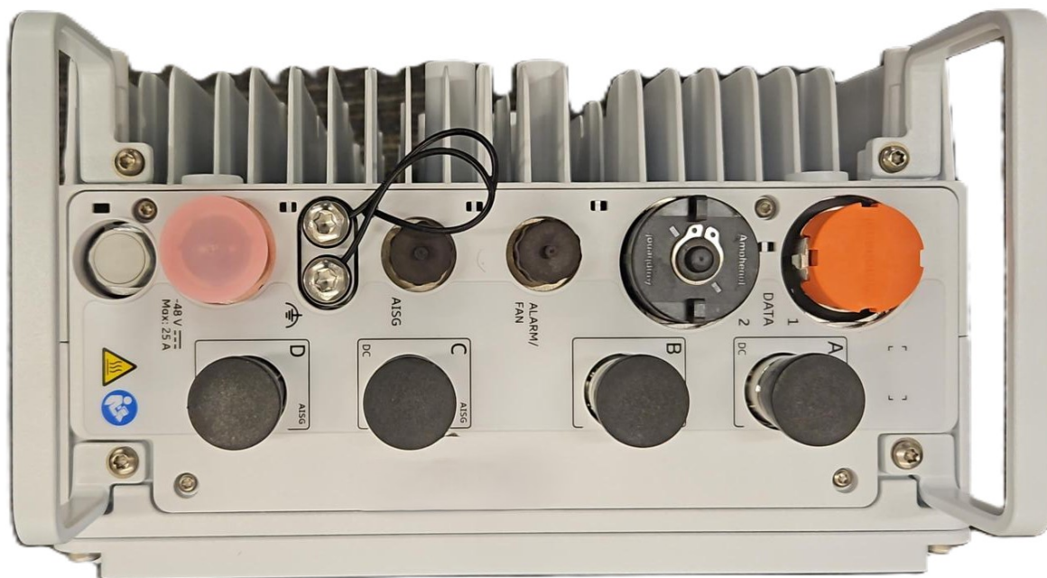
Figure 1: Radio 4472HP B5 Bottom / Connector / Handle View
