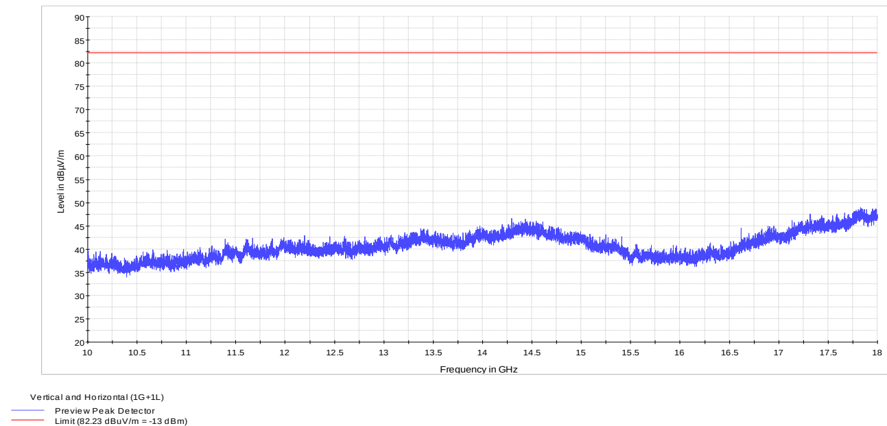
Figure 8.1-3: 10 to 18 GHz – 1G + 1L
