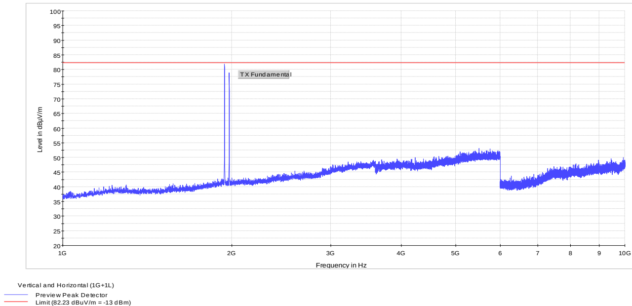
Figure 8.1-2: 1 to 10 GHz – 1G + 1L
