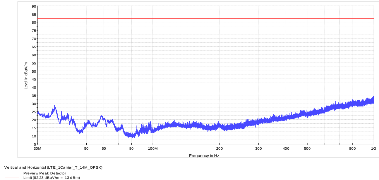
Figure 8.1-25: 30 to 1000 MHz – LTE_1Carrier_T_14M_QPSK
