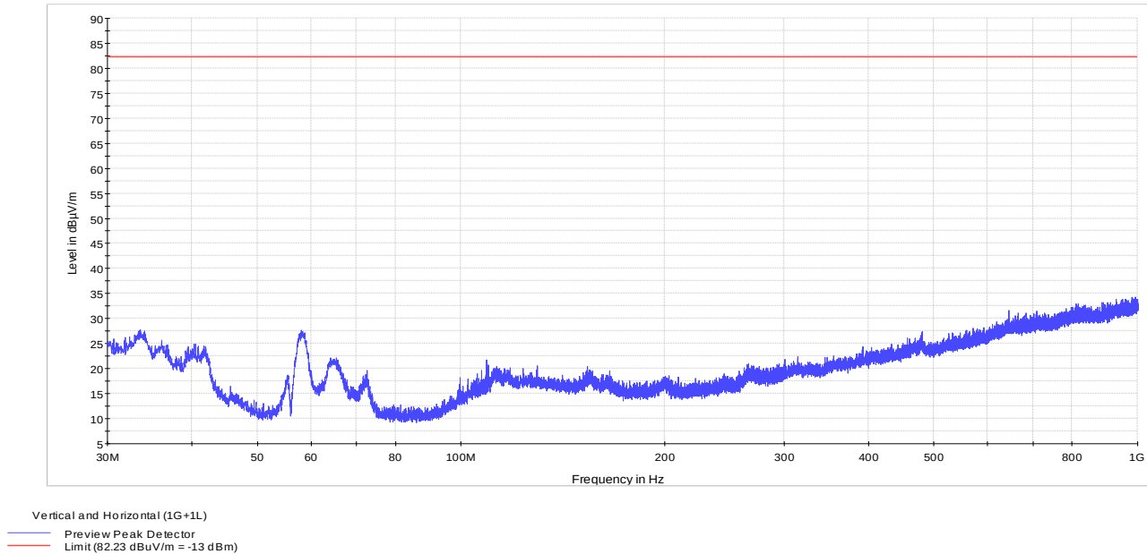
Figure 8.1-1: 30 to 1000 MHz – 1G + 1L
