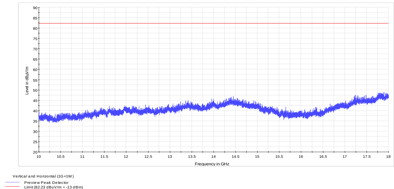
Figure 8.1-7: 10 to 18 GHz – 1G + 1W
