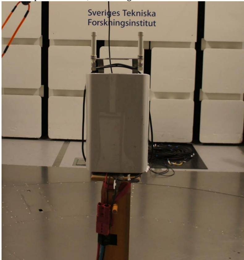
Test setup orientation 1, Semi-integrated omni antenna:
