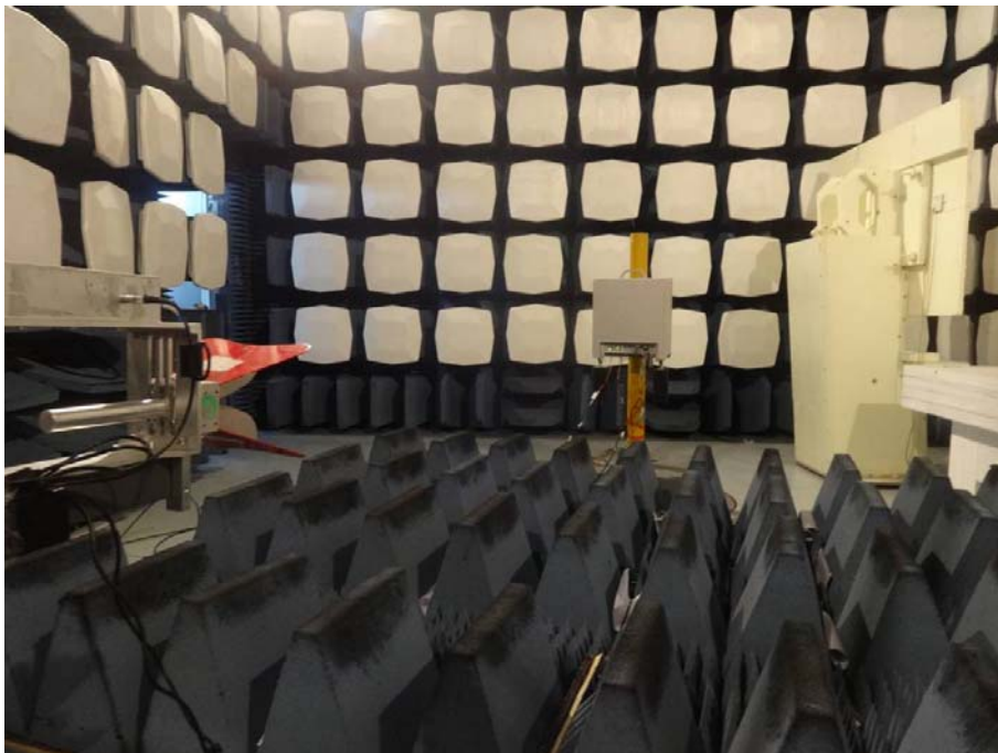
Radiated Spurious Emissions (1GHz – 18GHz)
