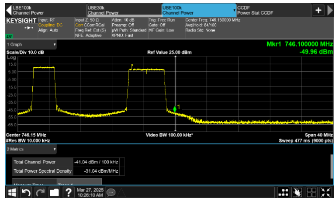
Figure 8.4-162: Conducted emission 100 kHz away from the upper band edge
