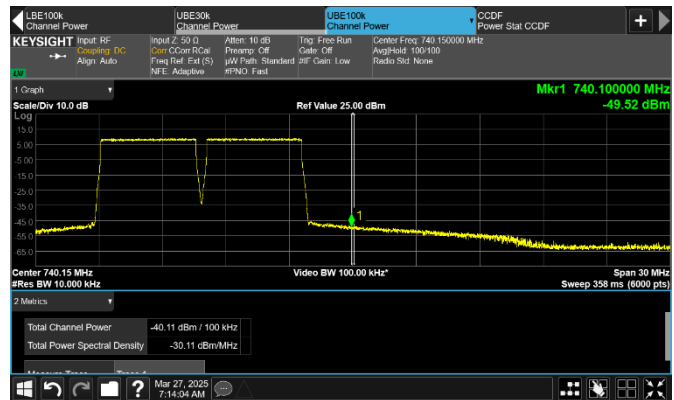
Figure 8.4-138: Conducted emission 100 kHz away from the upper frequency block edge of low channel
