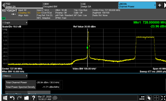
Figure 8.4-163: Conducted emission at the lower band edge
