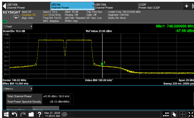
Figure 8.4-131: Conducted emission at the upper band edge
