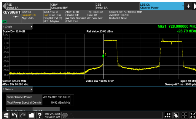
Figure 8.4-159: Conducted emission at the lower band edge
