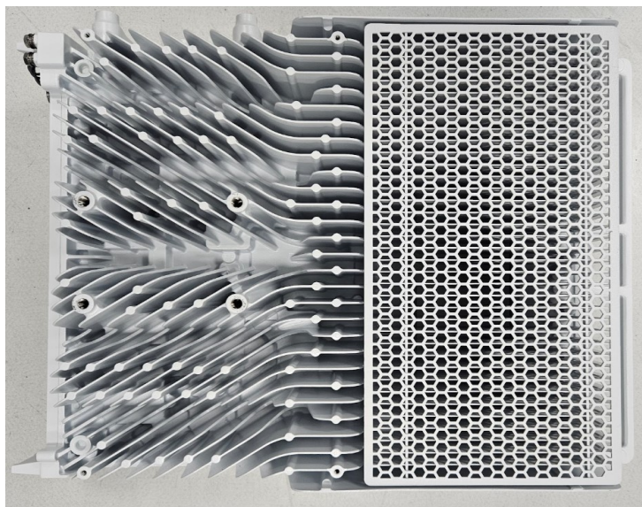
Figure 3: Radio 4495HP 44B71 44B85A C / Back / Heatsink (Mounting) View
