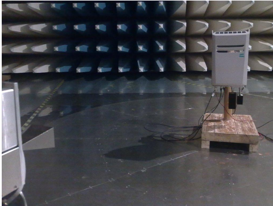
Radiated Emissions
