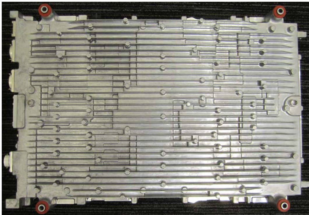
Figure 1: ARUS 32 B4 Bottom View
