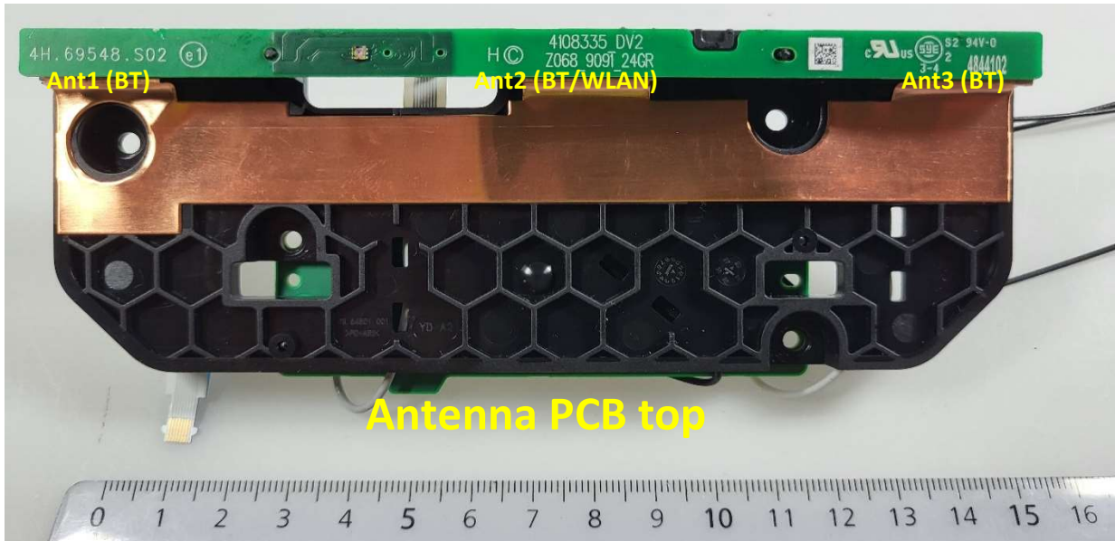
PCBA Z068 9091 Antenna top/bottom
