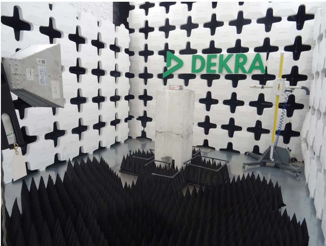
TEST SETUP FOR RADIATED MEASUREMENTS ABOVE 1 GHz
