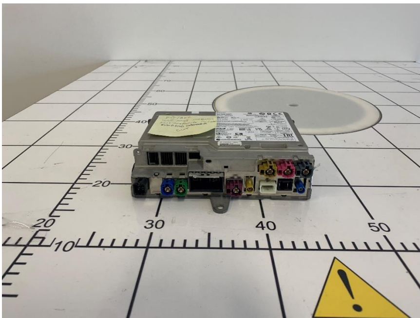
Figure B2. Rear View of DUT
