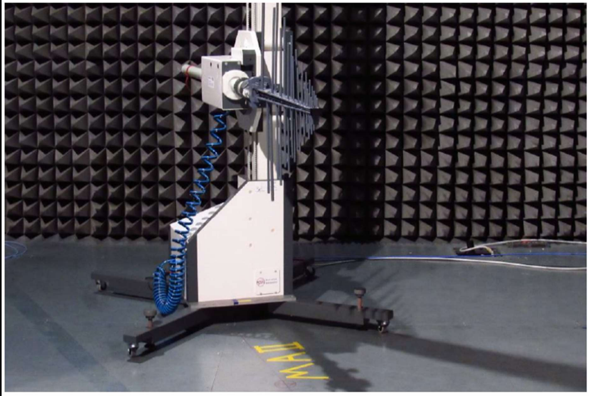
Radiated Setup - View E
