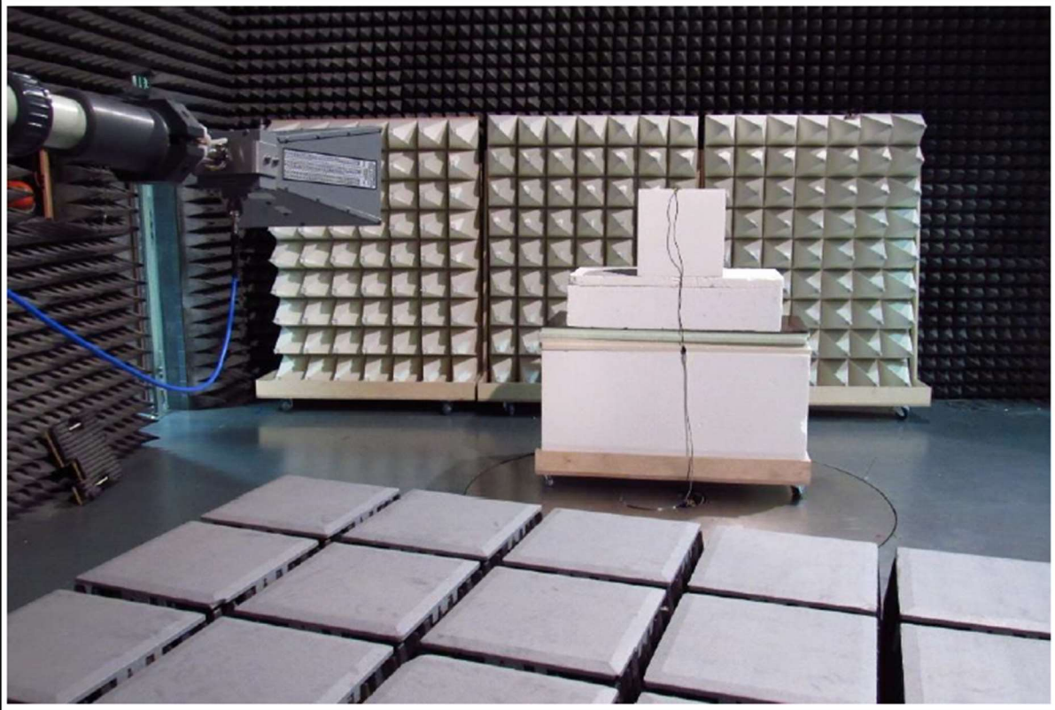
Radiated Setup - View G
