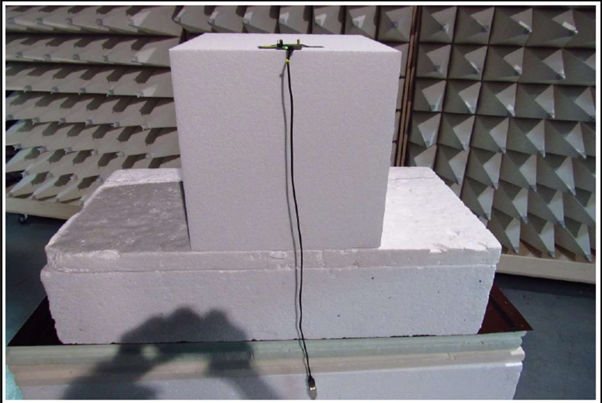
Radiated Setup - View F
