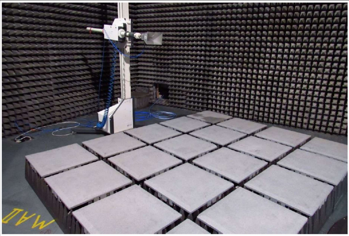
Radiated Setup - View H
