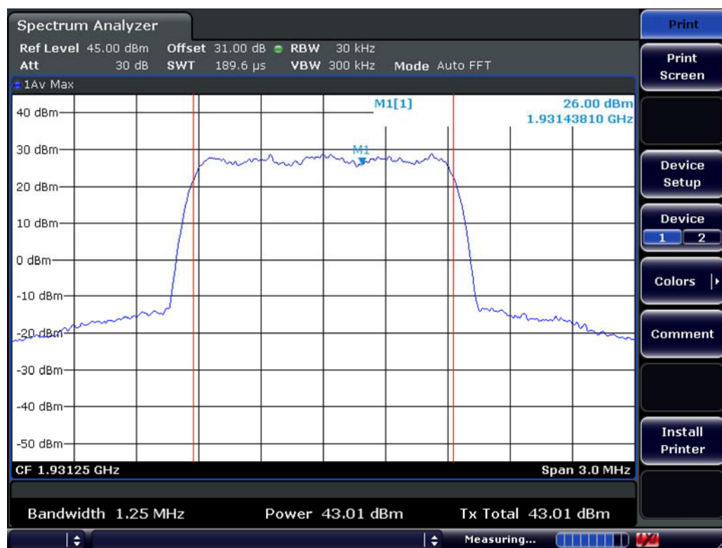
Downlink Output power (ch25)
