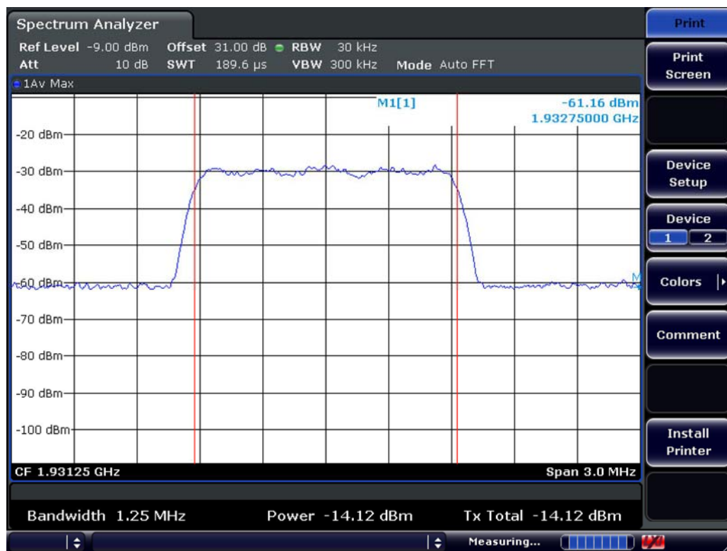
Input signal output Power (ch25)
