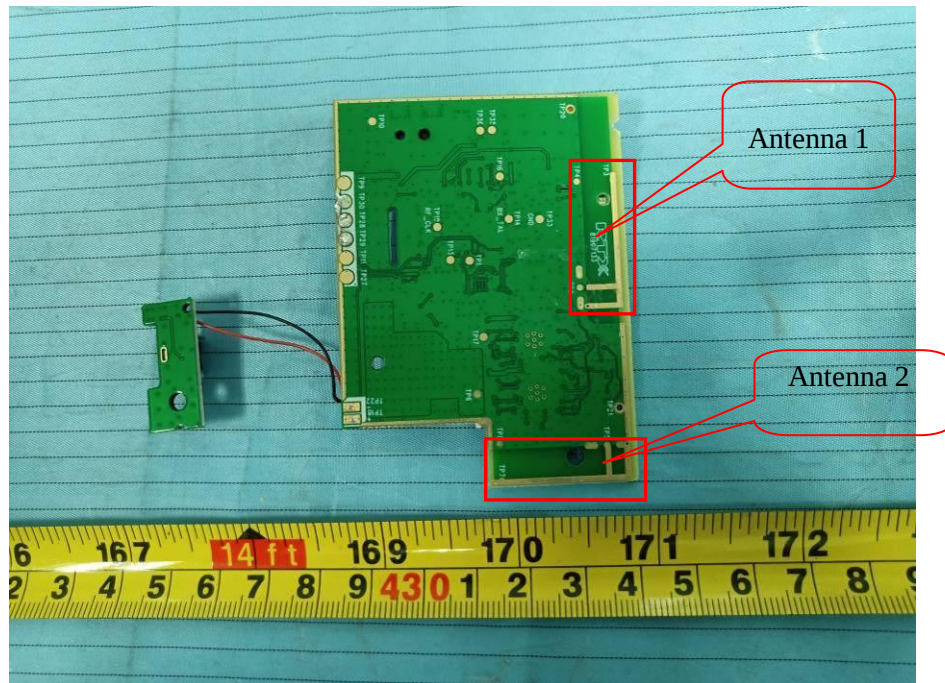
EUT – Main Board Bottom Shielding off View
