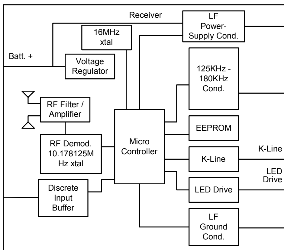
Figure 3. TPM Lowline Receiver Block Diagram
