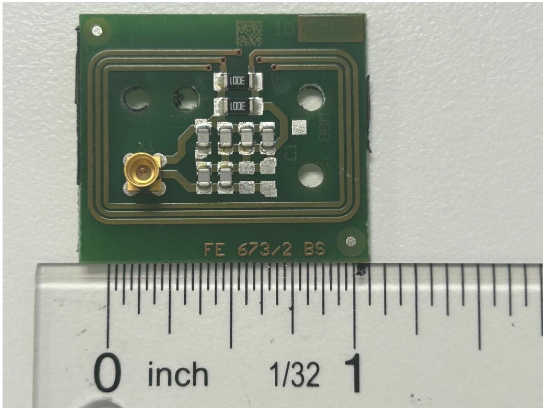
Photo 3: Antenna PCBA, no plastic, top
