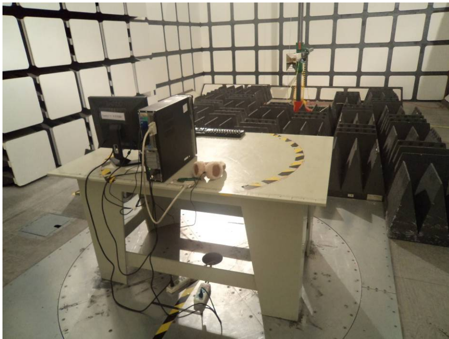
Radiated Emissions View – Rear View
