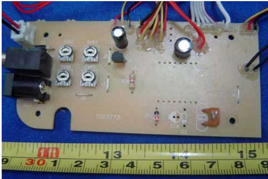
PCB(1) – Component View
