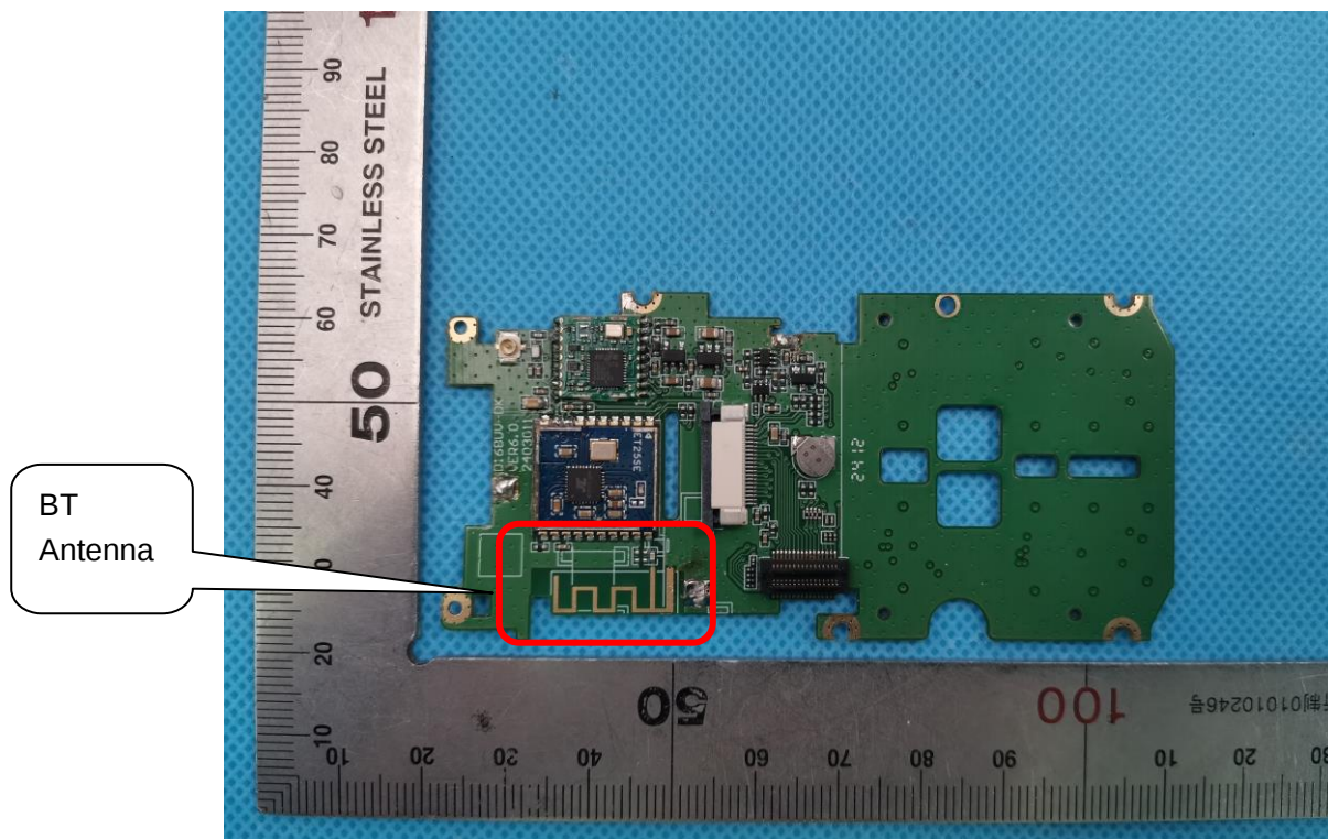
INTERNAL VIEW OF EUT (FIGURE 4)
