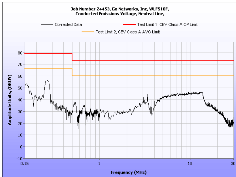
Plot 2. Conducted Emission, Neutral Line Plots
