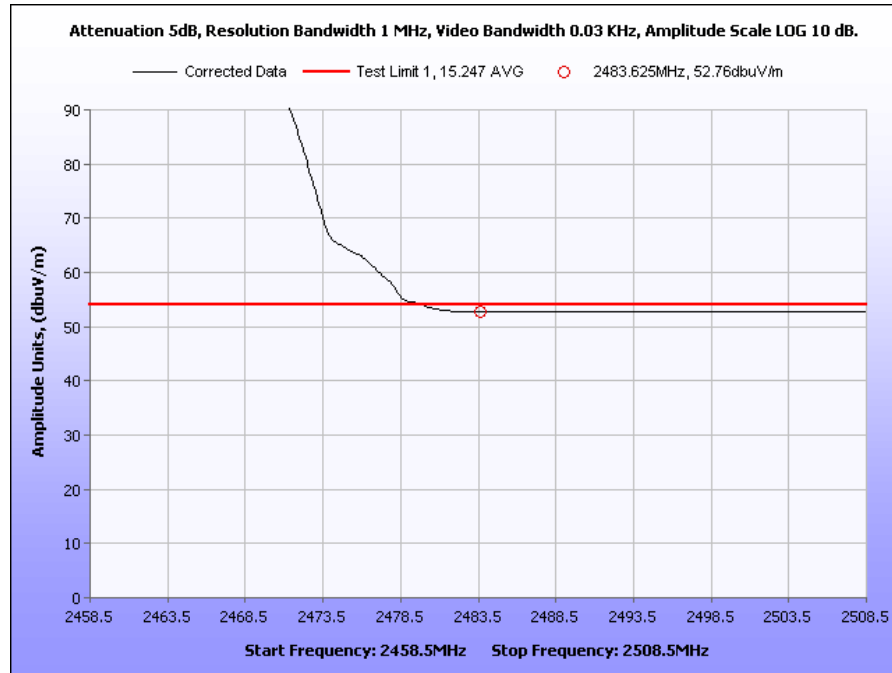
Plot 12. 802.11b Radiated Restricted Band, High Channel, Avg
