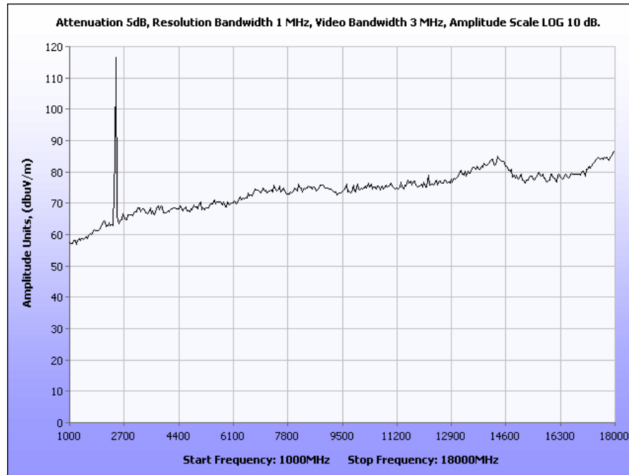
Plot 7. 802.11b Radiated Spurious, Low Channel, 1-18GHz
