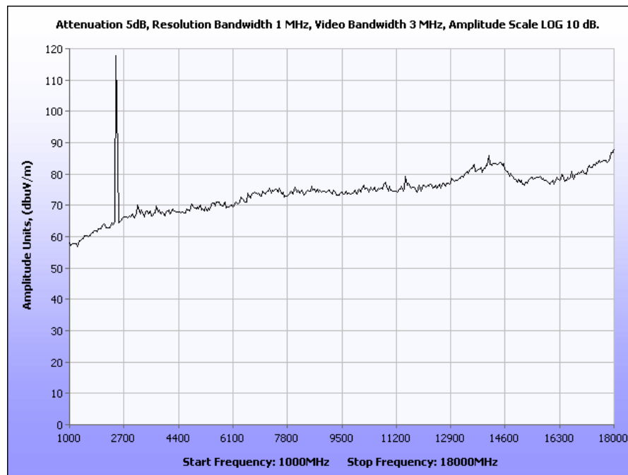
Plot 8. 802.11b Radiated Spurious, Mid Channel, 1-18GHz
