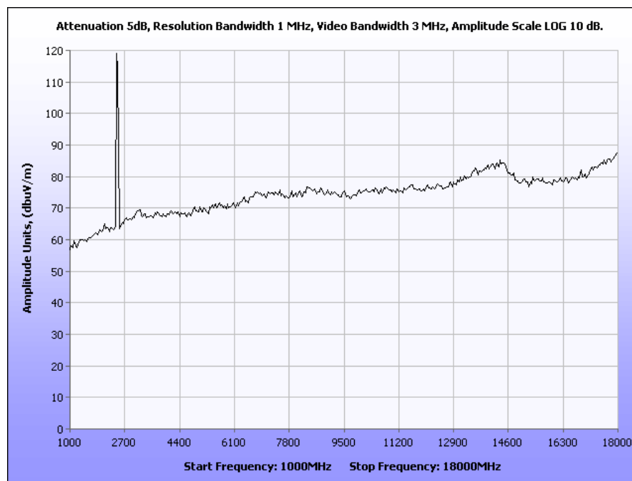
Plot 15. 802.11g Radiated Spurious, Mid Channel, 1-18GHz
