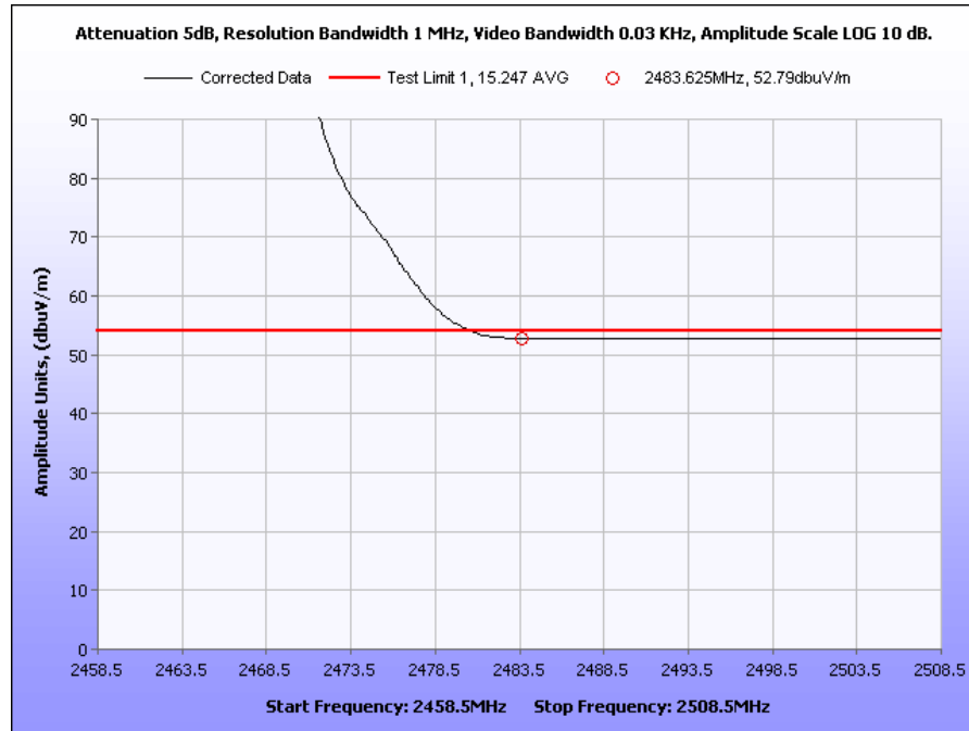
Plot 19. 802.11g Radiated Restricted Band, High Channel, Avg
