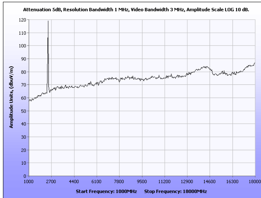
Plot 14. 802.11g Radiated Spurious, Low Channel, 1-18GHz
