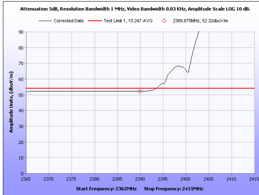
Plot 10. 802.11b Radiated Restricted Band, Low Channel, Avg
