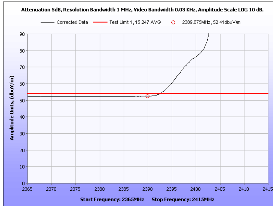
Plot 17. 802.11g Radiated Restricted Band, Low Channel, Avg
