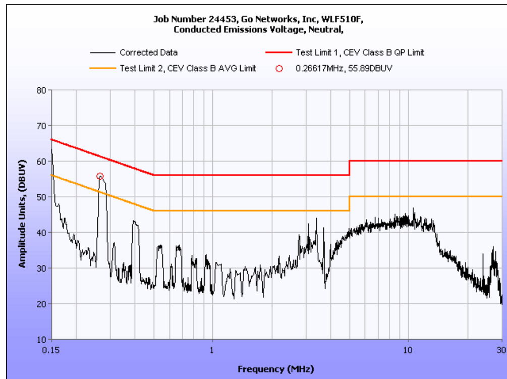
Plot 6. Conducted Emission, Neutral Line Plots
