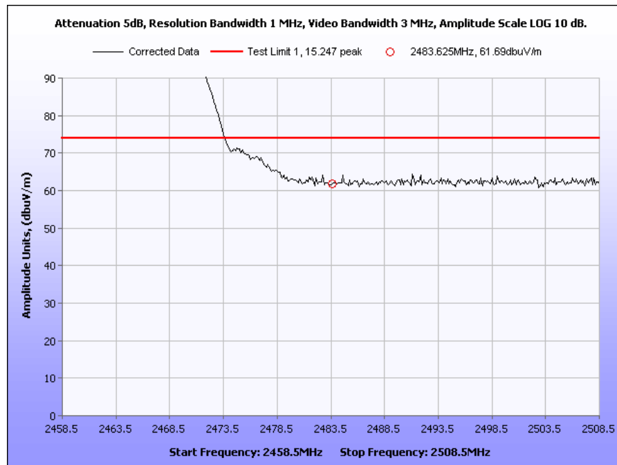
Plot 13. 802.11b Radiated Restricted Band, High Channel, Peak
