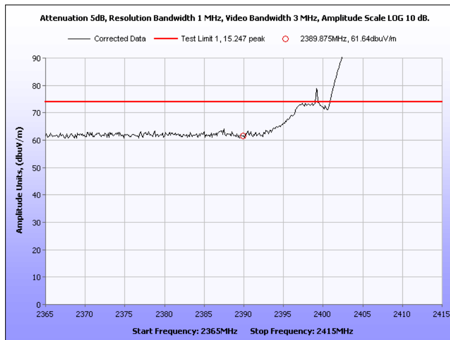
Plot 11. 802.11b Radiated Restricted Band, Low Channel, Peak
