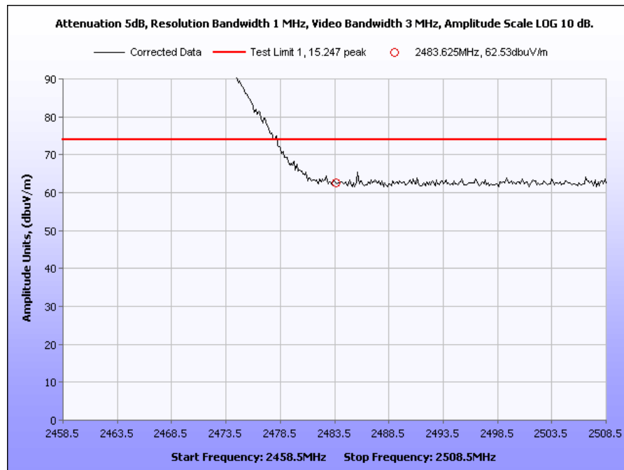
Plot 20. 802.11g Radiated Restricted Band, High Channel, Peak
