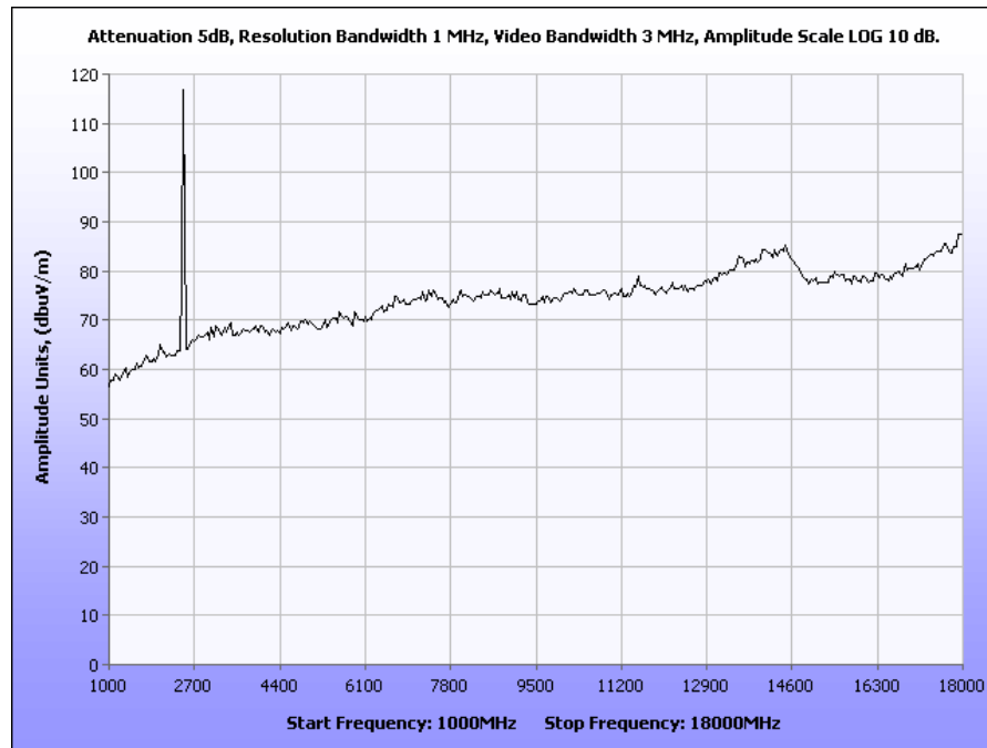
Plot 9. 802.11b Radiated Spurious, High Channel, 1-18GHz
