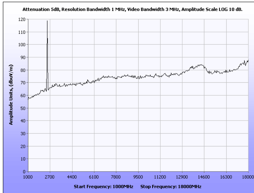
Plot 16. 802.11g Radiated Spurious, High Channel, 1-18GHz
