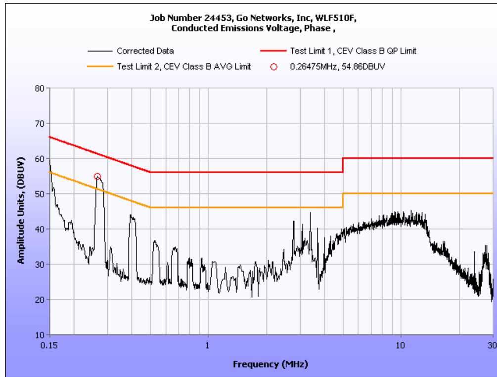
Plot 5. Conducted Emission, Phase Line Plots
