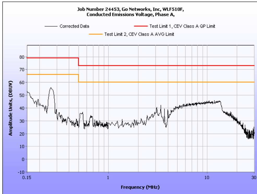
Plot 1. Conducted Emission, Phase Line Plots
