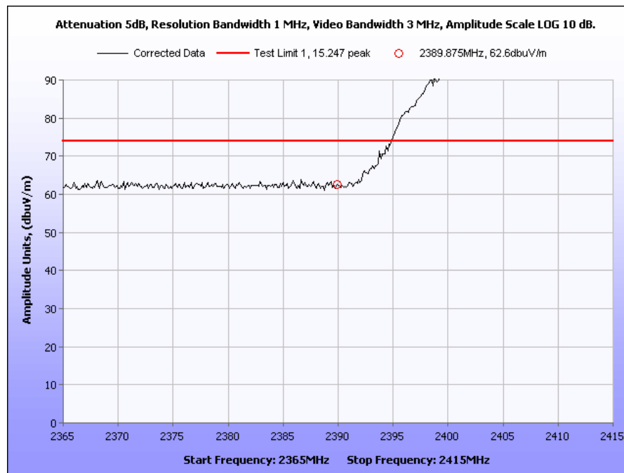
Plot 18. 802.11g Radiated Restricted Band, Low Channel, Peak
