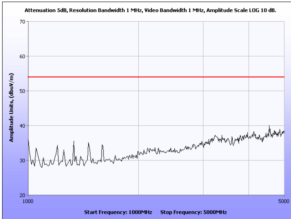
Plot 4. Radiated Emissions Limits Test Results, 1GHz – 5GHz
