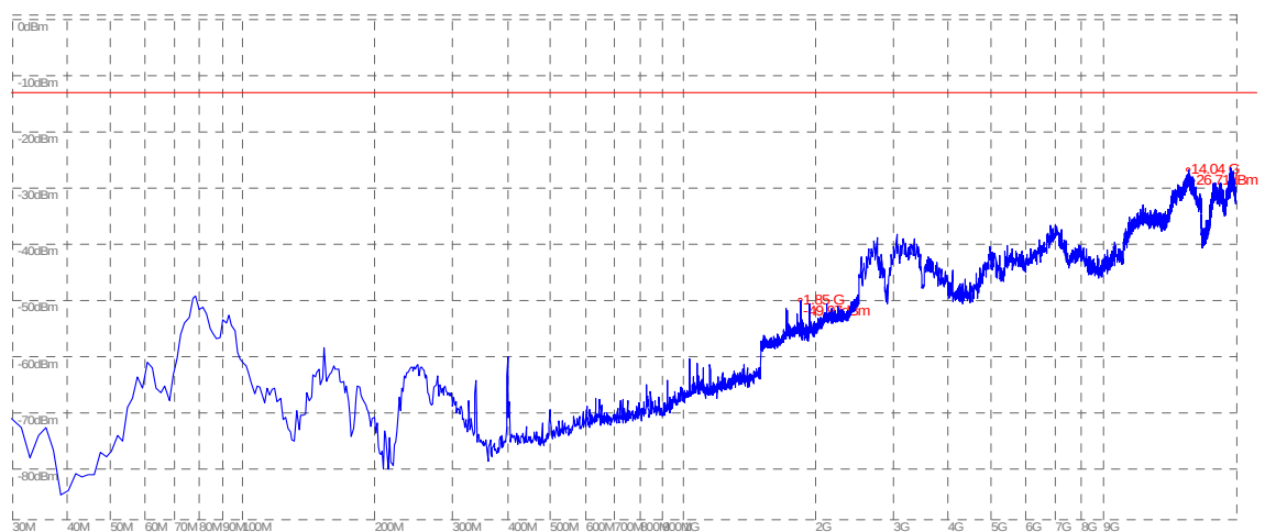
(Plot P.1: WCDMA 1900MHz Channel = 9262, Test Antenna Horizontal)
