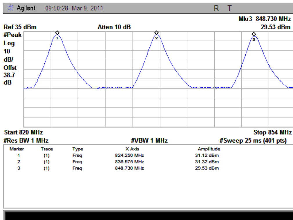
(Plot I: EDGE 850MHz Channel = 128, 190, 251)
