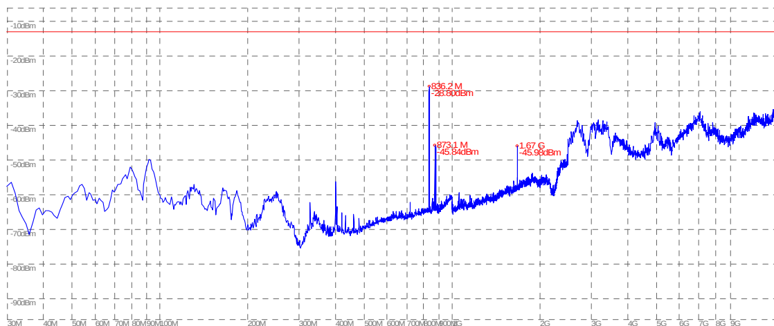
(Plot H.2: EGPRS 850MHz Channel = 190, Test Antenna Vertical)
