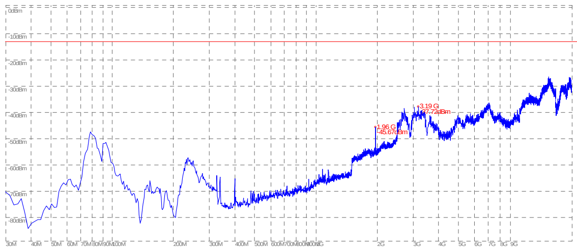
(Plot Q.1: WCDMA 1900MHz Channel = 9400, Test Antenna Horizontal)
