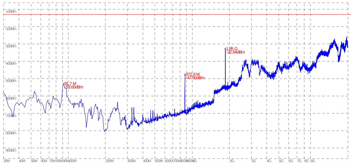
(Plot J.2: EGPRS 1900MHz Channel = 512, Test Antenna Vertical)
