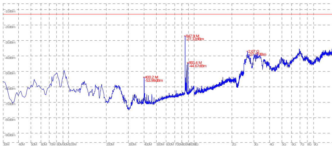
(Plot I.2: EGPRS 850MHz Channel = 251, Test Antenna Vertical)
