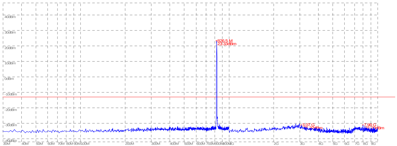
(Plot M: WCDMA 850MHz Channel = 4132, 30MHz to 10GHz)
