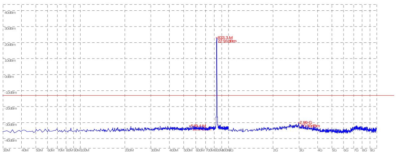
(Plot N: WCDMA 850MHz Channel = 4175, 30MHz to 10GHz)
