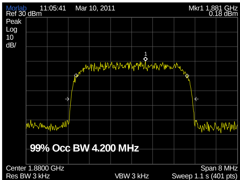
(Plot P: HSDPA 1900MHz Channel = 9400)
