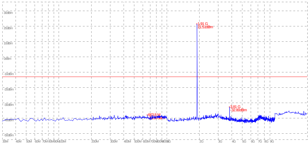
(Plot X: HSDPA 1900MHz Channel = 9538, 30MHz to 20GHz)
