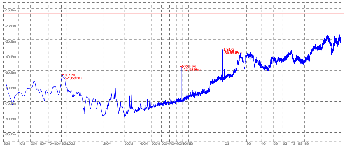
(Plot L.2: EGPRS 1900MHz Channel = 810, Test Antenna Vertical)
