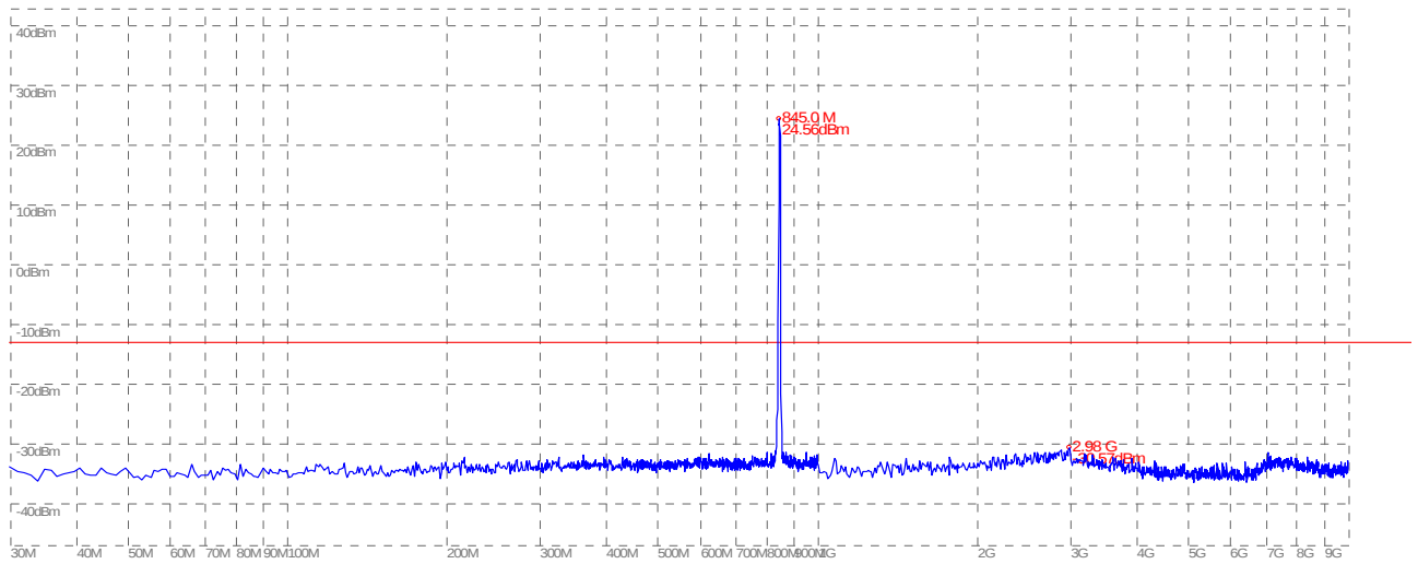
(Plot U: HSDPA 850MHz Channel = 4233, 30MHz to 10GHz)
