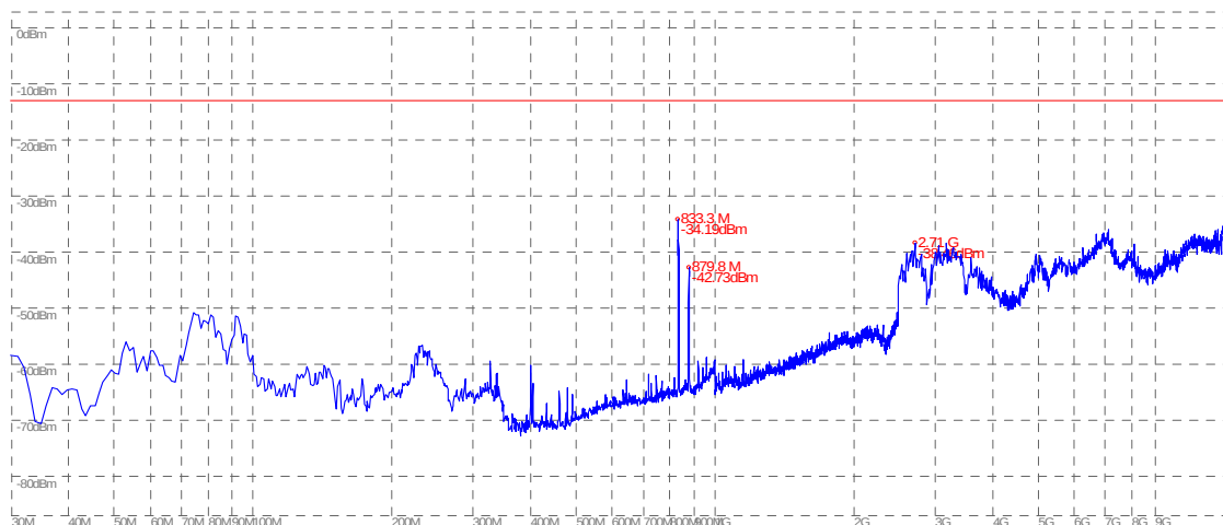
(Plot T.2: HSDPA 850MHz Channel = 4175, Test Antenna Vertical)
