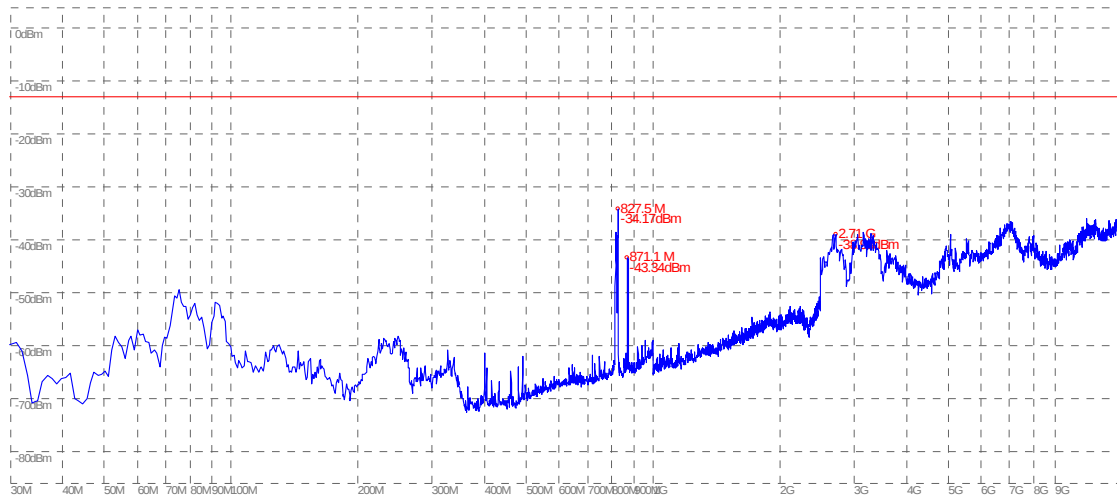
(Plot M.2: WCDMA 850MHz Channel = 4132, Test Antenna Vertical)
