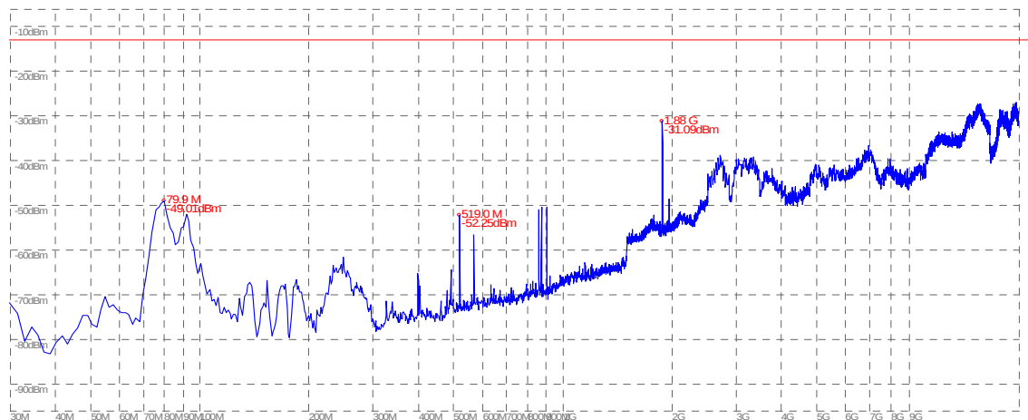
(Plot K.1: EGPRS 1900MHz Channel = 661, Test Antenna Horizontal)
