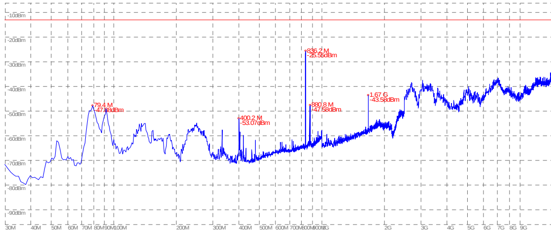
(Plot H.1: EGPRS 850MHz Channel = 190, Test Antenna Horizontal)
