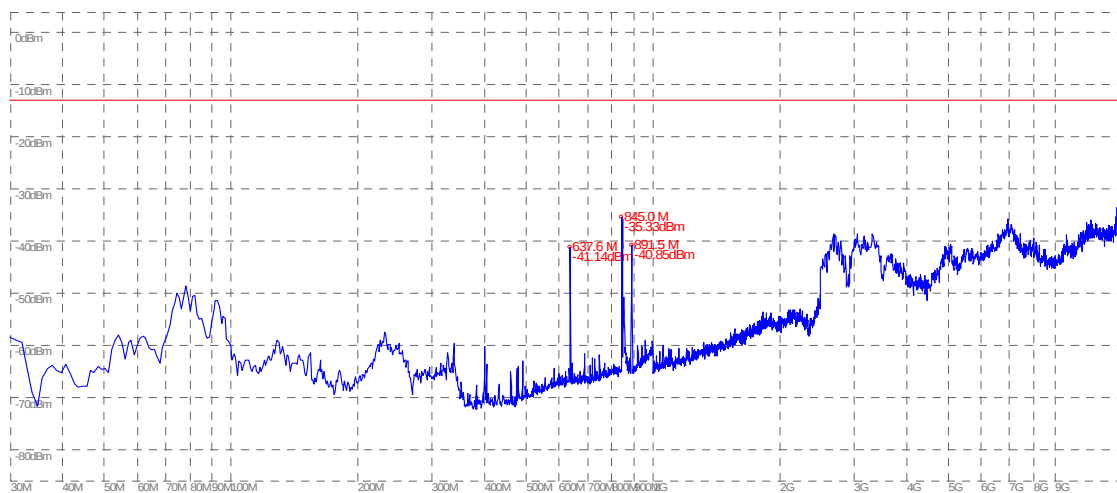
(Plot U.2: HSDPA 850MHz Channel = 4233, Test Antenna Vertical)
