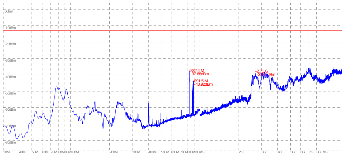
(Plot T.1: HSDPA 850MHz Channel = 4175, Test Antenna Horizontal)
