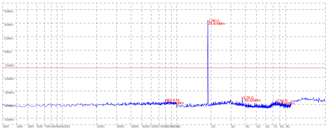
(Plot Q: WCDMA 1900MHz Channel = 9400, 30MHz to 20GHz)
