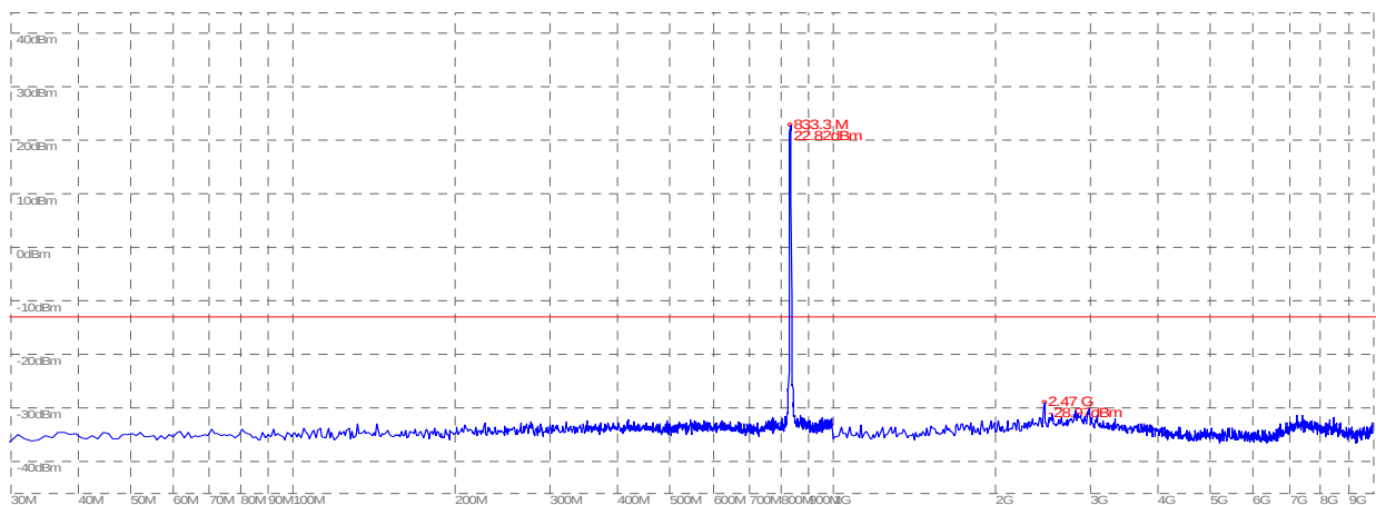
(Plot T: HSDPA 850MHz Channel = 4175, 30MHz to 10GHz)
