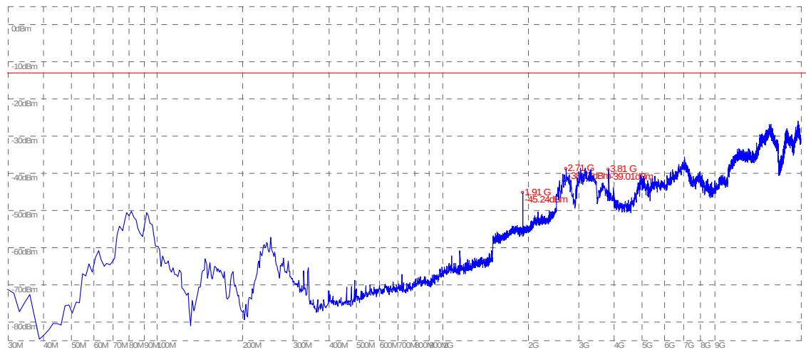
(Plot R.1: WCDMA 1900MHz Channel = 9538, Test Antenna Horizontal)
