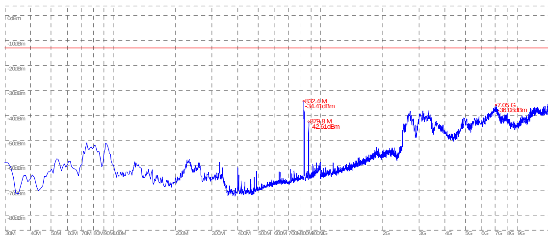
(Plot N.2: WCDMA 850MHz Channel = 4175, Test Antenna Vertical)
