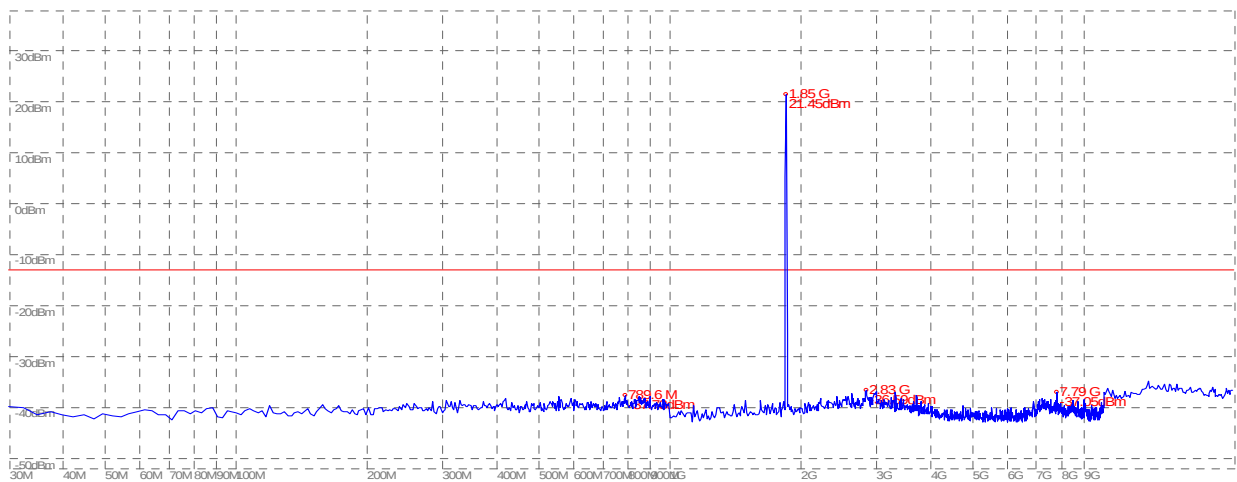
(Plot V: HSDPA 1900MHz Channel = 9262, 30MHz to 20GHz)
