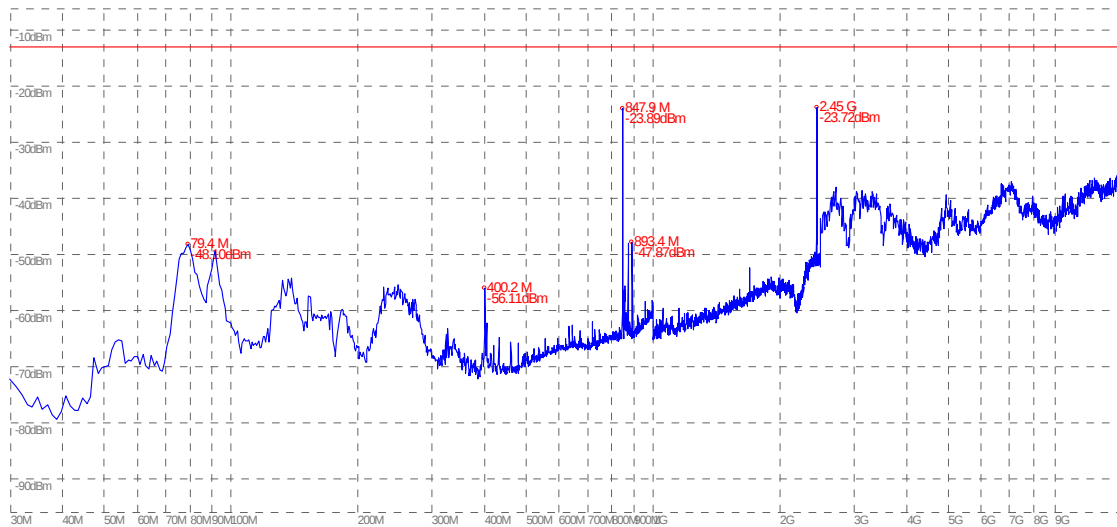
(Plot I.1: EGPRS 850MHz Channel = 251, Test Antenna Horizontal)
