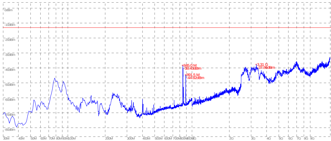
(Plot O.1: WCDMA 850MHz Channel = 4233, Test Antenna Horizontal)
