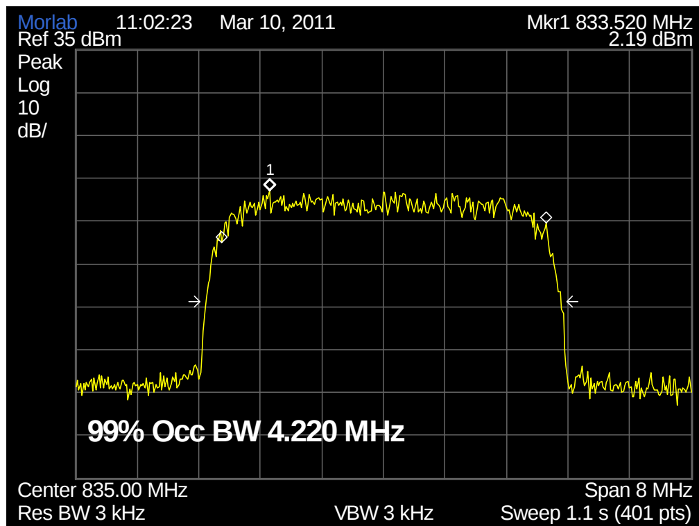
(Plot O: HSDPA 850MHz Channel = 4175)
