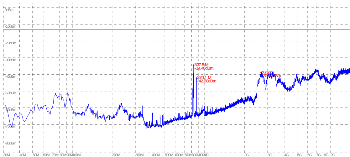
(Plot S.2: HSDPA 850MHz Channel = 4132, Test Antenna Vertical)
