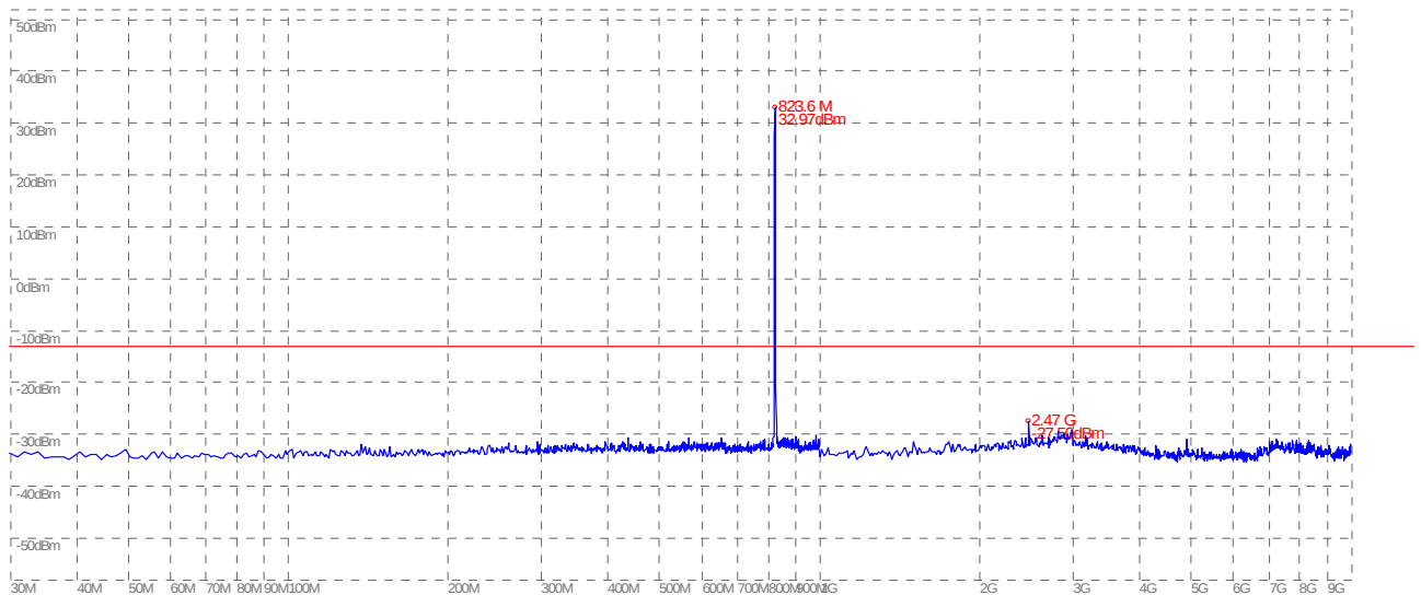
(Plot A: GSM 850MHz Channel = 128, 30MHz to 10GHz)
