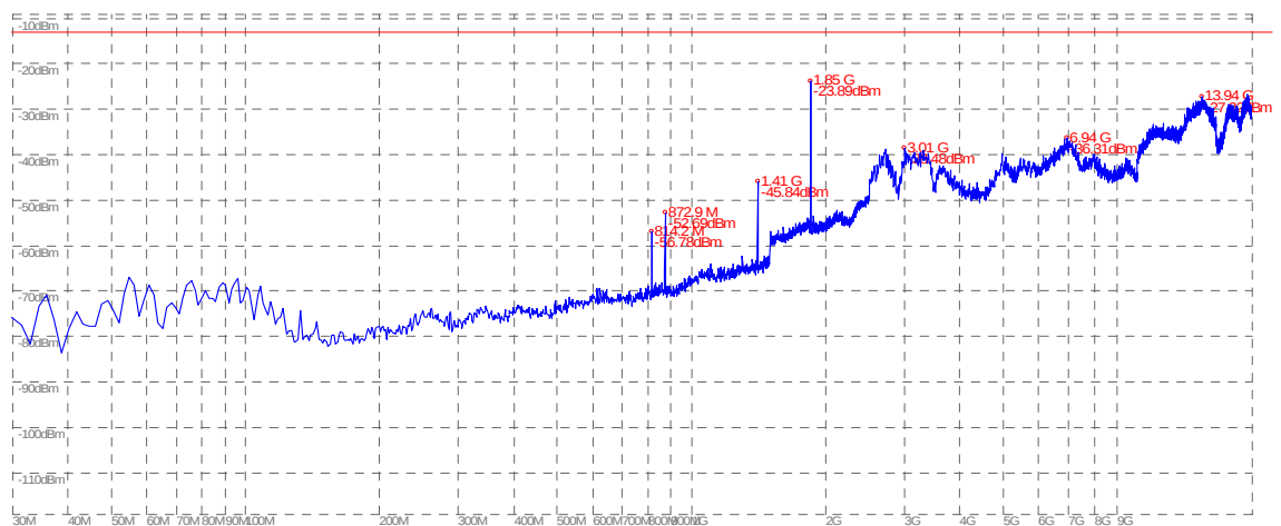
(Plot D.2: GSM 1900MHz Channel = 512, Test Antenna Vertical)
