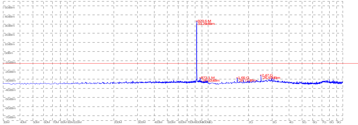
(Plot A: GSM 850MHz Channel = 128, 30MHz to 10GHz)
