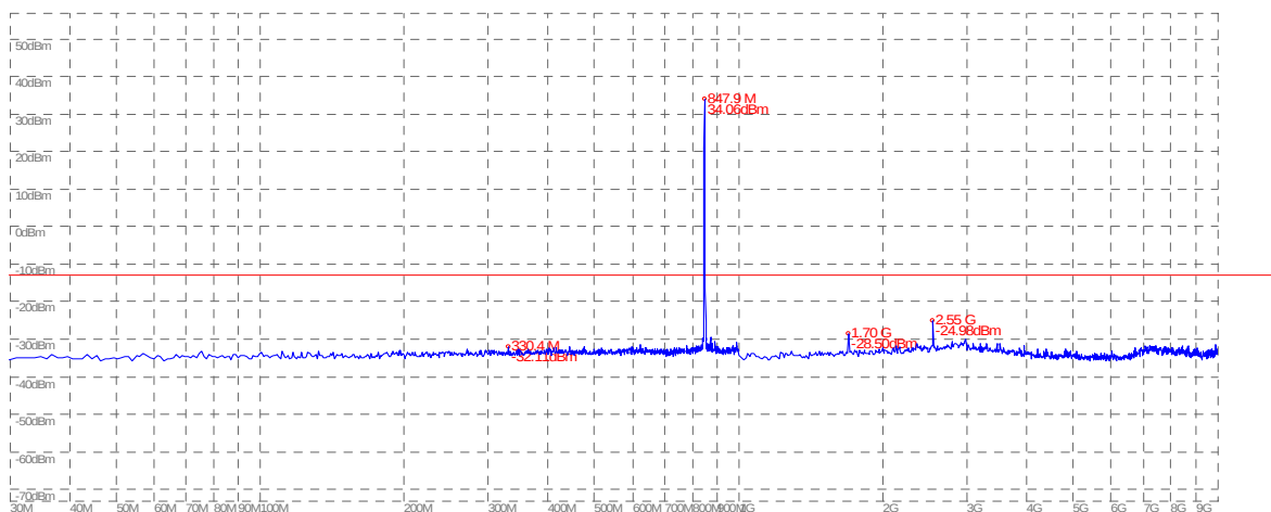
(Plot C: GSM 850MHz Channel = 251, 30MHz to 10GHz)
