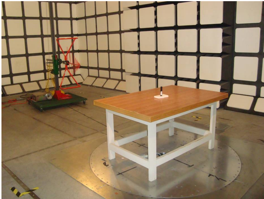
Below 1 GHz: Spurious Radiated Emissions - Rear View (Transmitting mode)
