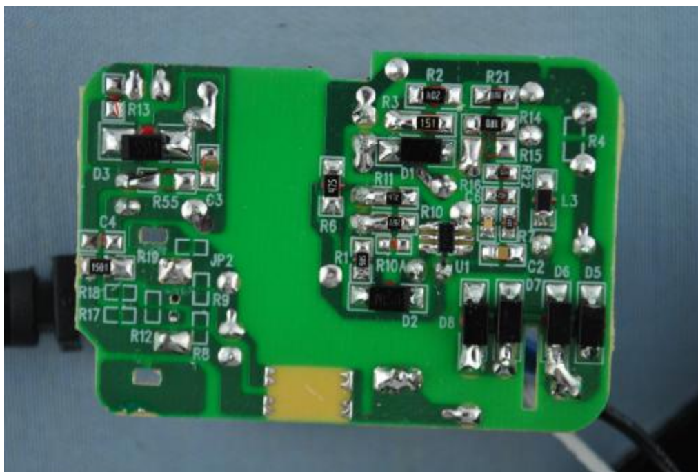
Adapter PCB rear view
