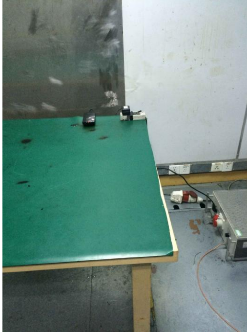
FP Conducted Emission test view
