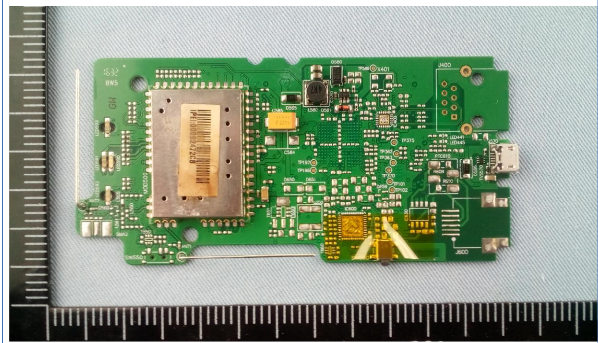
Main board component side
