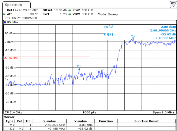
2DH1_Hopping_Lower
