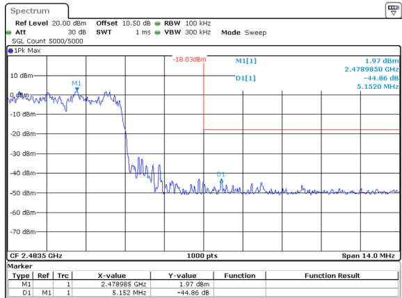
2DH1_Hopping_Upper
