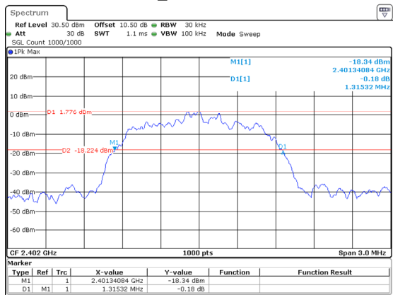
3DH1_Low 1.315MHz
