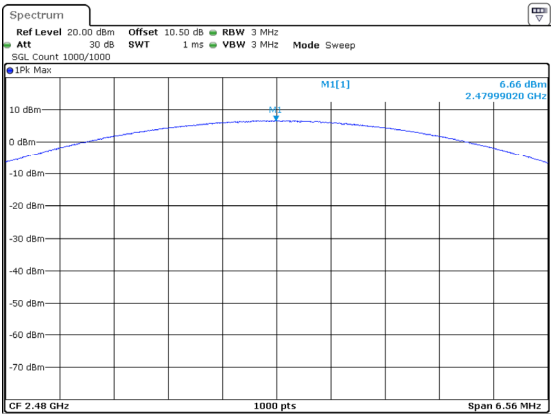
3DH1_High 6.66dBm
