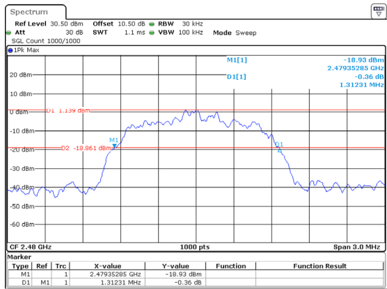
3DH1_High 1.312MHz
