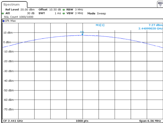
3DH1_Middle 7.27dBm
