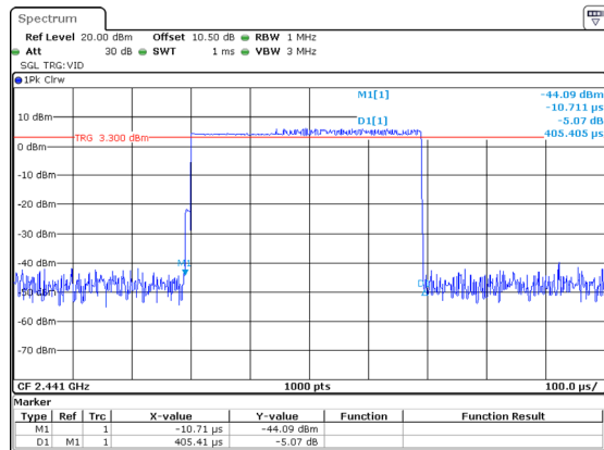
2DH1_Hopping 0.405ms
