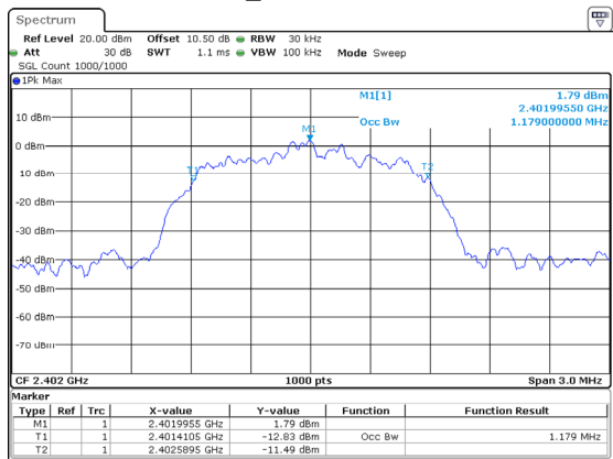
3DH1_Low 1.179MHz
