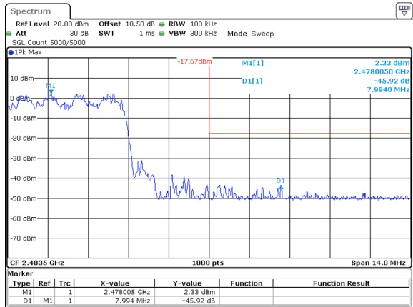
3DH1_Hopping_Upper
