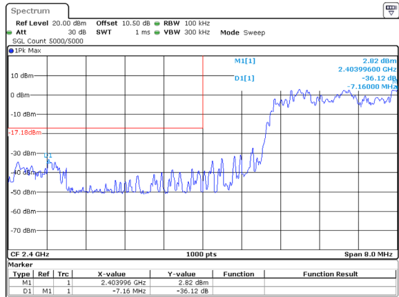
3DH1_Hopping_Lower
