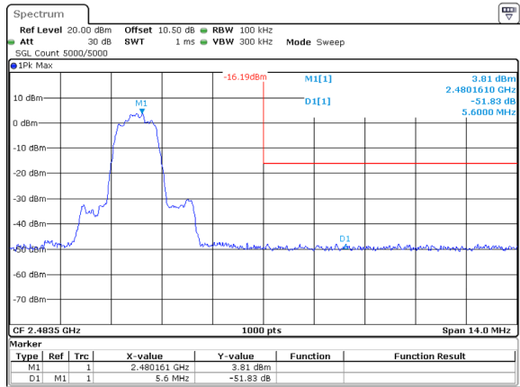
3DH1_High
