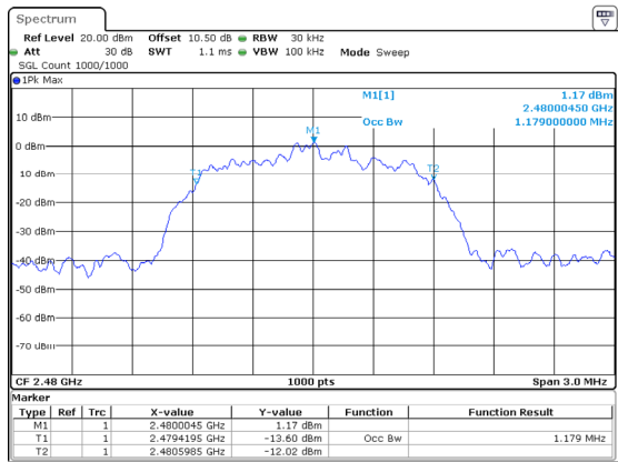
3DH1_High 1.179MHz
