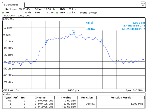
3DH1_Middle 1.182MHz
