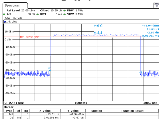
2DH5_Hopping 2.913ms
