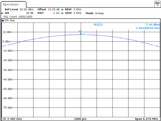
3DH1_Low 7.44dBm
