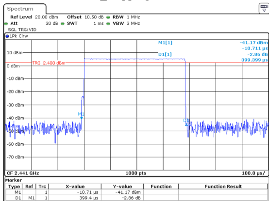
DH1_Hopping 0.399ms
