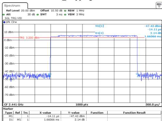
2DH3_Hopping 1.661ms
