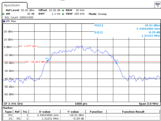
3DH1_Middle 1.312MHz
