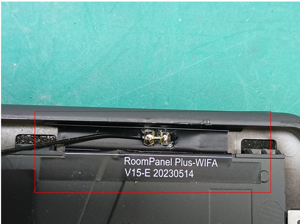
BT/Wi-Fi ANT
