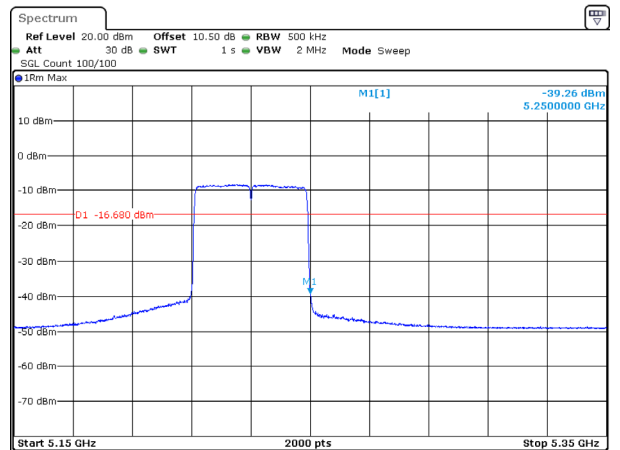
802.11ax40_5230MHz_RU_Full
