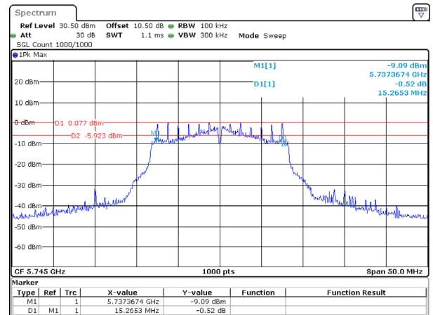
802.11a_5745MHz
