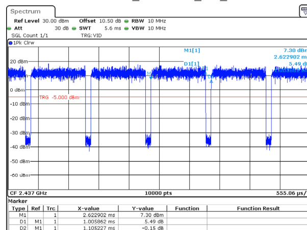
802.11ax20_2437MHz_RU_Full
