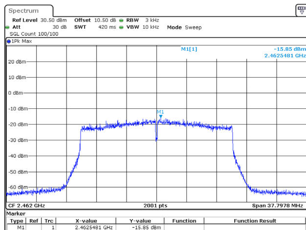
802.11ax20_2462MHz_RU_Full
