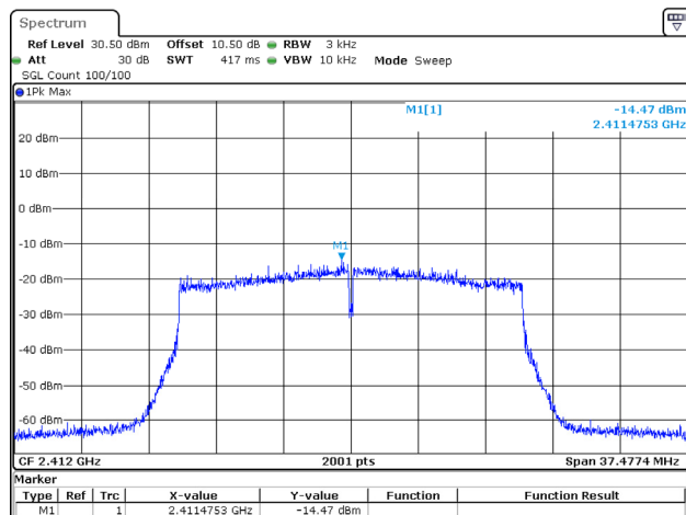
802.11ax20_2412MHz_RU_Full
