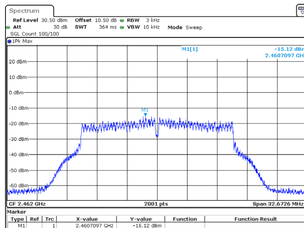
802.11g_2462MHz
